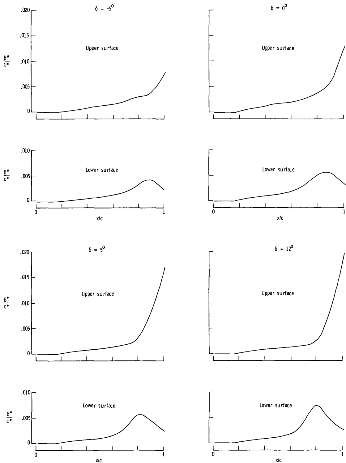
Figure 8.- Chordwise boundary-layer displacement thickness distributions along center line \left(\frac{y}{b/2} = 0.60\right) of midspan control surface. M_\infty = 0.80 ; \alpha = 1.10^\circ ; q_\infty = 6.31 \text{ kPa (131.8 lb/ft}^2\text{)} .
