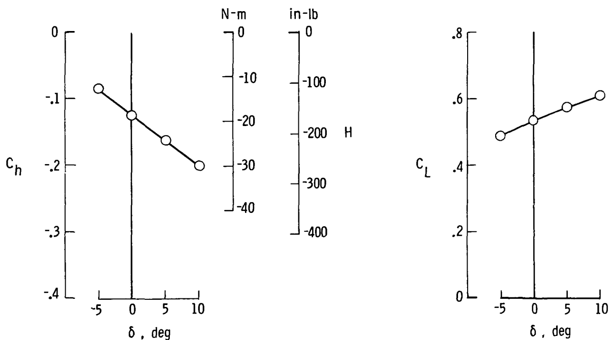
Figure 6.- Hinge-moment and lift coefficients for inboard control surface. M_\infty = 0.60 ; \alpha = 1.63^\circ ; q_\infty = 19.70 kPa (411.3 lb/ft 2 ).
