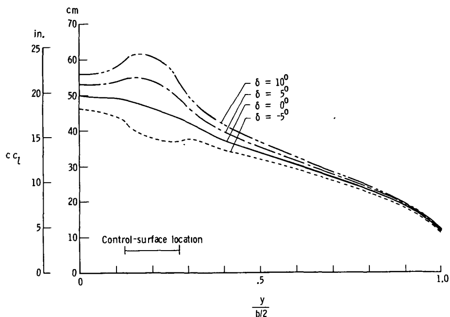
Figure 5.- Spanwise load distribution for inboard control surface deflected. M_\infty = 0.60 ; \alpha = 1.63^\circ ; q_\infty = 19.70 kPa (411.3 lb/ft 2 ).
