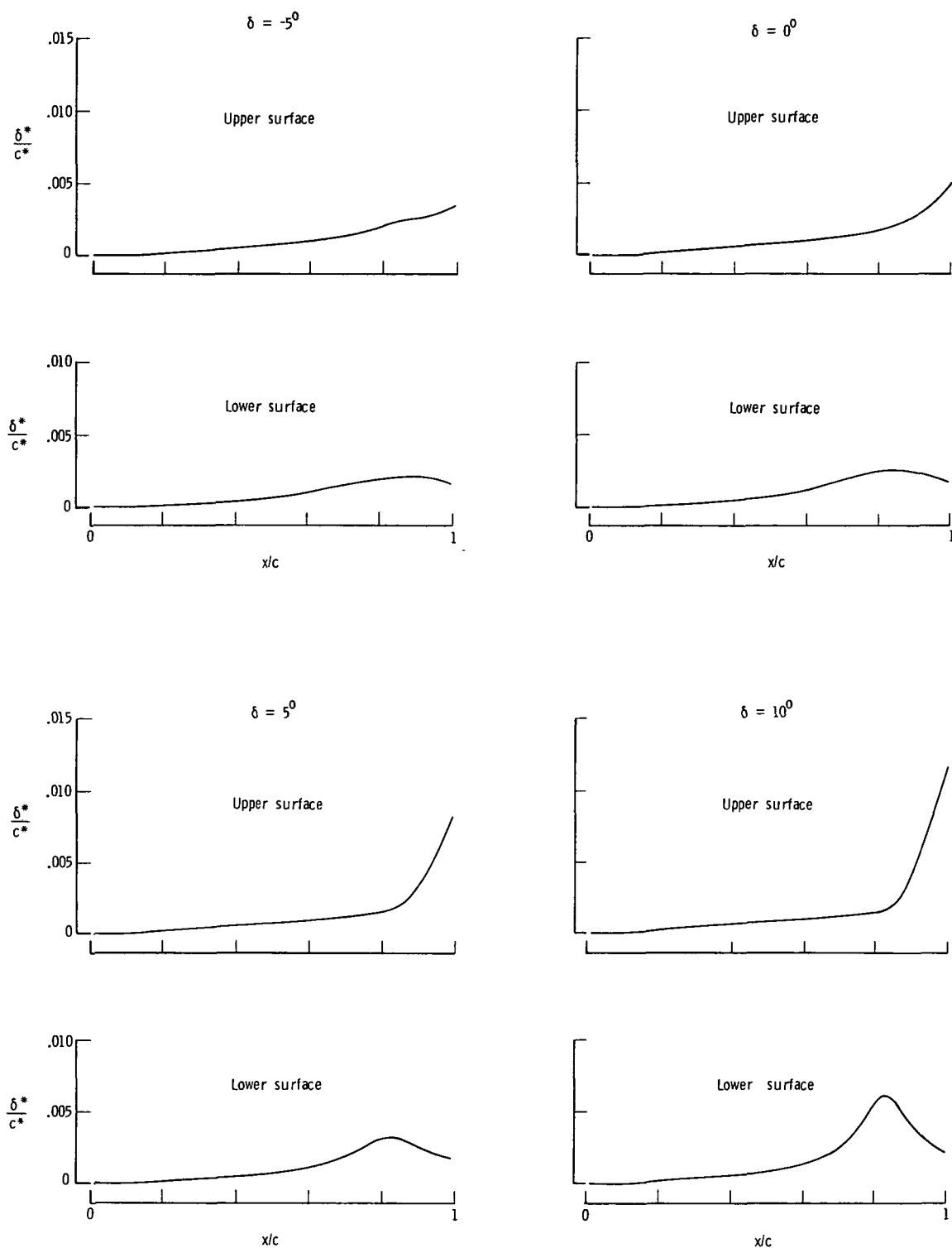
Figure 4.- Chordwise boundary-layer displacement thickness distributions along center line ( \frac{y}{b/2} = 0.20 ) of inboard control surface. M_\infty = 0.60 ; \alpha = 1.63^\circ ; q_\infty = 19.70 kPa (411.3 lb/ft 2 ).
