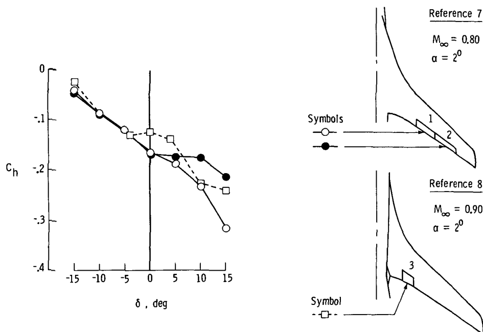
Figure 11.- Hinge-moment coefficient as a function of control-surface deflection angle for references 7 and 8.
