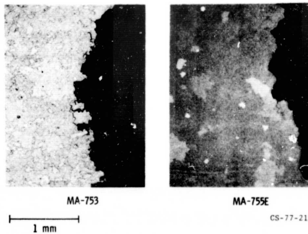
Figure 4. - Shear failures of tensile shear specimens along grain boundaries, transverse views.
