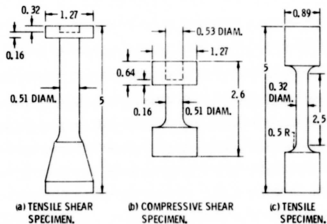
Figure 2. - Test specimens used in program; all dimensions in cm.
