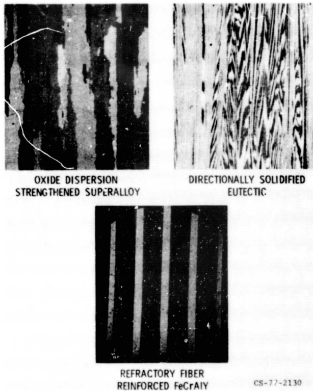
Figure 1. - Competitive materials for advanced turbine blades with elongated microstructures for improved creep strength.
