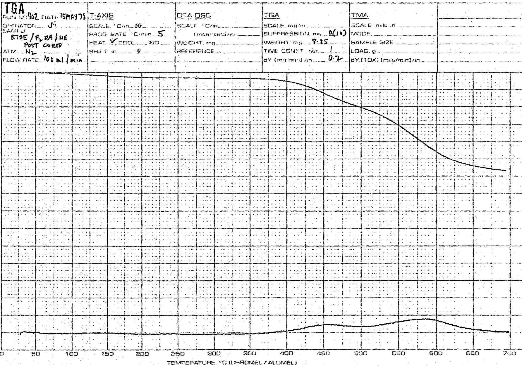
Figure 8: TGA Scan of Post Cured BTDE/HFD/NE Resin (in Nitrogen)
