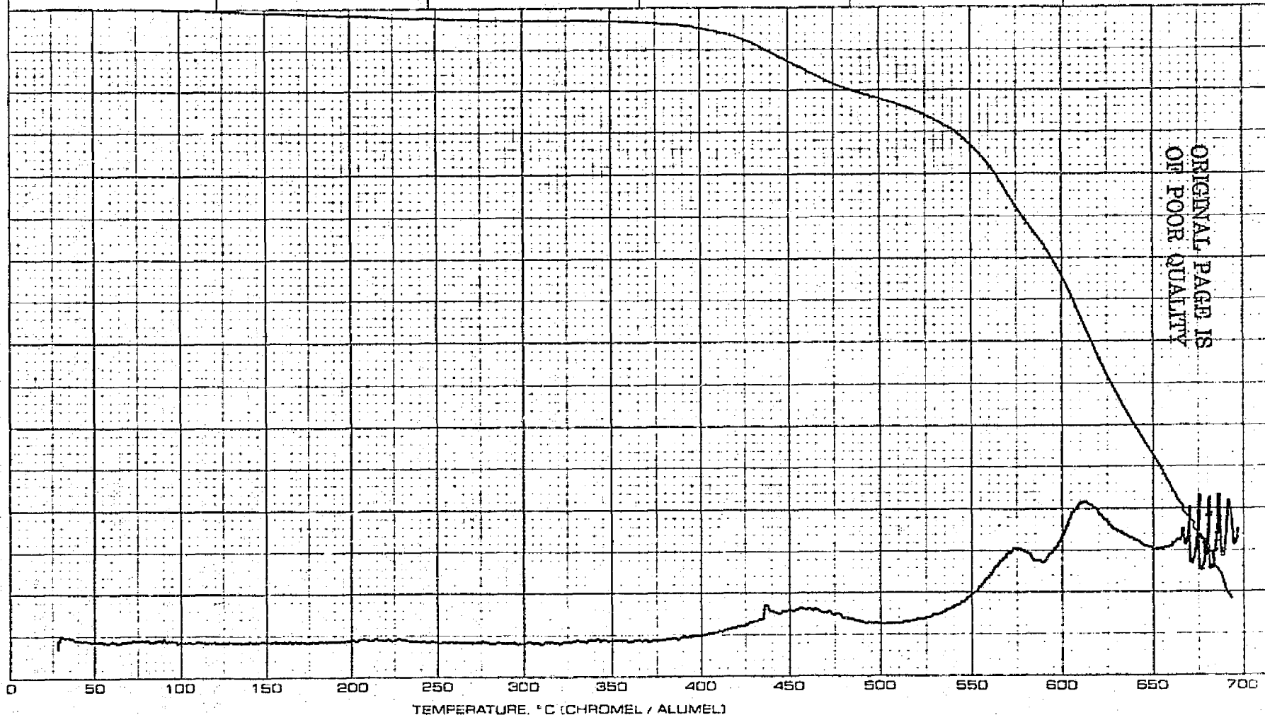
Figure 9: TGA Scan of Post Cured BTDE/HFD/NE Resin (in Air)
