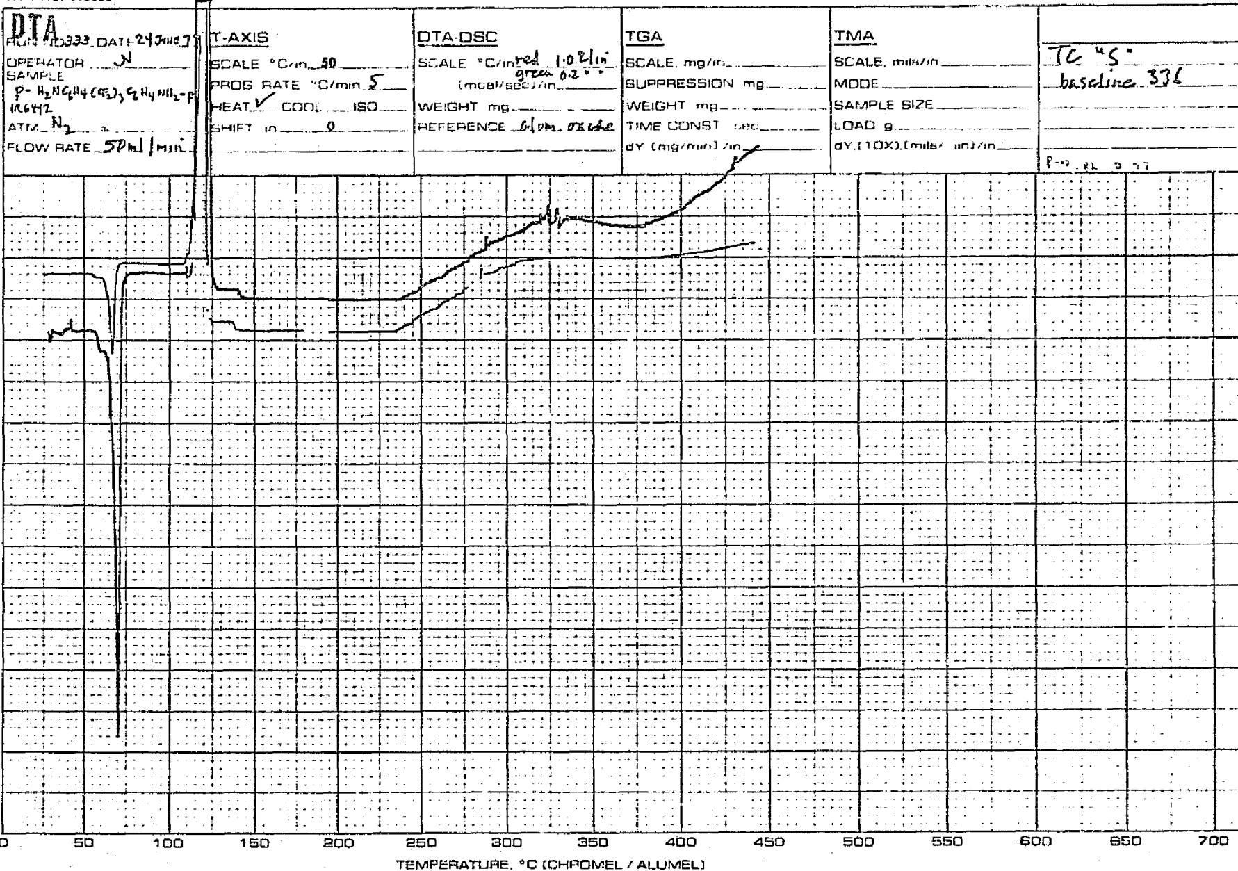
Figure 1: DTA Scan of 1,3-Bis(4-aminophenyl)hexafluoropropane
