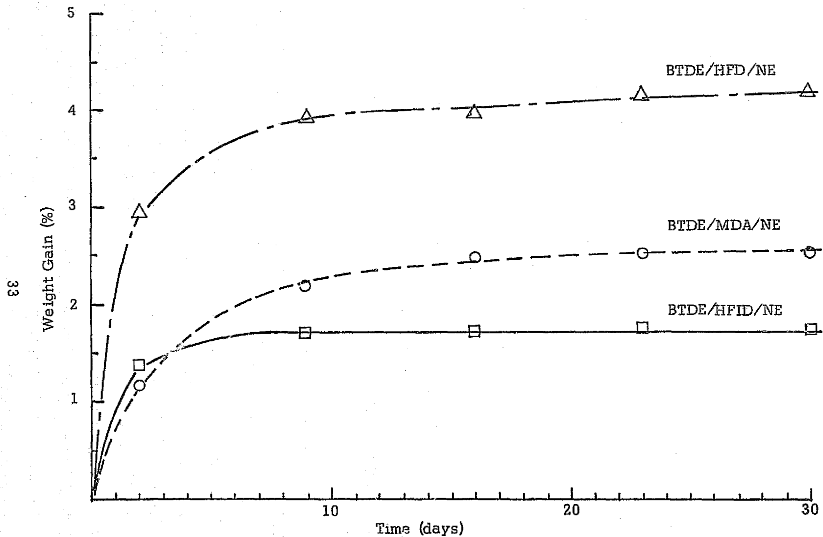
Figure 3: Weight Gain as a Function of Time of Fully Cured Resins on Exposure to 95% Humidity.
