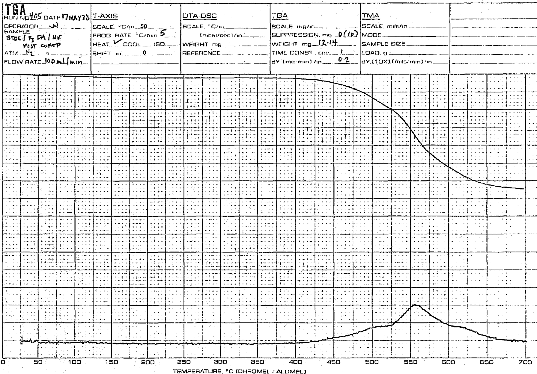
Figure 12: TGA Scan of Post Cured BTDE/HFID/NE Resin (in Nitrogen)
