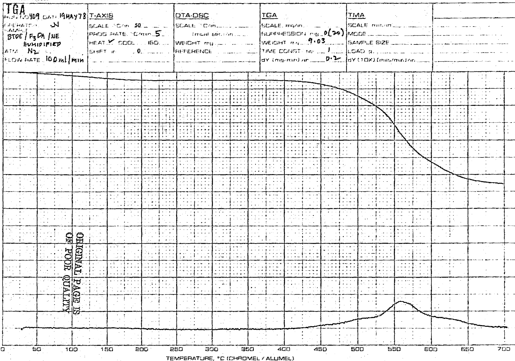
Figure 14: TGA Scan of Post Cured-Humidity Exposed BTDE/HFID/NE Resin (in Nitrogen)
