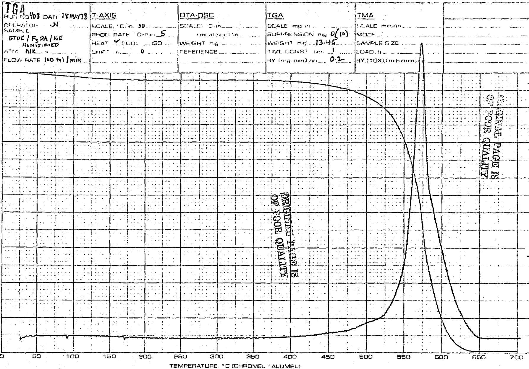
Figure 15: TGA Scan of Post Cured-Humidity Exposed BTDE/HFID/NE Resin (in Air)
