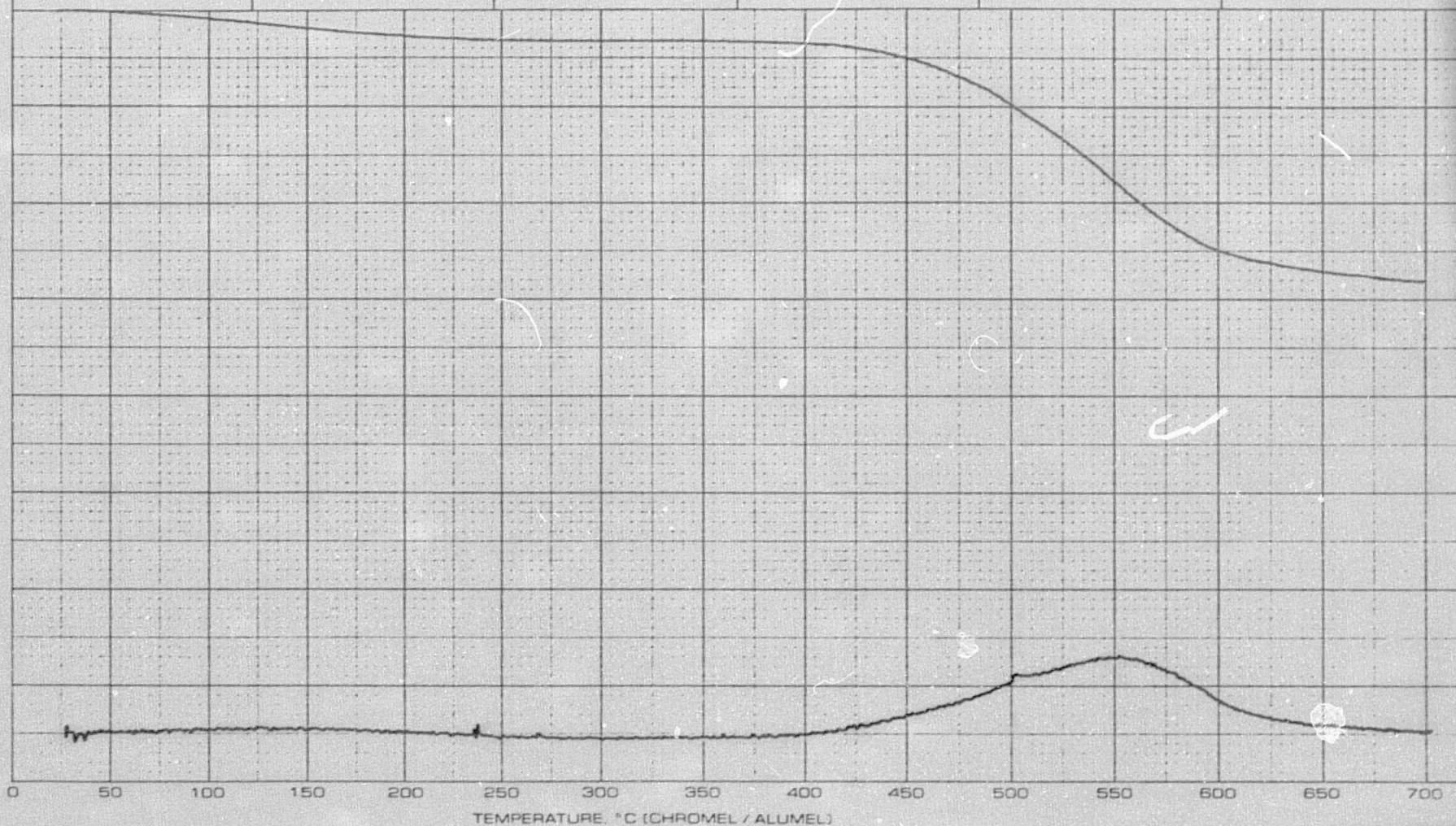
Figure 6: TGA Scan of Post Cured-Humidity Exposed BTDE/MDA/NE Resin (in Nitrogen)
