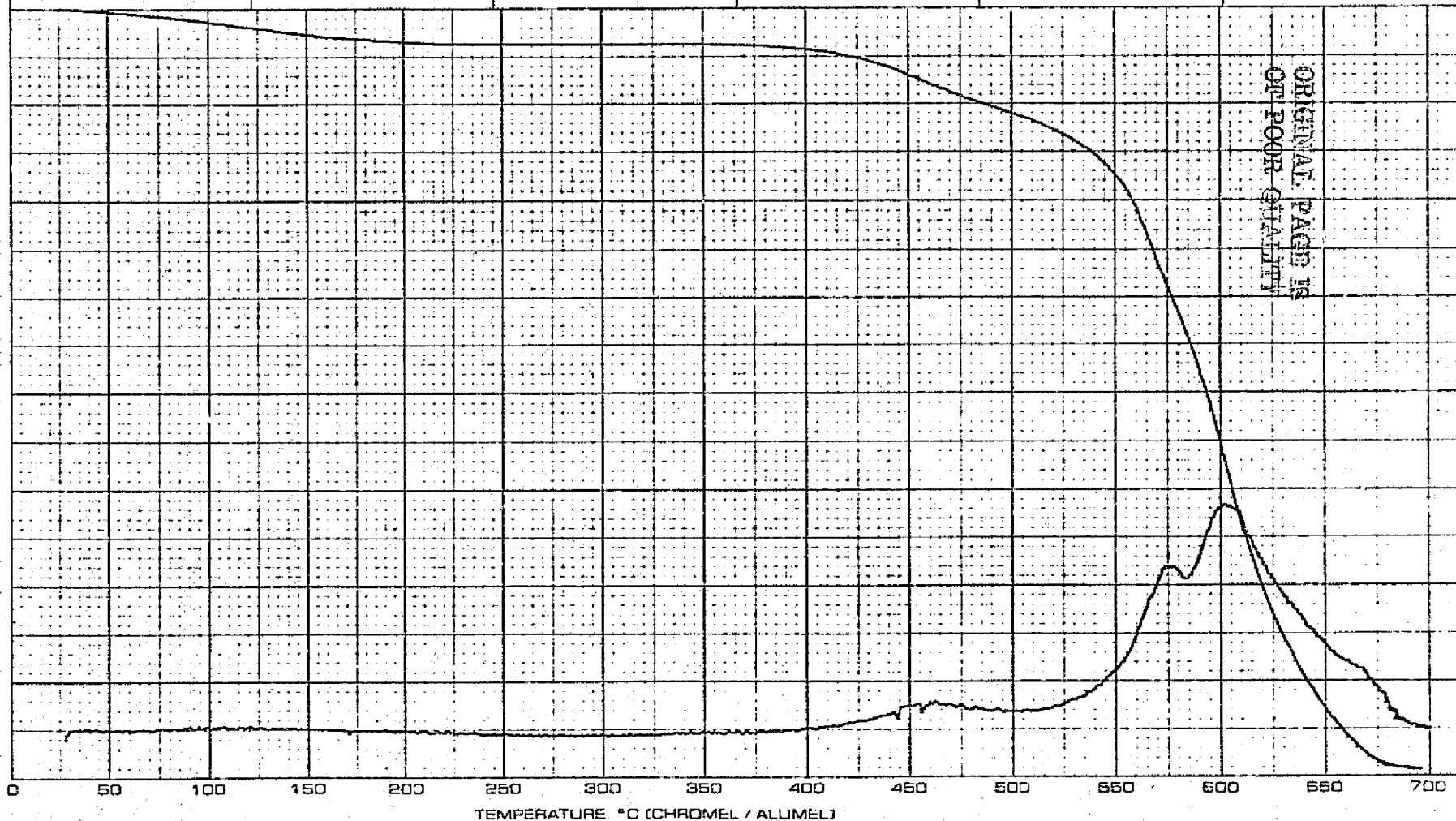
Figure 11: TGA Scan of Post Cured-Humidity Exposed BTDE/HFD/NE Resin (in Air)
