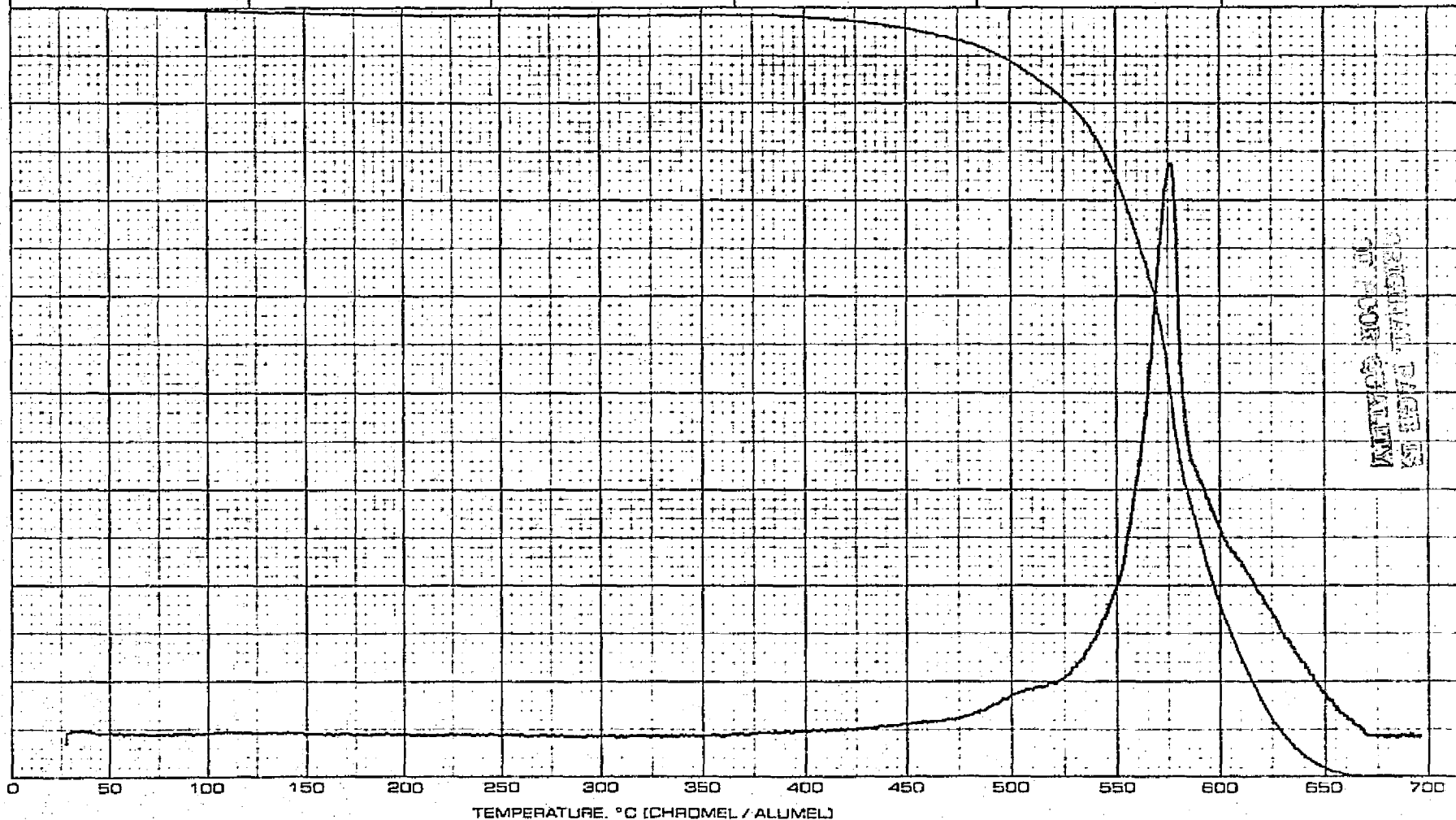
Figure 10: TGA of Post-Cured BTDE (HTD) (Air) Resin (in N 2 )
