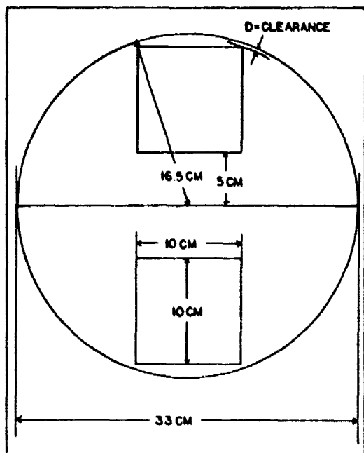
Fig. 4. Format projection on surface of parabolic mirror.
