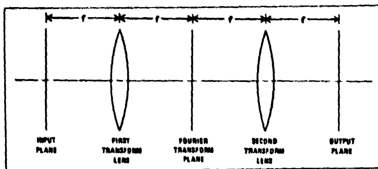
Fig. 1. Basic optical processor.
