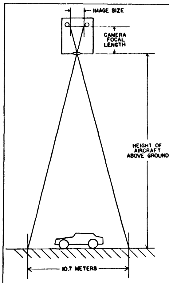
Fig. 5. Scaling of aerial photograph.
