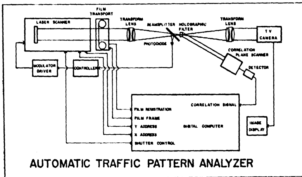
Fig. 1. Basic optical processor.
