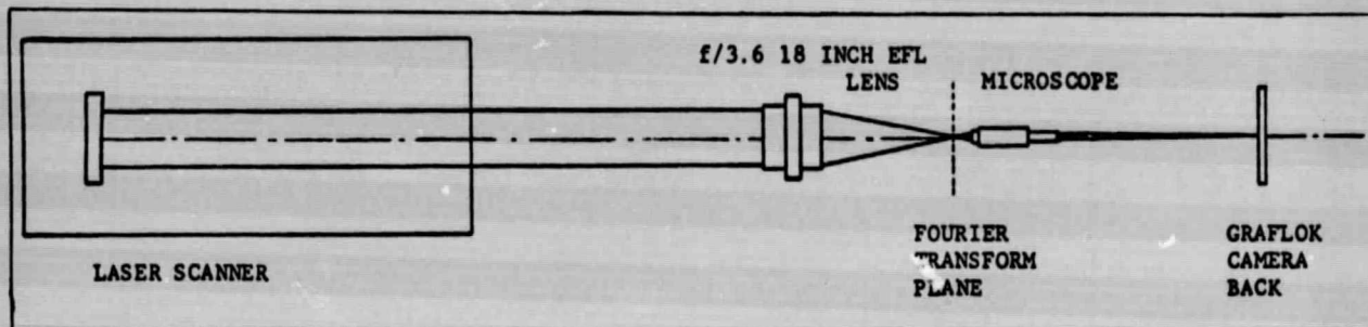
Fig. 6. (Above) Fourier transform spatial invariance test.
