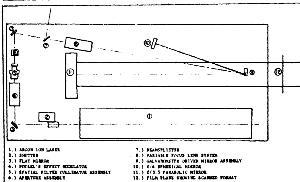
Fig. 3. Laser scanner optical system.
