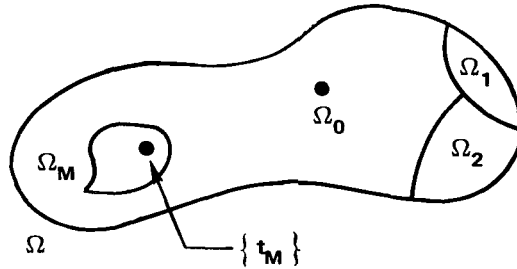
Figure 2. Sample space for the random-point process.
