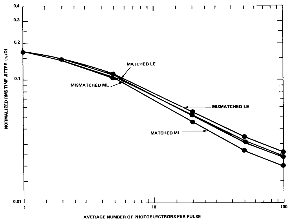
Figure 15. Performance of several matched-filter type receivers to bell-shaped optical pulses, given at least one photoelectron observation. Mismatched filters represent filter impulse responses equal to the laser pulse shape rather than to the logarithm of the pulse shape. LE represents timing to the 50-percent point on the leading edge of the filter output waveform; the ML receivers time to the peak of the waveform.
