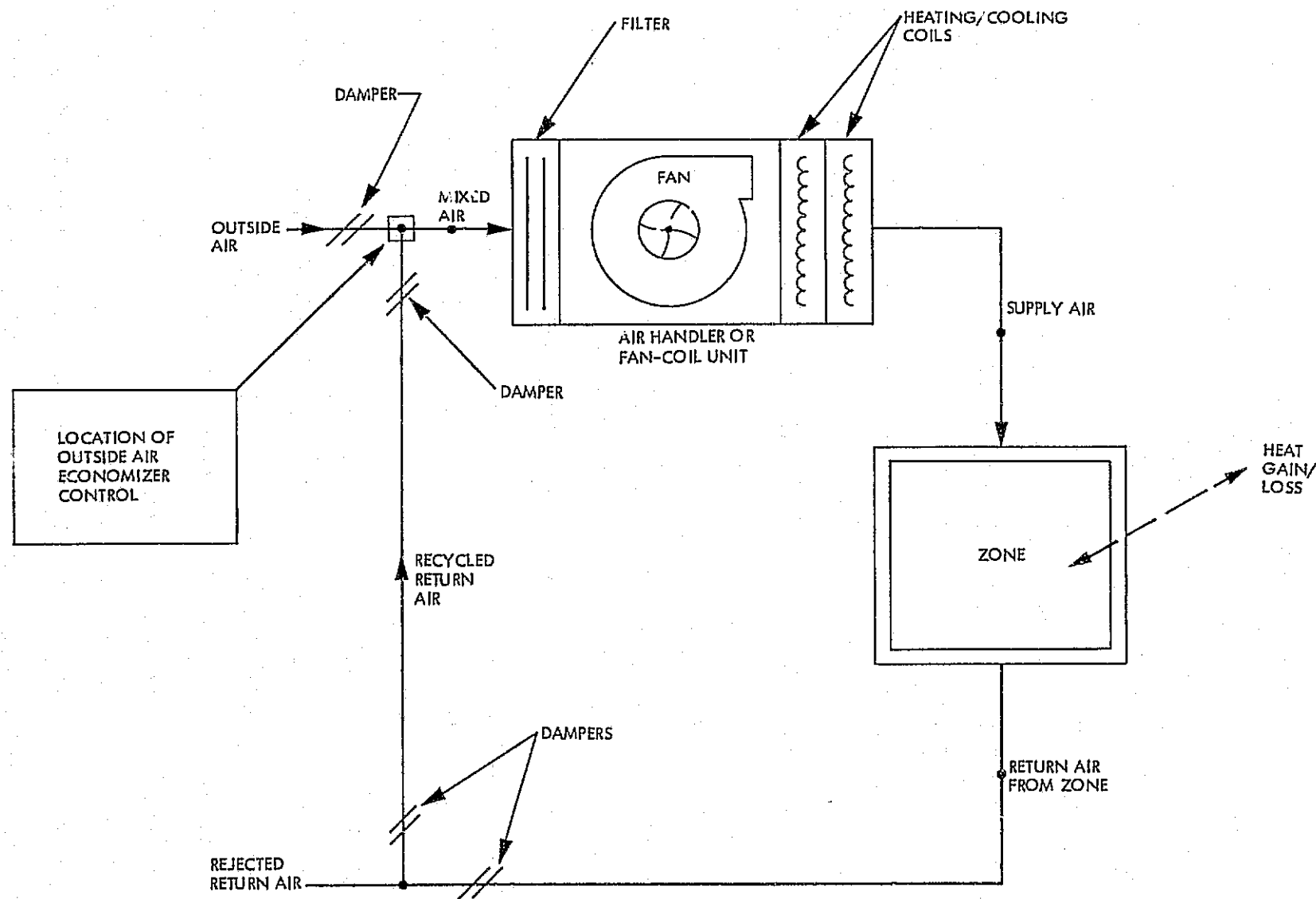
Figure 1-2. General schematic of an air conditioning system
