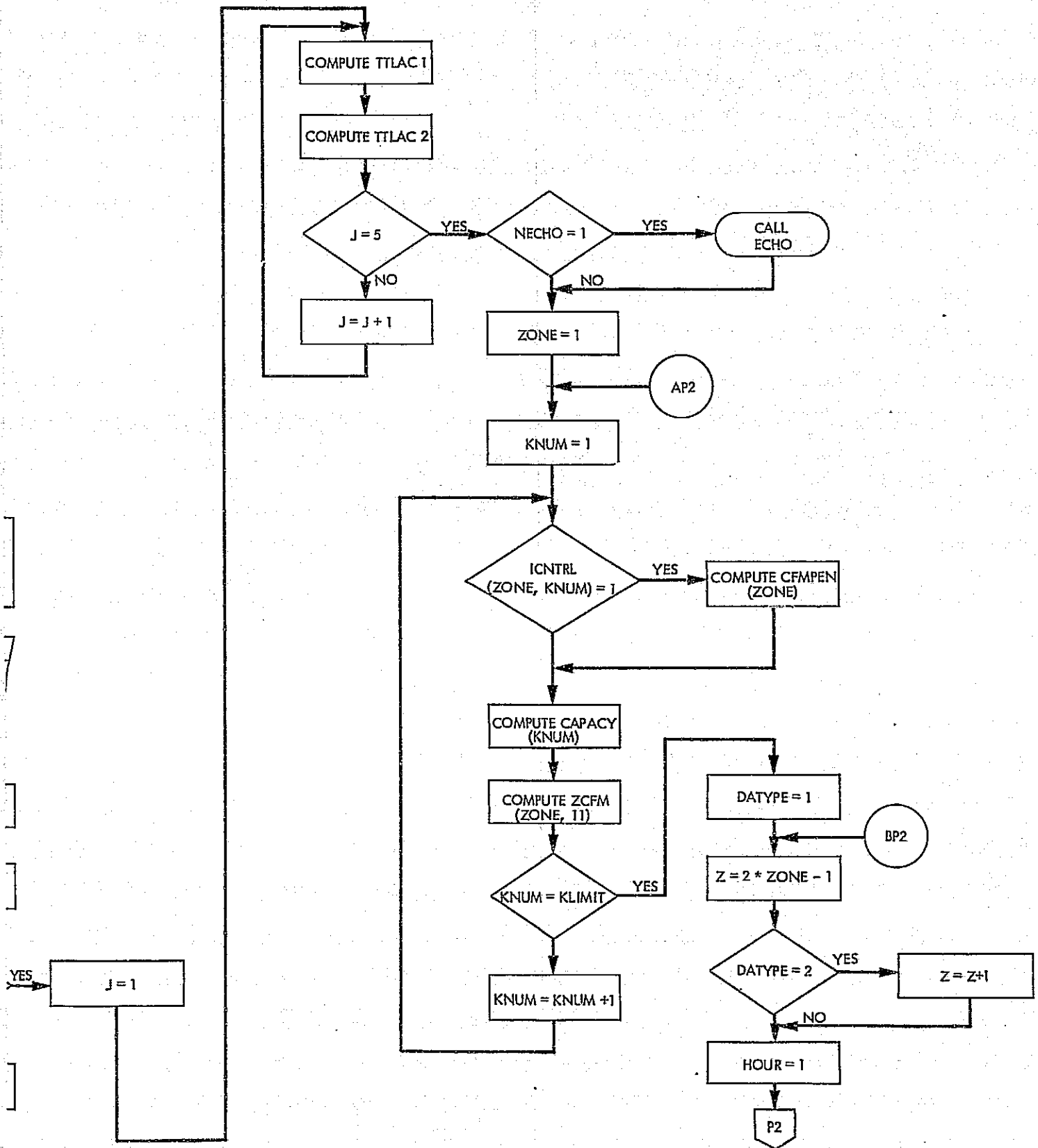
Figure 5-1. Main program flow chart
