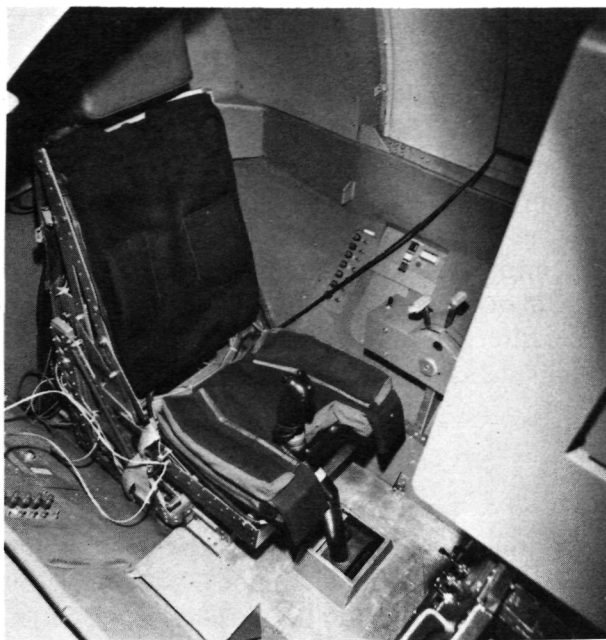
Figure 6.— G-seat cockpit configuration.
