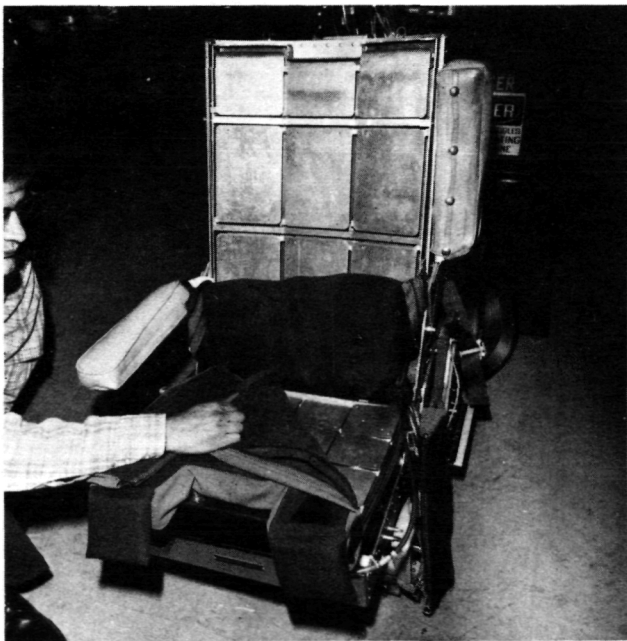
Figure 2.— G-seat photograph.
