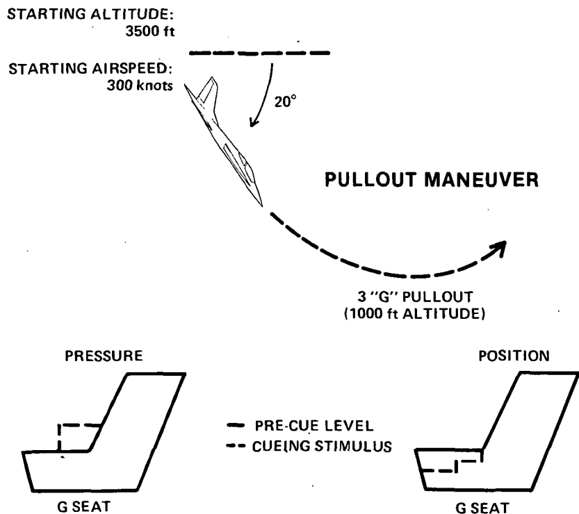
Figure 8.— Pressure vs position cueing scheme for -Z accelerations.
