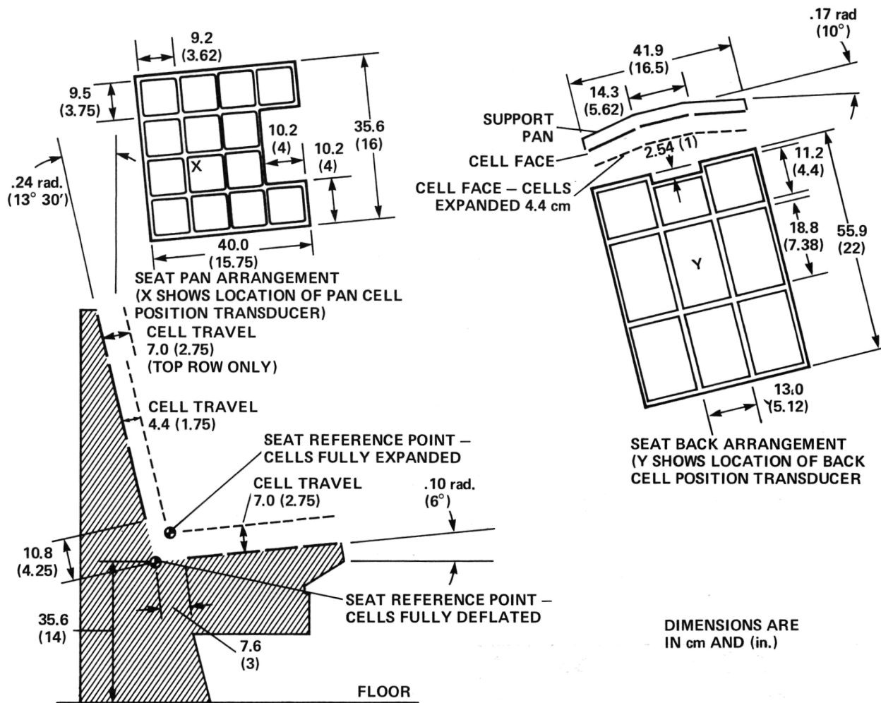
Figure 4.— G-seat dimensions.
