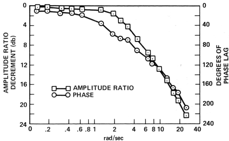
Figure 5.— G-seat frequency response characteristics.
