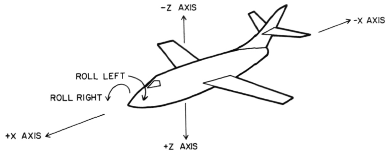
Figure 1.— Sign conventions for vertical, longitudinal, and roll accelerations.
