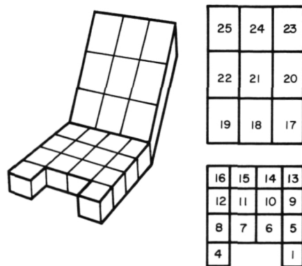
Figure 3.— G-seat cell diagram.
