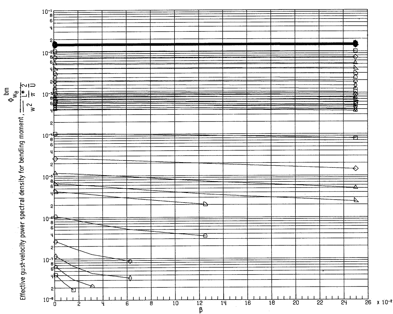
(b) Effective power spectral density plotted against wing-span ratio.
