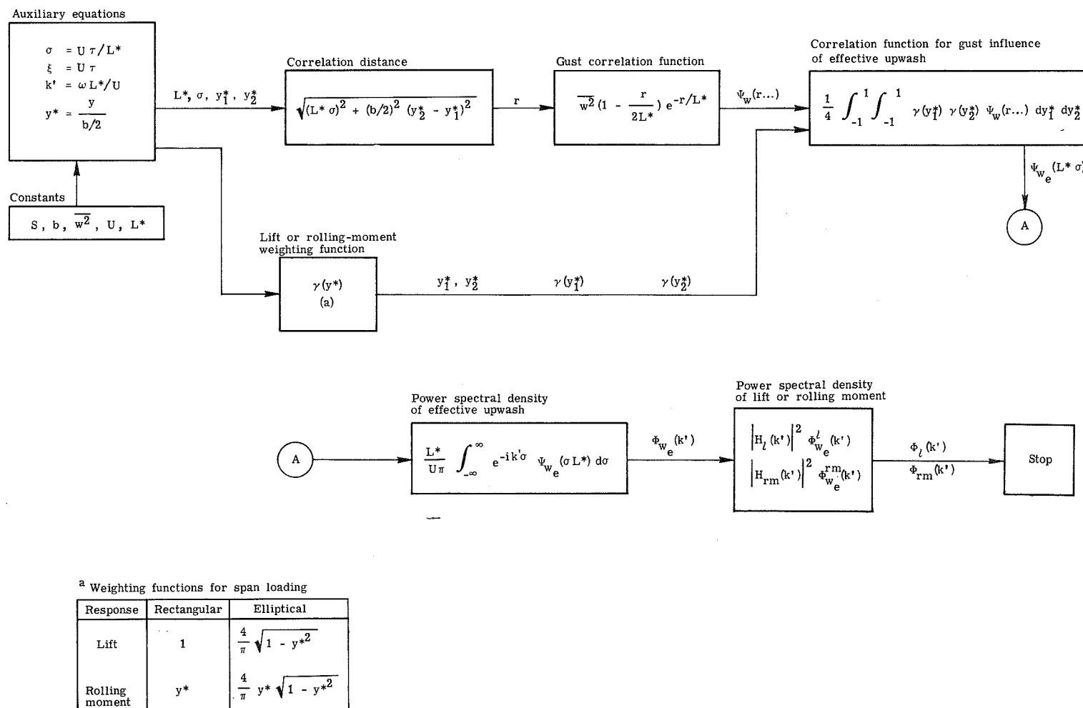
(a) Lift and rolling moment.
