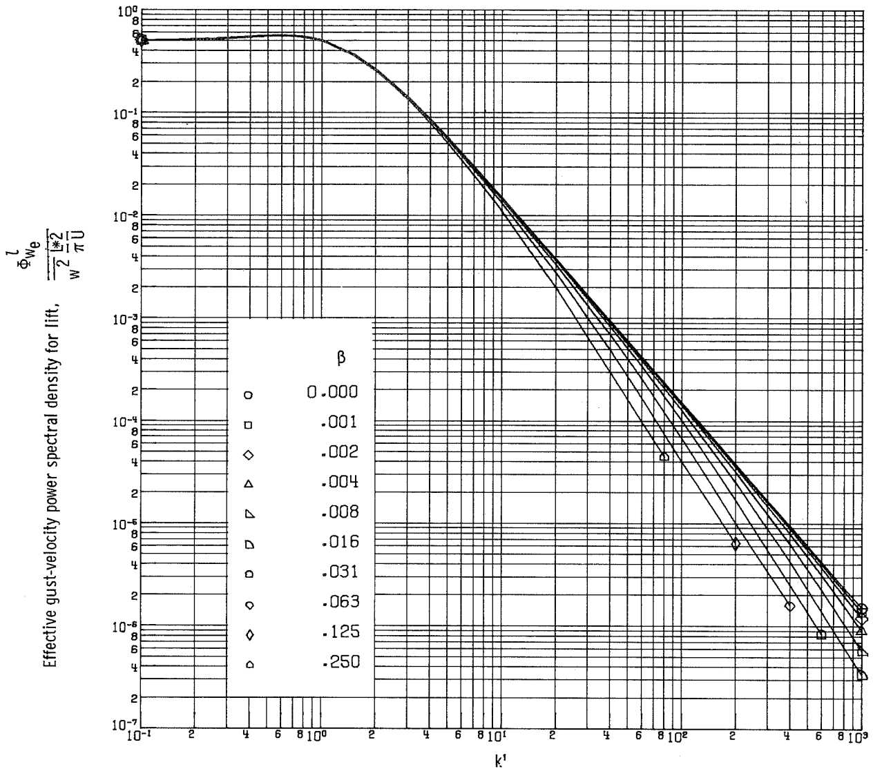
(a) Effective power spectral density plotted against nondimensional frequency for various span ratios.
