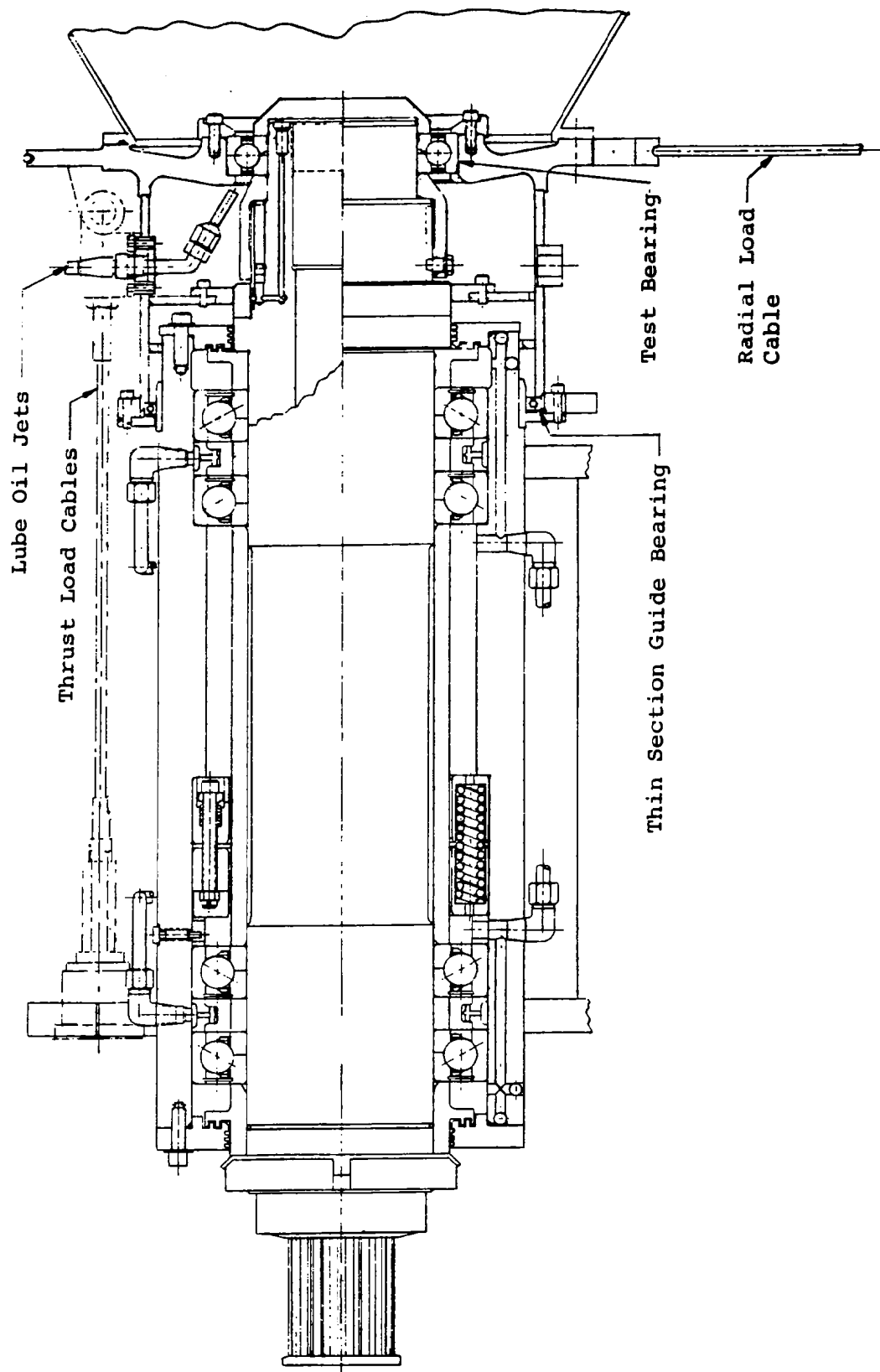
FIG. 1b Schematic of Shaft Assembly
