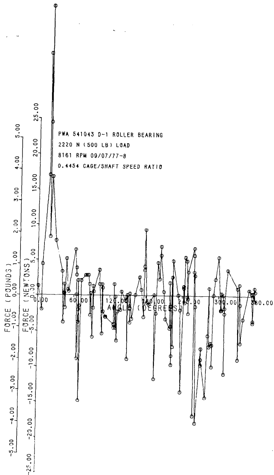
FIG. 3d Roller Contact Forces 0.18 mm Clearance Bearing
