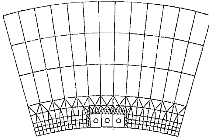
Figure 12 Residual Superelement
