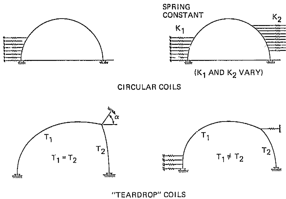
Figure 6 Configuration and Support of Coils (TF1G2D)
