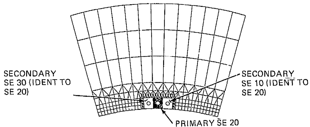
Figure 13 Primary Superelement
