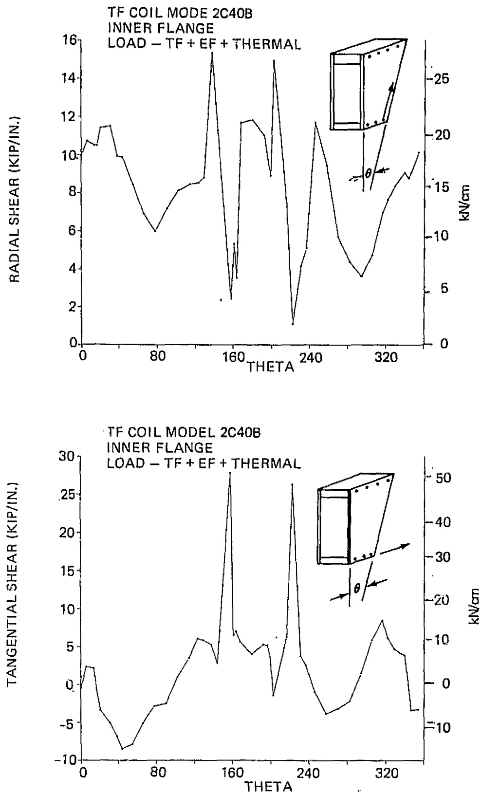
Figure 20 Typical Radial and Tangential Shear
