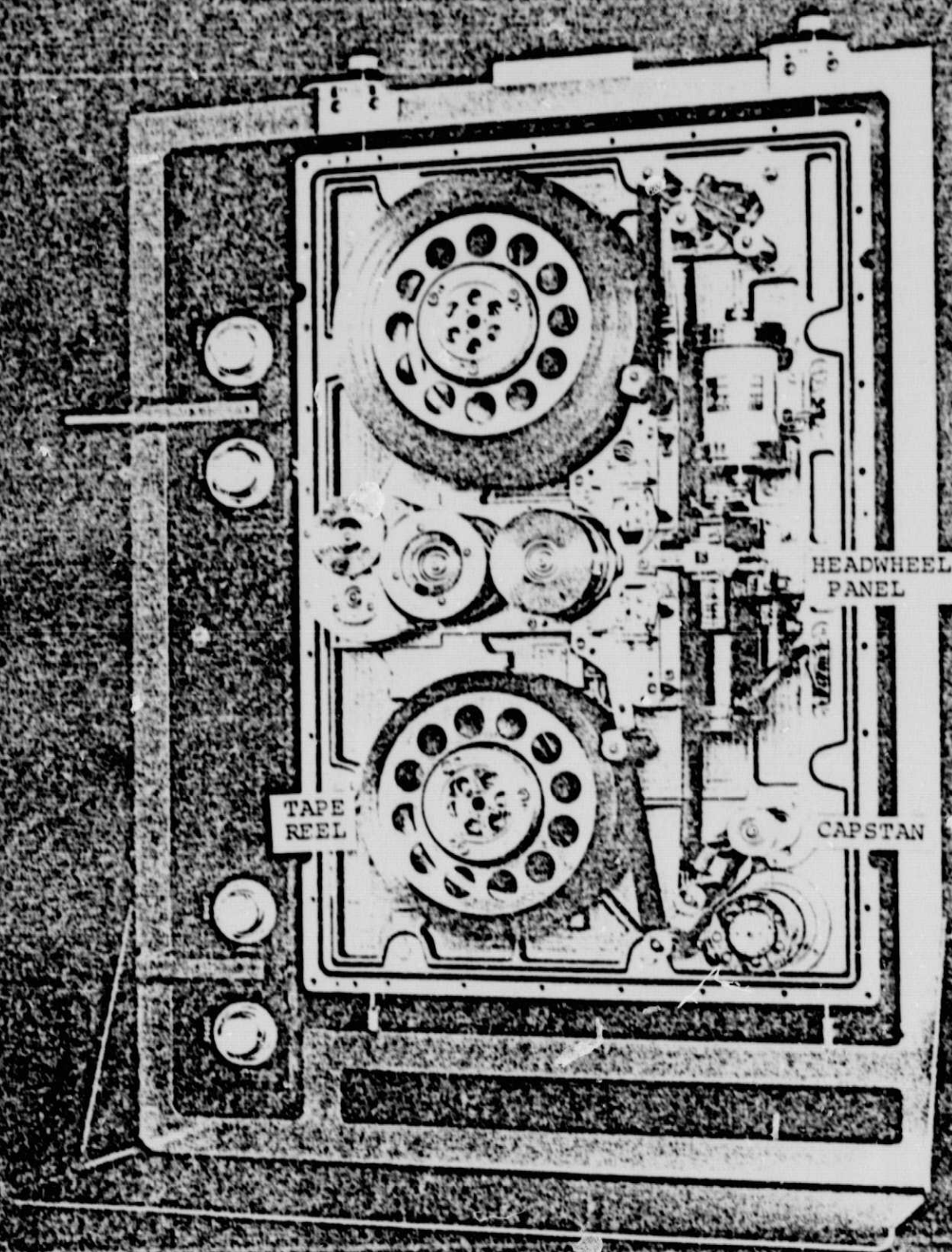
FIG. 1 LANDSAT WBVTR TRANSPORT UNIT
