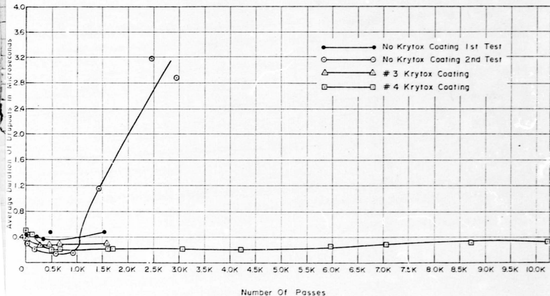
FIGURE 3 AVERAGE DURATION OF DROPOUTS VS. NUMBER OF PASSES TAPE TYPE MTA - 20237
