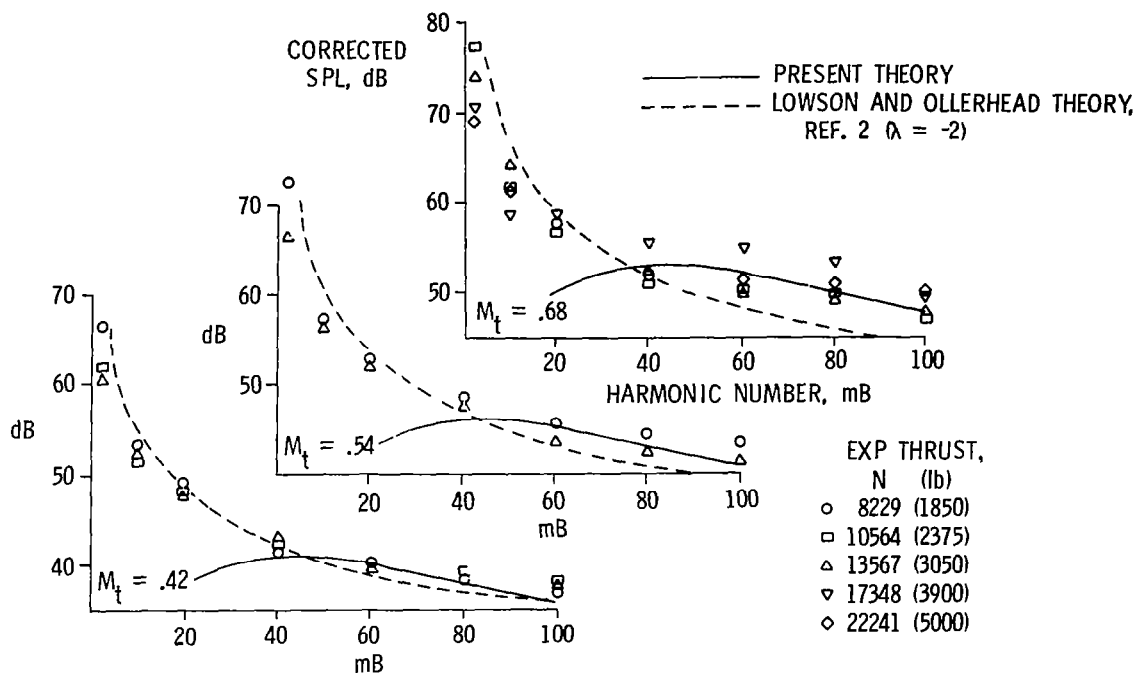
Figure 3.- Rotor discrete tone noise, microphone B ( 11.5^\circ from rotor plane).
