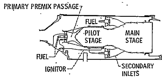
(c) Staged premix combustor.
