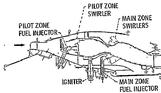
Figure 4. - Pratt and Whitney Vortex combustor for the JT9D-7 engine.
