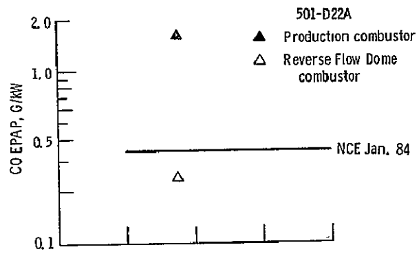
(a) CO emission standards.
