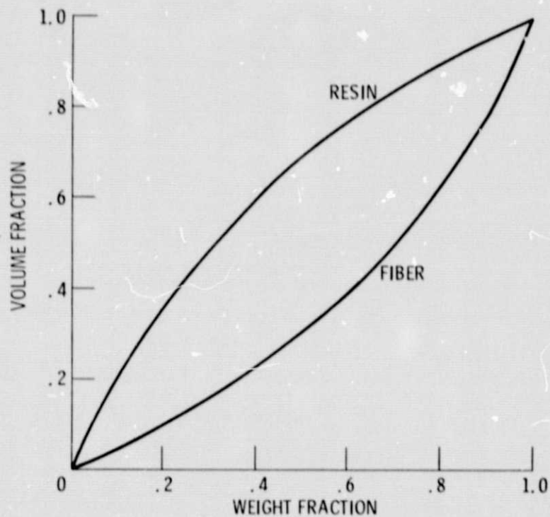
Figure 5. - Volume fraction versus weight fraction glass-resin system (fiber density = 2.60 \text{ g/cm}^3 ( 0.094 \text{ lb/in}^3 ), resin density = 1.19 \text{ g/cm}^3 ( 0.042 \text{ lb/in}^3 )) (ref. 4).
