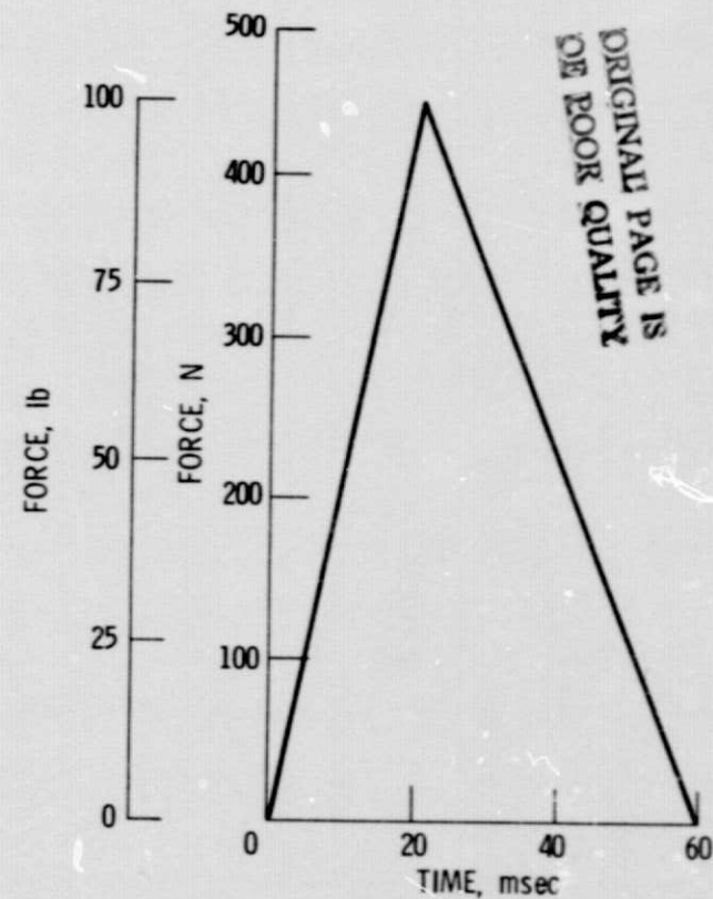
Figure 8. - Impulsive load for determining the relative dynamic response of strip hybrids.
