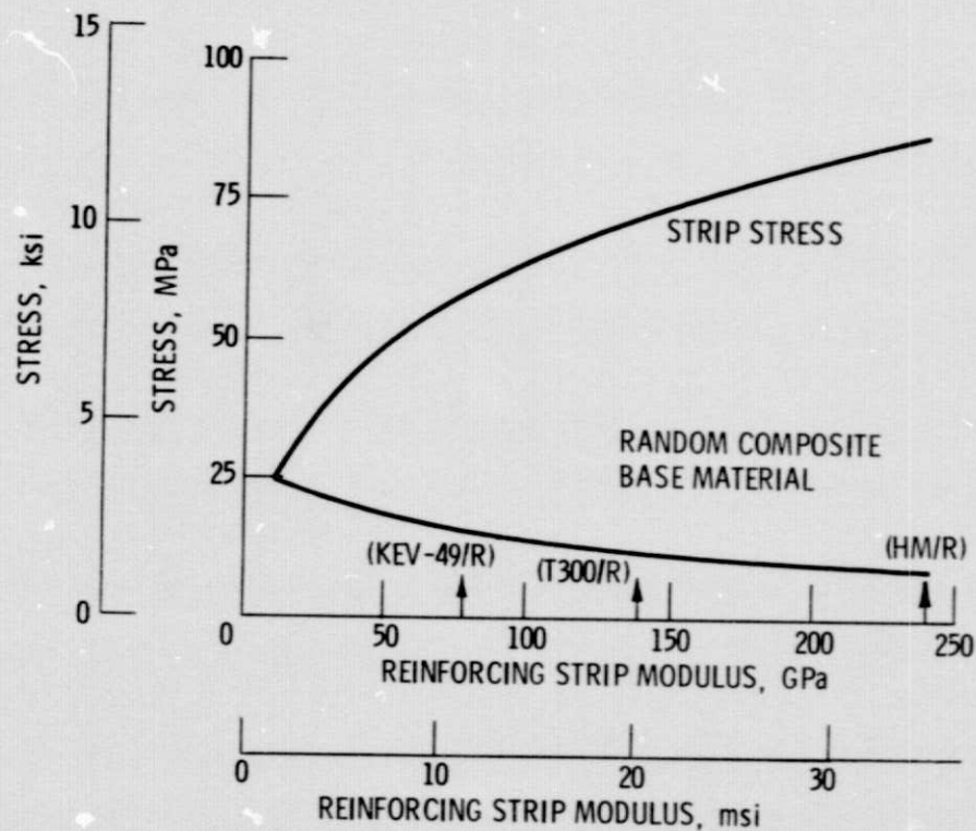
Figure 7. - Maximum stresses in strip hybrid square plates with fixed edges and subjected to concentrated load 44.6 N (10 lb) at the center. E-glass/resin planar random composite reinforced with two-way unidirectional composite strips 20 percent by volume (50.8 by 50.8 by 0.128 cm (2) by 20 by 0.05 in. ).
