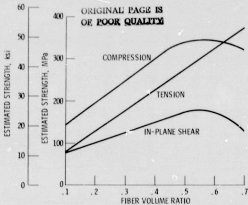
Figure 4. - Estimated fracture stresses (strengths) of planar random E-glass/resin composites.
