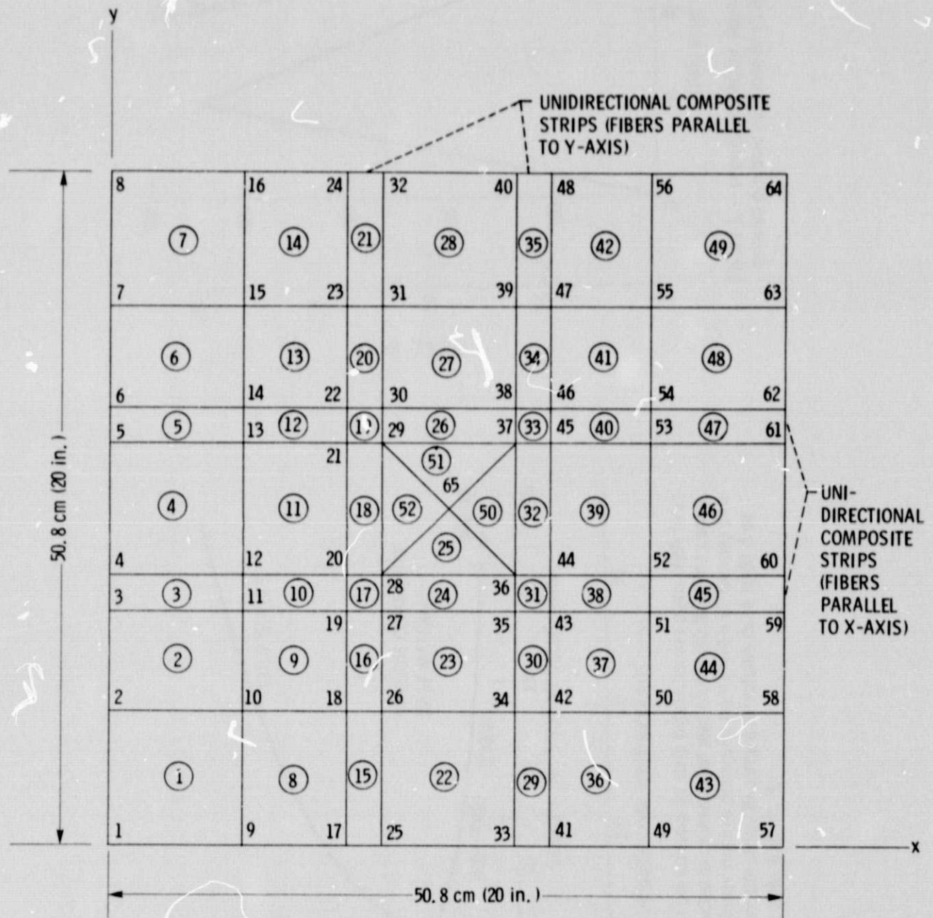
Figure 6. - Finite element representation of a random composite flat panel reinforced with unidirectional composite strips (strip hybrid).
