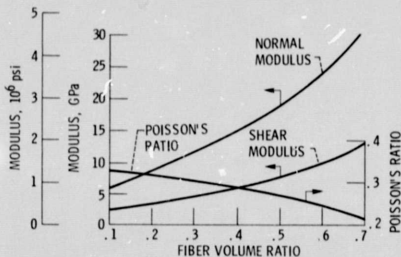
Figure 3. - Elastic properties of planar random E-glass/resin composites predicted using the quasi-isotropic analogy (ref. 1).
