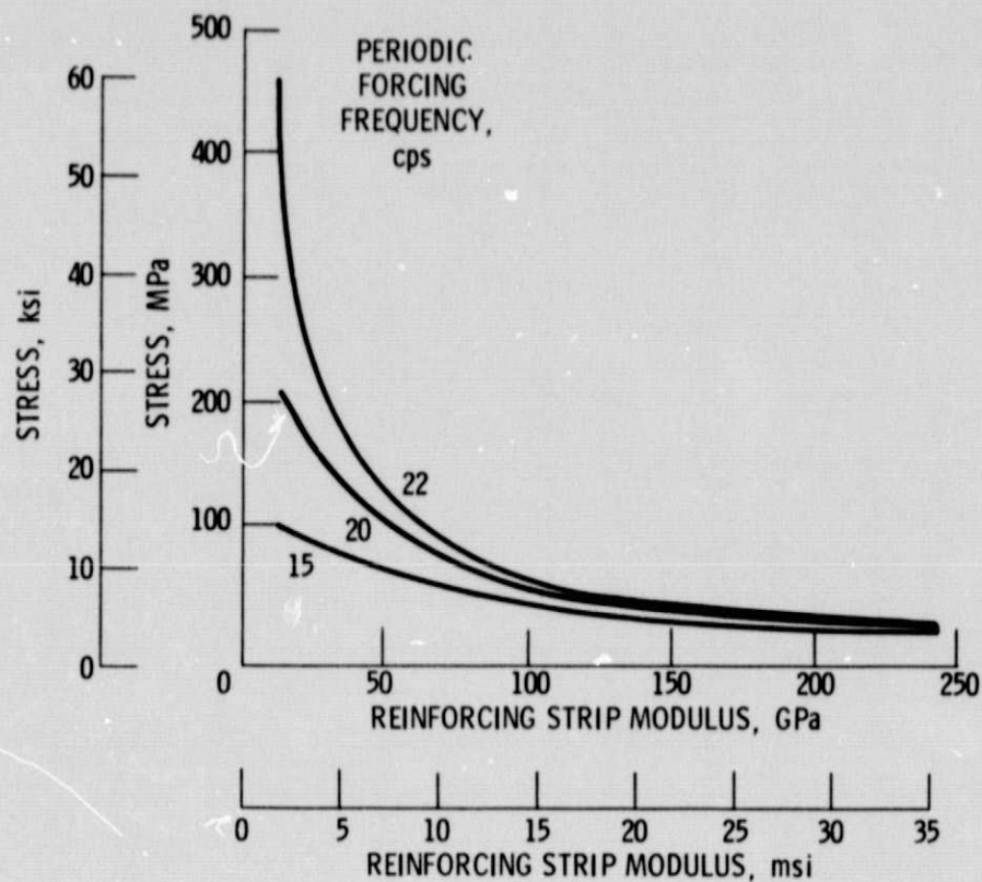
Figure 10. - Base material maximum stresses in strip hybrid square plates with fixed edges and subjected to periodic excitations at center with forcing frequencies below resonance. E-glass/resin planar random composite reinforced with two-way unidirectional composite strips 20 percent by volume (50.8 by 50.8 by 0.127 cm (20 by 20 by 0.05 in.)).
