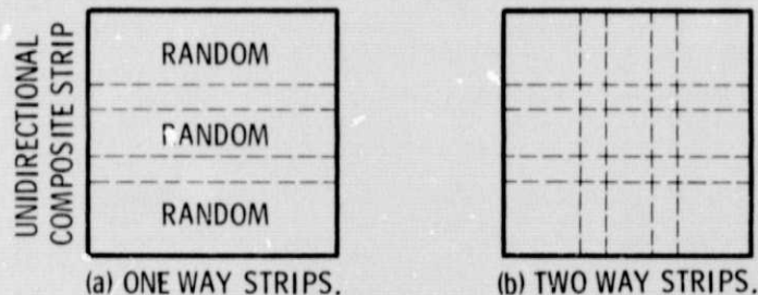
Figure 1. - Schematic of strip hybrids depicting possible location of advanced unidirectional composite strips in a random composite.
