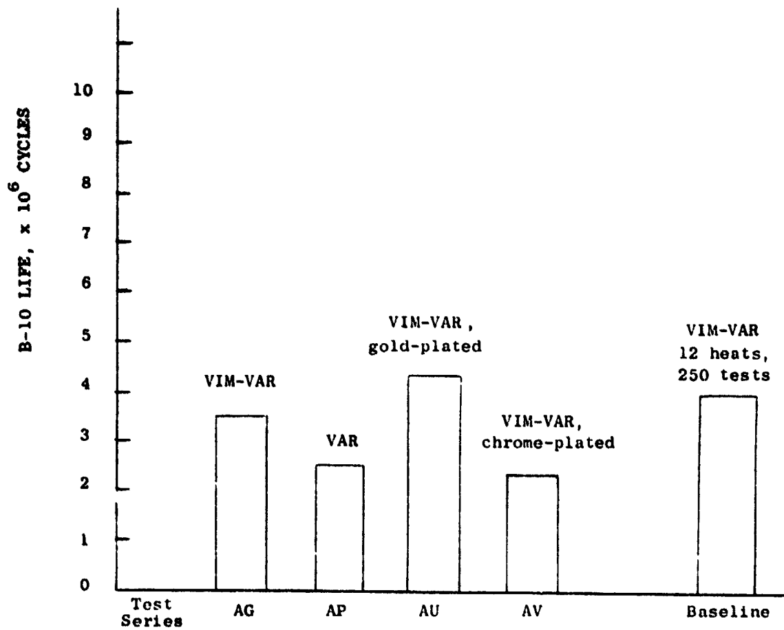
Figure 6. B-10 Fatigue Life of AISI M-50.
