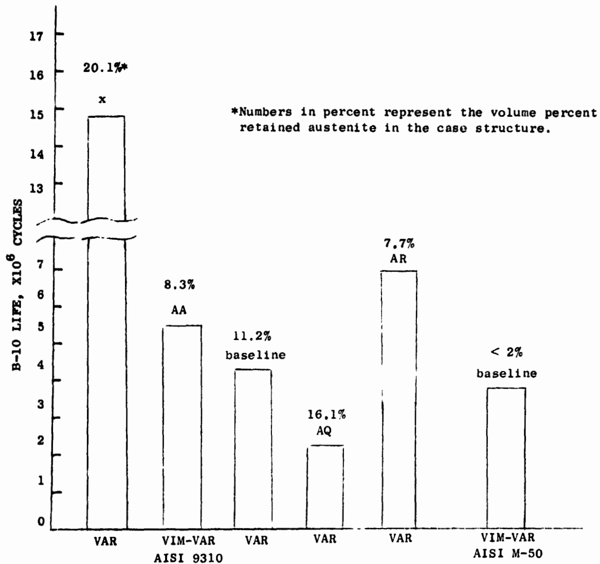
Figure 11. B-10 Fatigue Life Comparision of AISI 9310.
