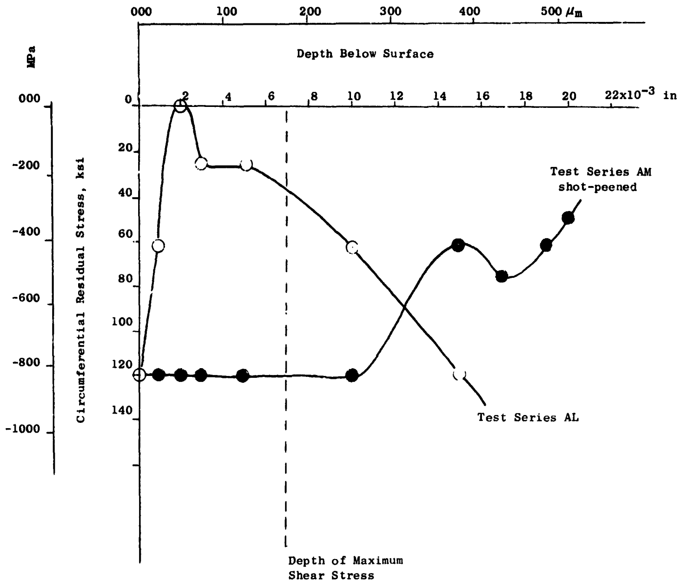
Figure 29. Circumferential Residual Stress as a Function of Depth Below Surface of Vasco X-2 Specimens.
