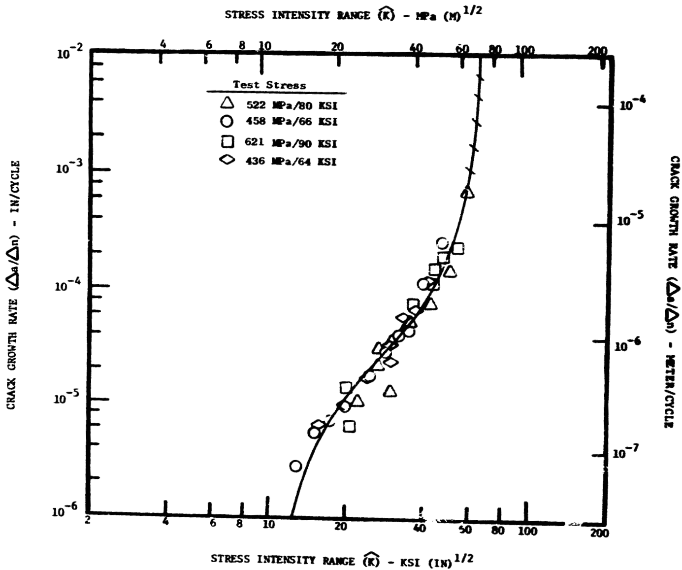
Figure 49. As-HIP René 95 Crack Propagation, 650° C, 0.33 Hz, A_\sigma = 0.95 .
