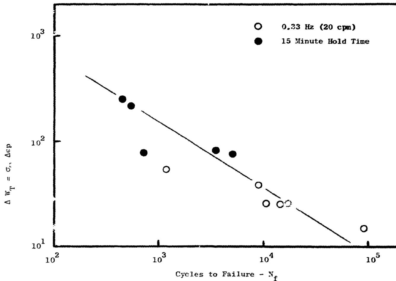
Figure 42. Correlation of R.'95 (H + F) LCF Data (Both 0.33 Hz and 15-Minute Hold Time) with Damage Function \sigma_T \Delta\epsilon_p .
