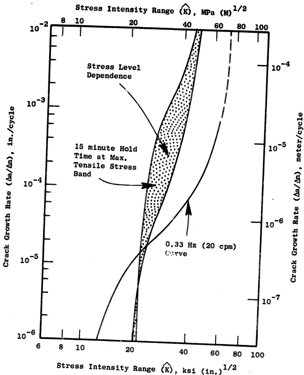
Figure 53. Cyclic Crack Growth Behavior for As-HIP Rene' 95 Under Both Continuous and Hold Time Cycling Condition at 650° C (1200° F).
