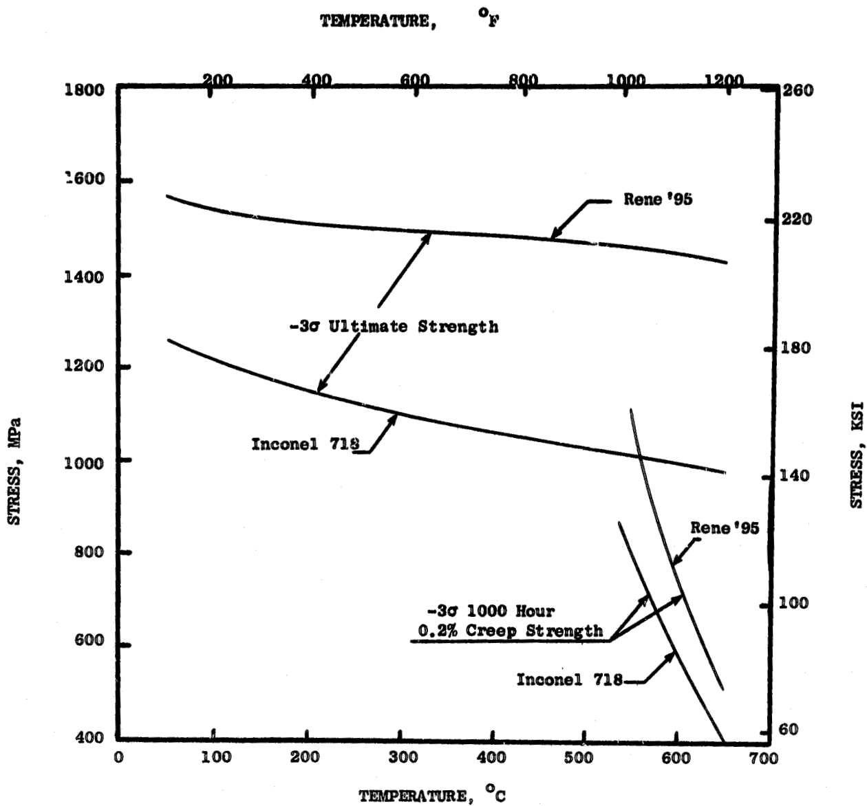
Figure 66. Comparison of Tensile and Creep Behavior of Disk Alloys.
