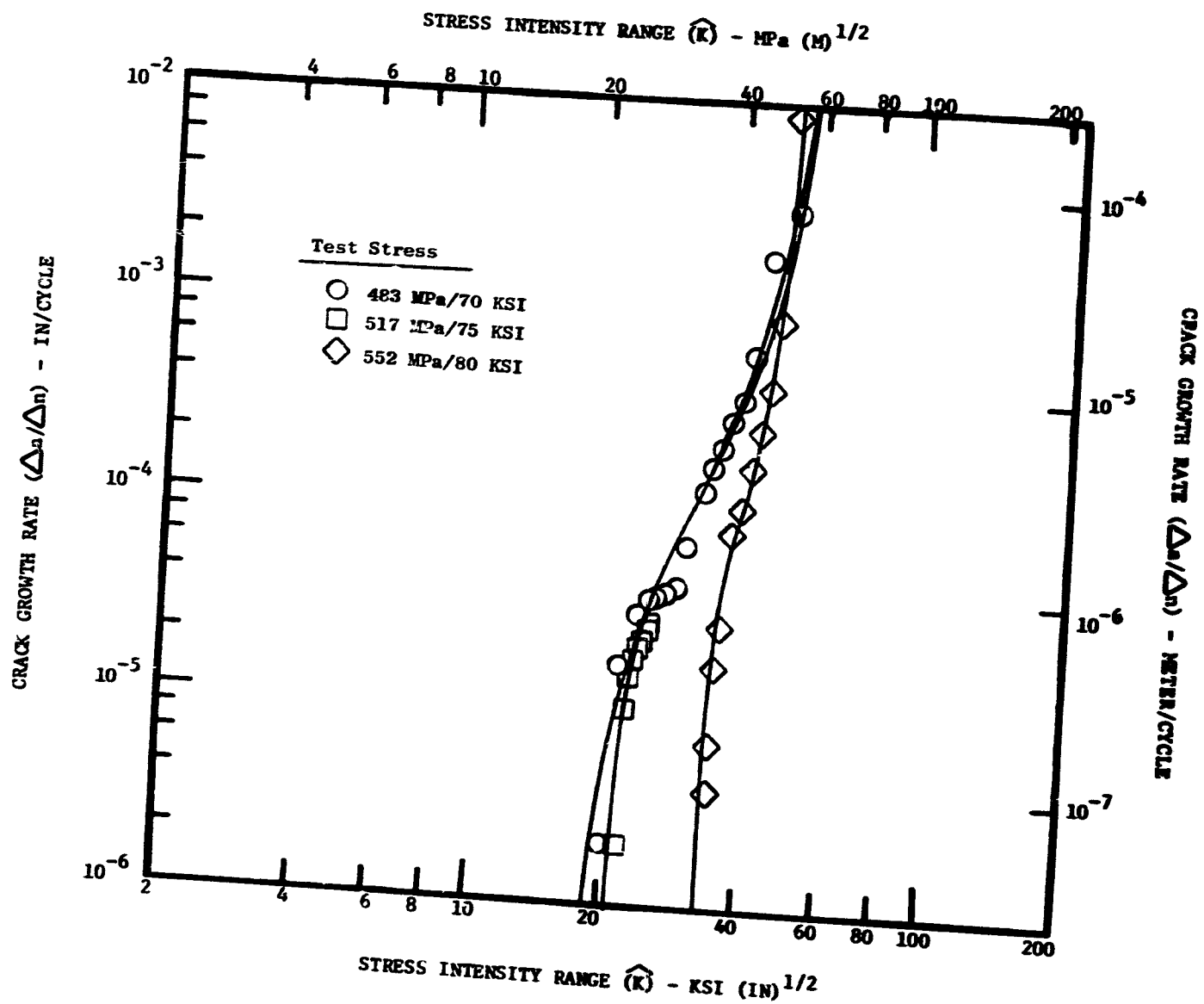
Figure 46. Inconel 718 Crack Propagation, t_h = 15 Minutes, 650° C, A_G = 0.95 .
