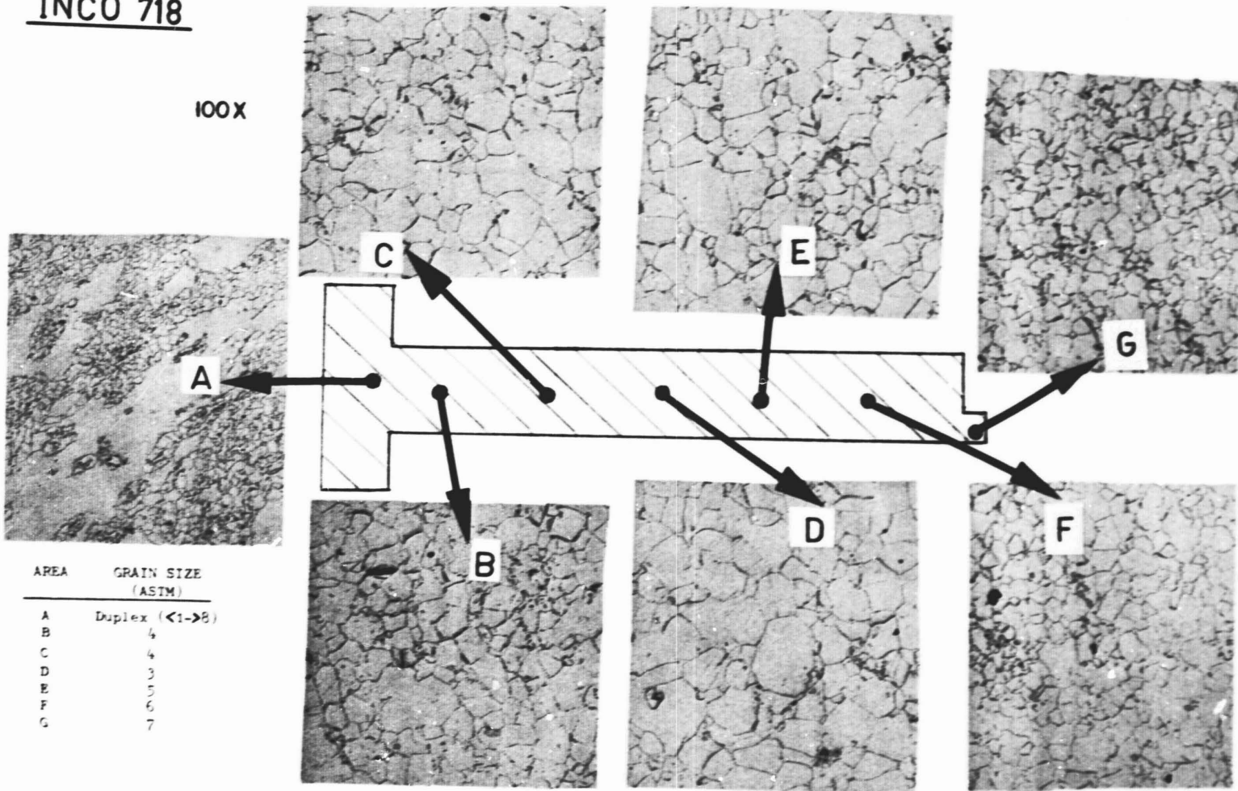
Figure 2. Alloy No. 1 Wrought Inconel 718 - Typical Microstructure Variation Through the Cross Section of the Forging.
