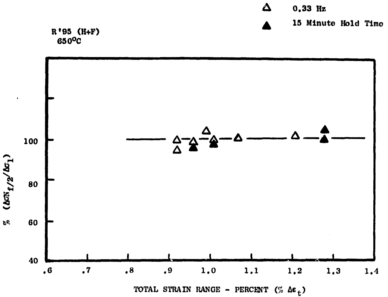
Figure 17. Percent Stress Range Ratio from First Cycle to Mid-Life Cycle as a Function of Total Strain Range.
