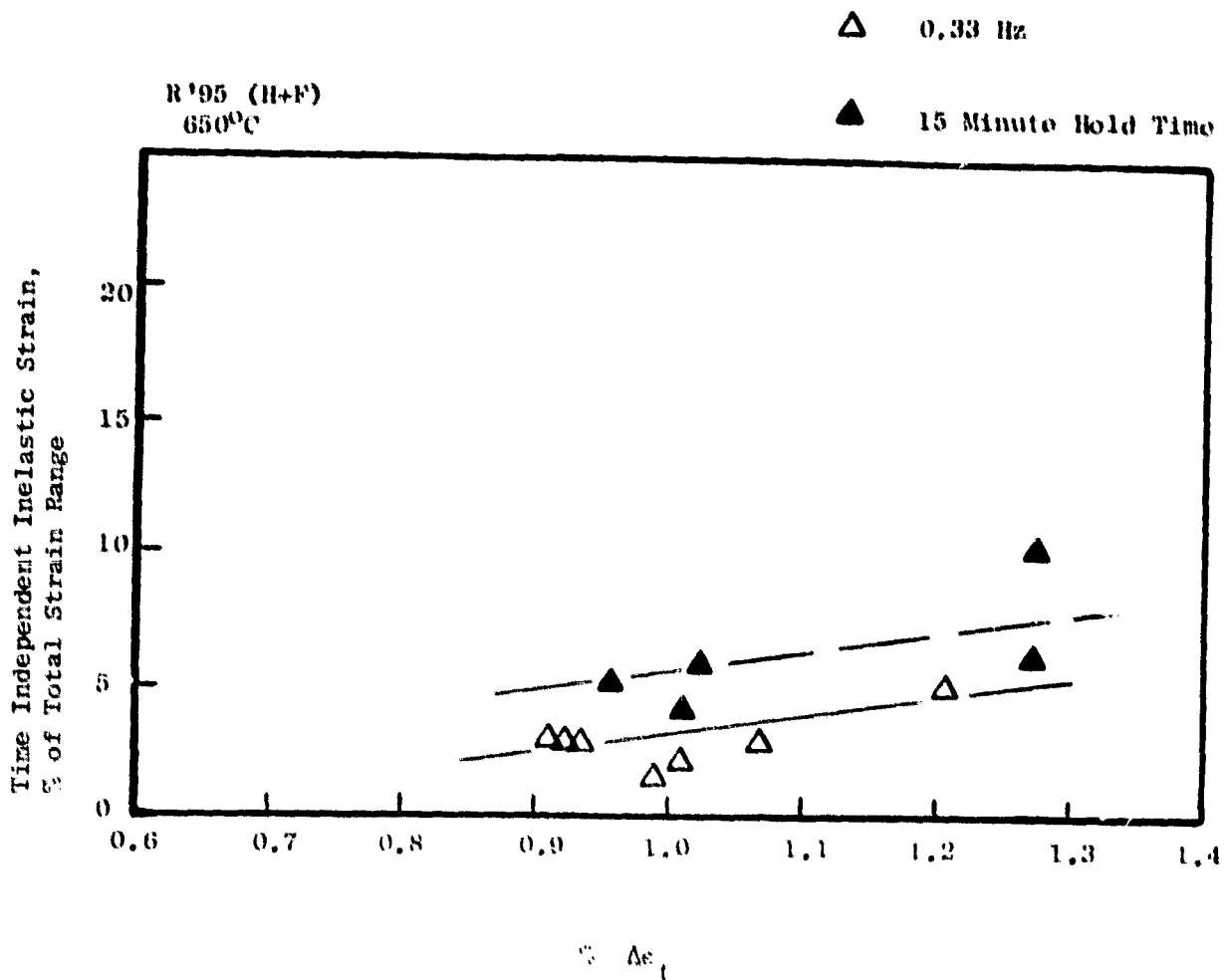
Figure 18. Percent Normalized Time Independent Total Strain Range ( \% \Delta \epsilon_p / \Delta \epsilon_t ) vs. Percent Total Strain Range ( \% \Delta \epsilon_t ).
