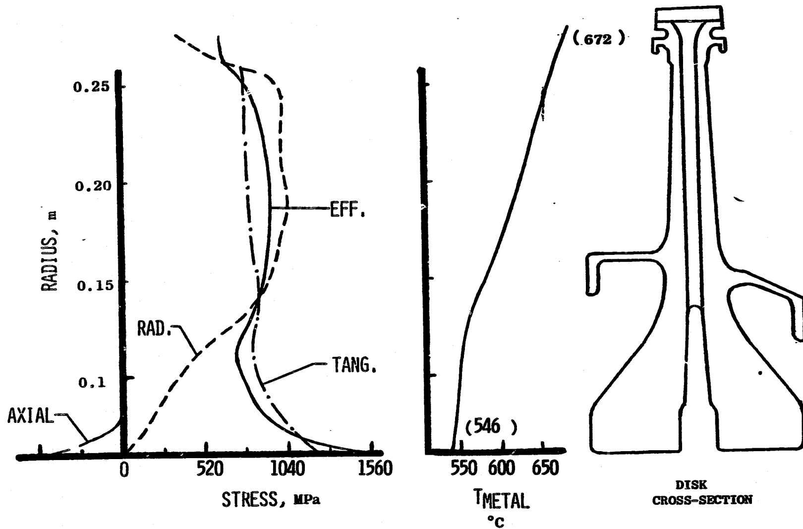
Figure 55. Stress and Temperature Distribution for Advanced Engine HPT Disk.
