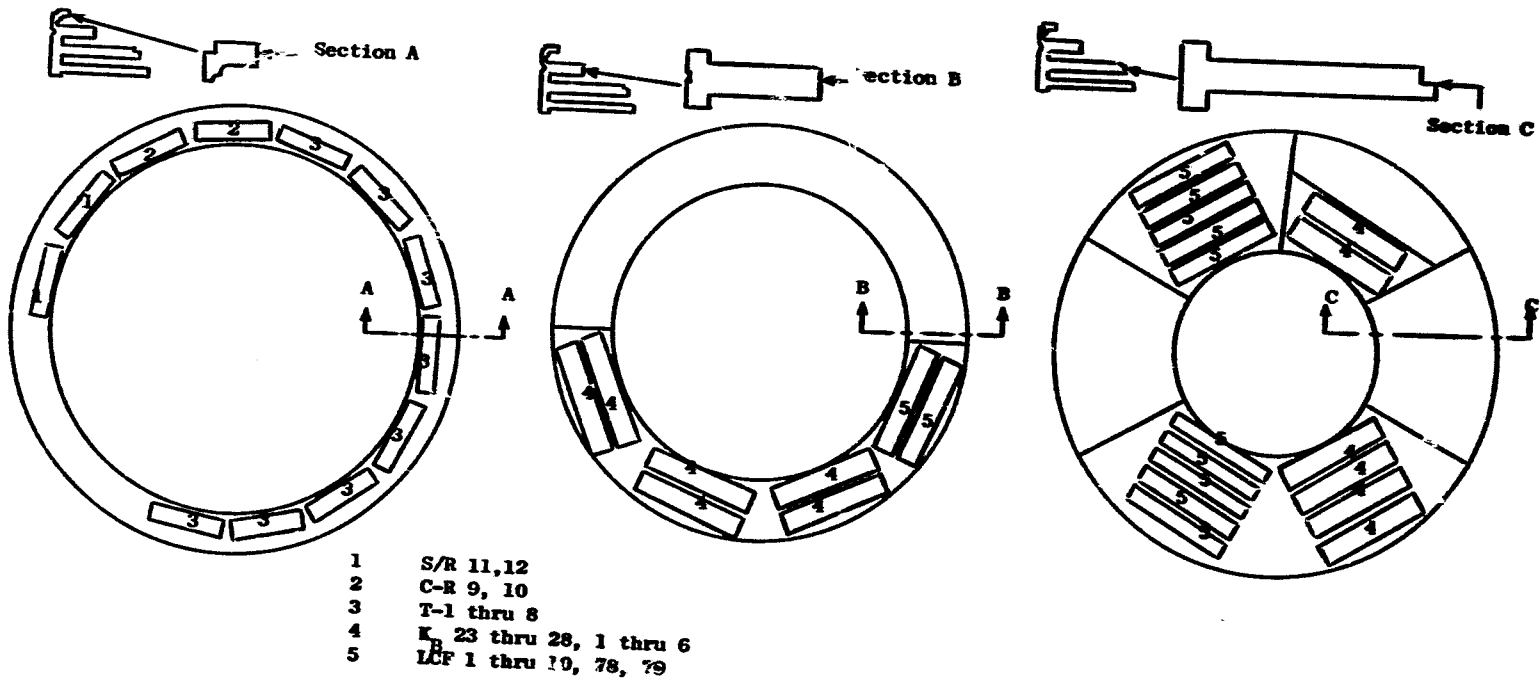
Figure 1. Specimen Cutup Arrangement - Inconel 718.
