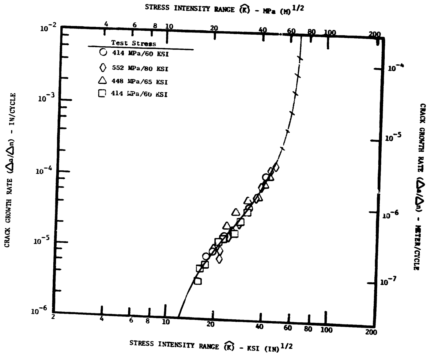
Figure 47. HIP + Forged René 95 Crack Propagation, 650° C, 0.33 Hz.
