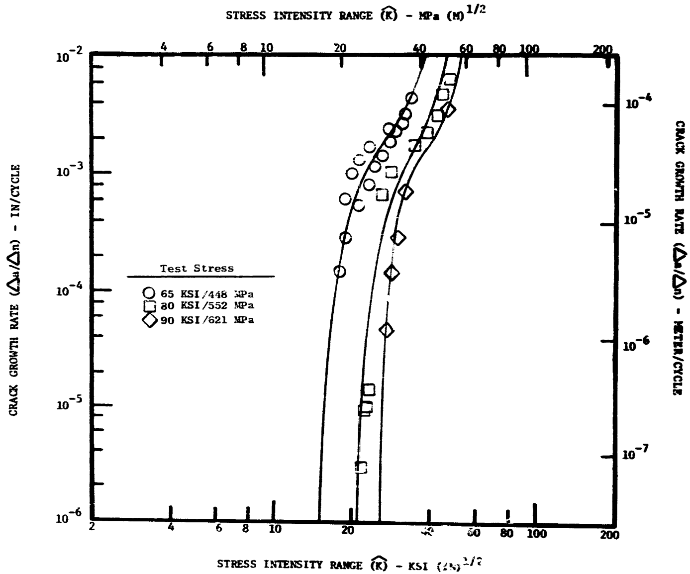
Figure 48. HIP + Forged René 95 Crack Propagation, t_h = 15 Minutes, 650^\circ\text{C} , A_\sigma = 0.95 .
