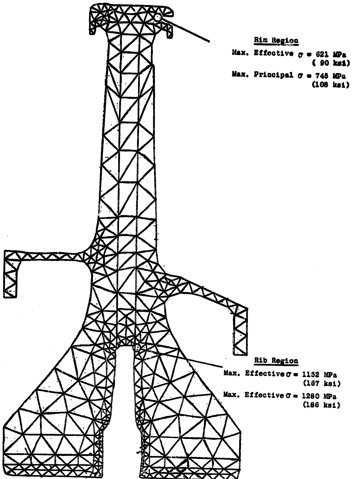
Figure 56. Advanced Engine Disk Finite Element Mesh Showing Critical Stress Locations.
