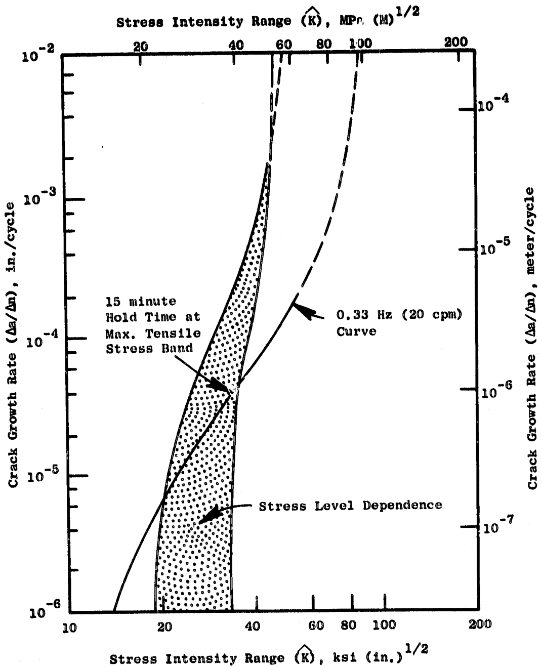
Figure 51. Cyclic Crack Growth Behavior for Inconel 718, Under Both Continuous and Hold Time Cycling Conditions at 650° C (1200° F).
