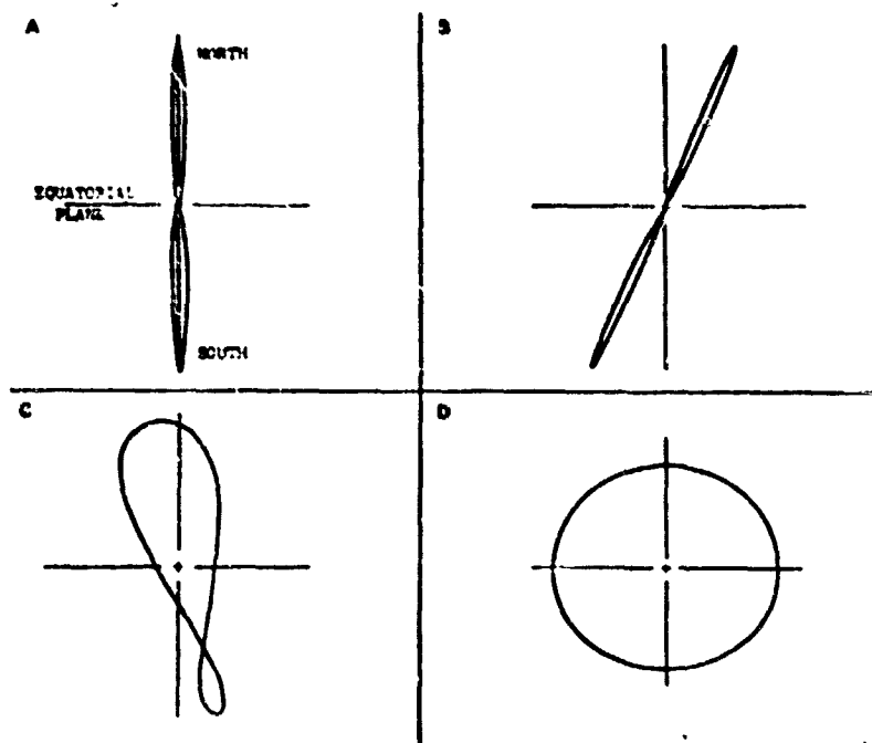
Figure 6-31. Subsateellite Track
