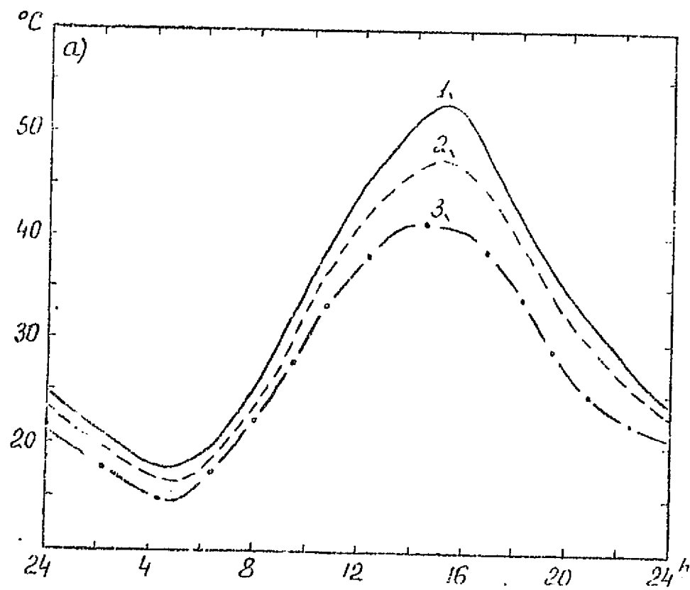
Fig. 37. Daily course of temperature: a) on road surfaces on a cloudless summer day [37], 1-3" asphalt layer; 2-packed sandy soil; 3-9" concrete layer; b) [3] 1-on a dirt road; 2-on a wormwood plain; 3-in a damp hollow with thick meadow vegetation.
