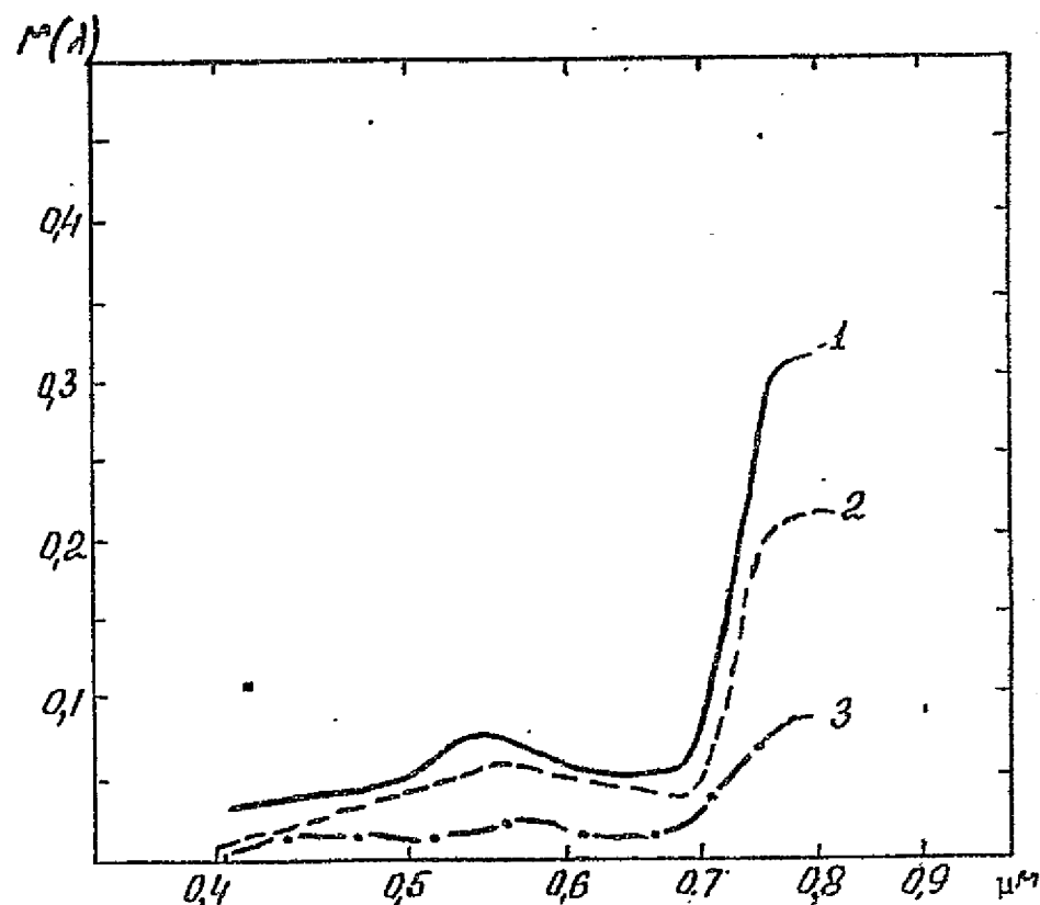
Fig. 30. Spectral brilliance coefficients a) [17] wormwood in budding stages on a rocky talus with various areas of projected covering: 1- S_n=100\% , 2- S_n=80\% , 3- S_n=50\% , 4- S_n=0 ; b) 18 pine with crowns of various thicknesses: 1-100%, 2-80%, 3-50%.
