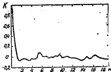
Fig. 10 [20] K(\rho) and Q(\rho) for a calm water surface ( \lambda = 0.55 + i0.70 ).
