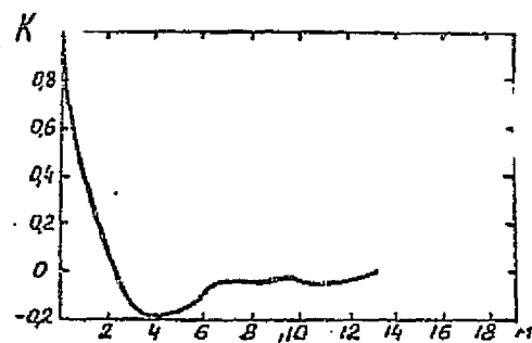
Fig. 7. [20] K(\lambda) and Q(\lambda) of an oak grove with birch and aspens ( a\lambda = 0.55 + 0.70i ).
