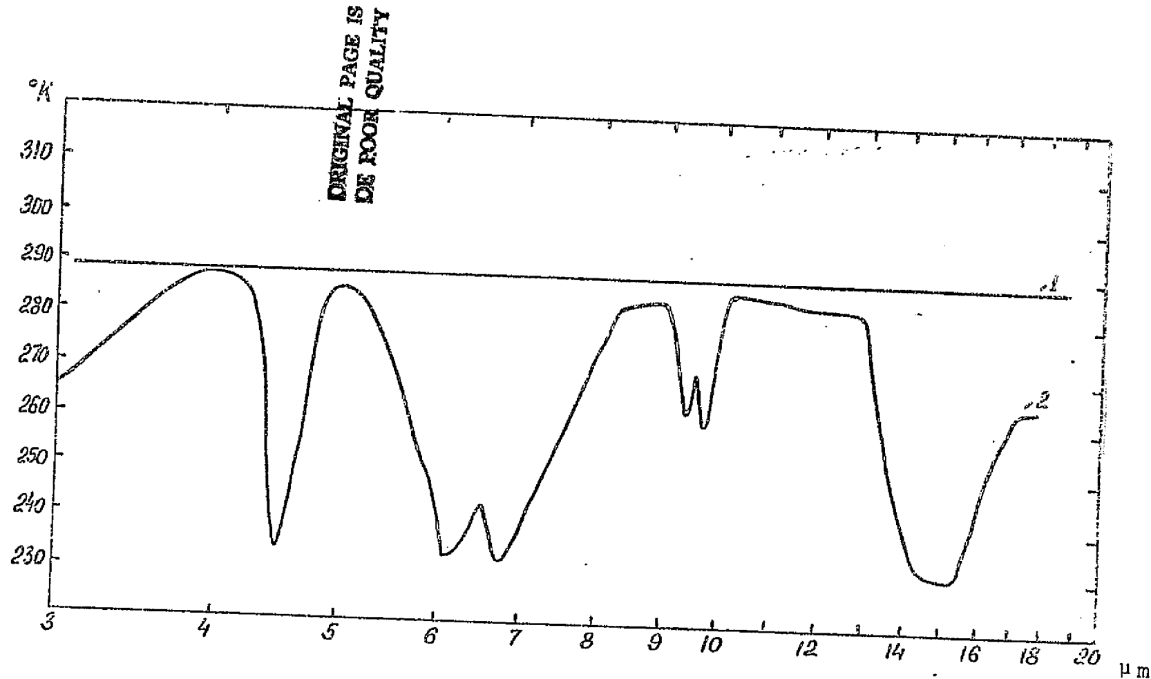
Fig. 47. [6] Spectral distribution of brilliance temperature values of an underlying surface, Leningrad, July: 1-true temperature; 2-radiative temperature.
