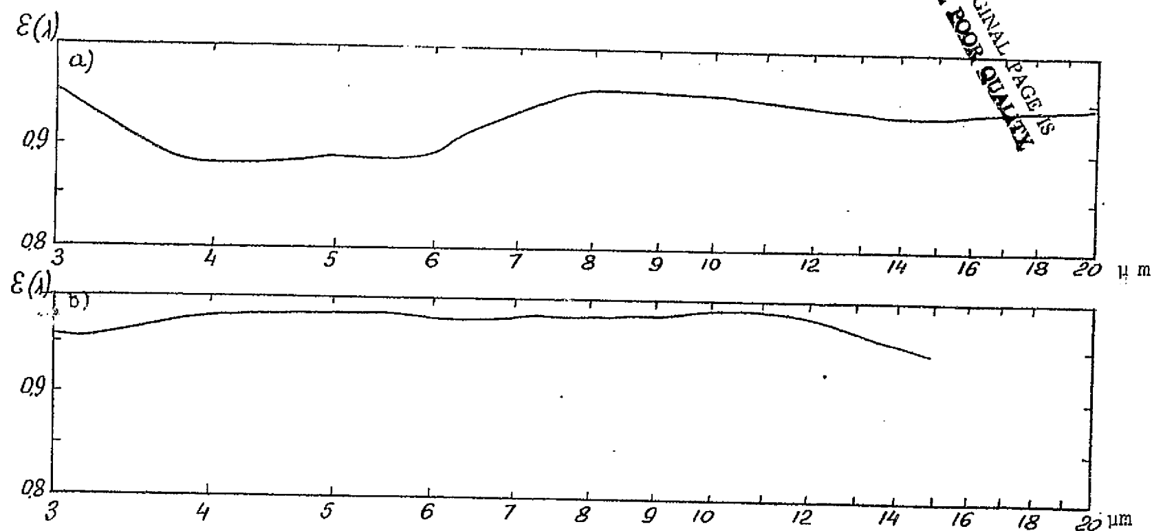
Fig. 36. Spectral radiation coefficients: a)-green leaf of an indoor lemon [19]; b)-water ( \theta=0 ) [2].
