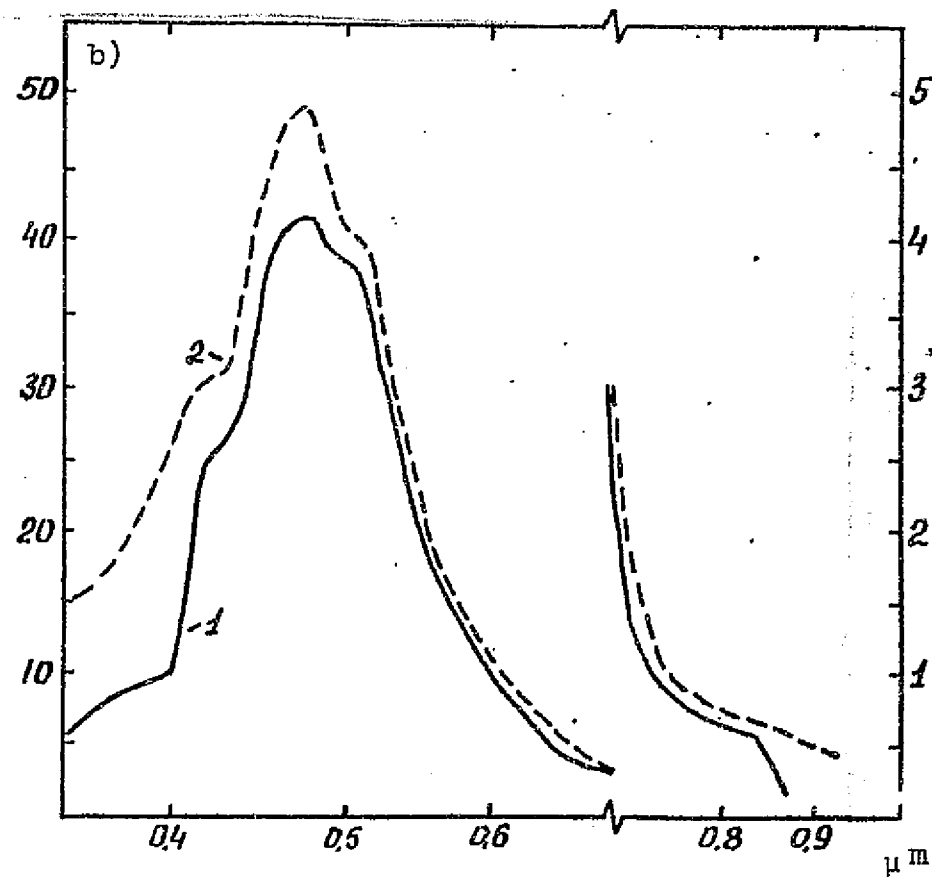
Fig. 29. Spectral brilliances of the surface of the ocean, a) [39] with chlorophyll concentration: 1-0.0..., 2-0.2 \text{mg}/\text{m}^3 ; b) [42] 1-clean surface; 2-surface covered with petroleum film.
