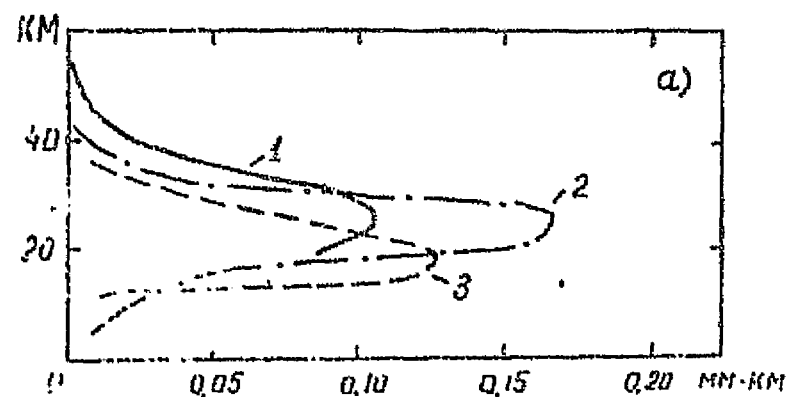
Fig. 41. Ozone concentration in the earth's atmosphere: a) the amount of ozone in a vertical path in mm in 1km at a given altitude [24]; 1-June; 2-October; 3-April.
