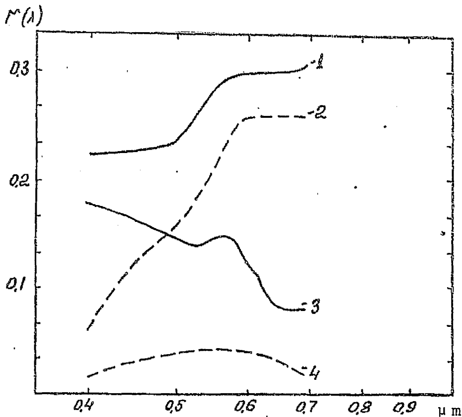
Fig. 45. [9] Spectral brilliance coefficients for two types of underlying surfaces, measured from space and from the surface of the earth: 1-sand, H=250 km; 2-sand, H=0 ; 3-water, H=250 km; 4-water H=0 .
