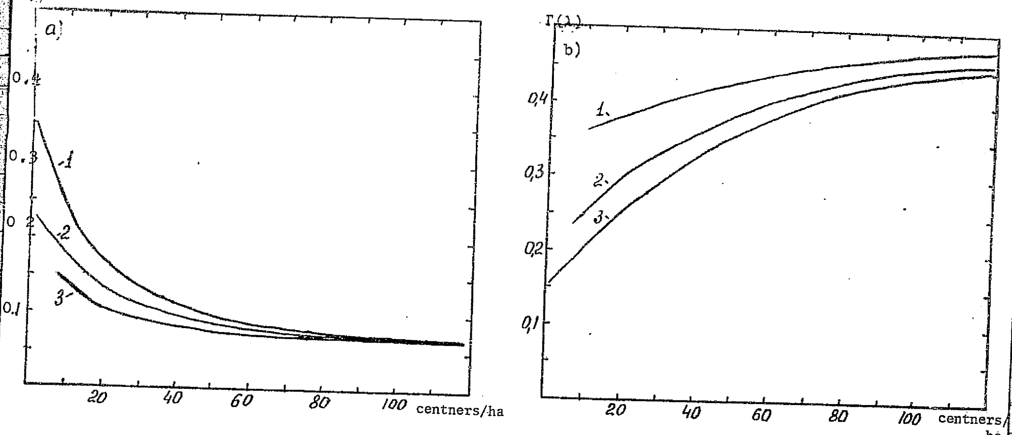
Fig. 31. [9] The relation between the brilliance coefficients of soil-plant covering systems and the quantity of green mass for various types of soil in the spectral intervals 0.59 \div 0.72 \mu\text{m} (a) and 0.68 \div 1.2 \mu\text{m} (b). 1- clay soil, 2-light sand, 3-dark sand
