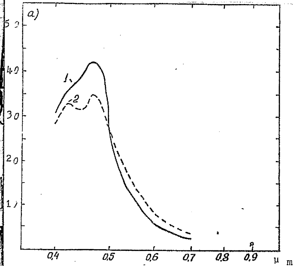
Fig. 29. Spectral brilliances of the surface of the ocean, a) [39] with chlorophyll concentration: 1-0.0..., 2-0.2 \text{mg}/\text{m}^3 ; b) [42] 1-clean surface; 2-surface covered with petroleum film.
