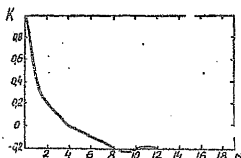
Fig. 9. [20] K(\lambda) and Q(\Omega) for a low-land swamp ( \lambda = 0.55 \pm 0.70 ).
