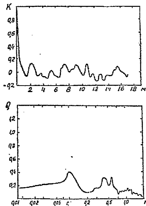
Fig. 5. [20] K(\lambda) and Q(\lambda) of fresh-plowed field ( \Delta\lambda = 0.55 \pm 0.70 \mu\text{m} ).
