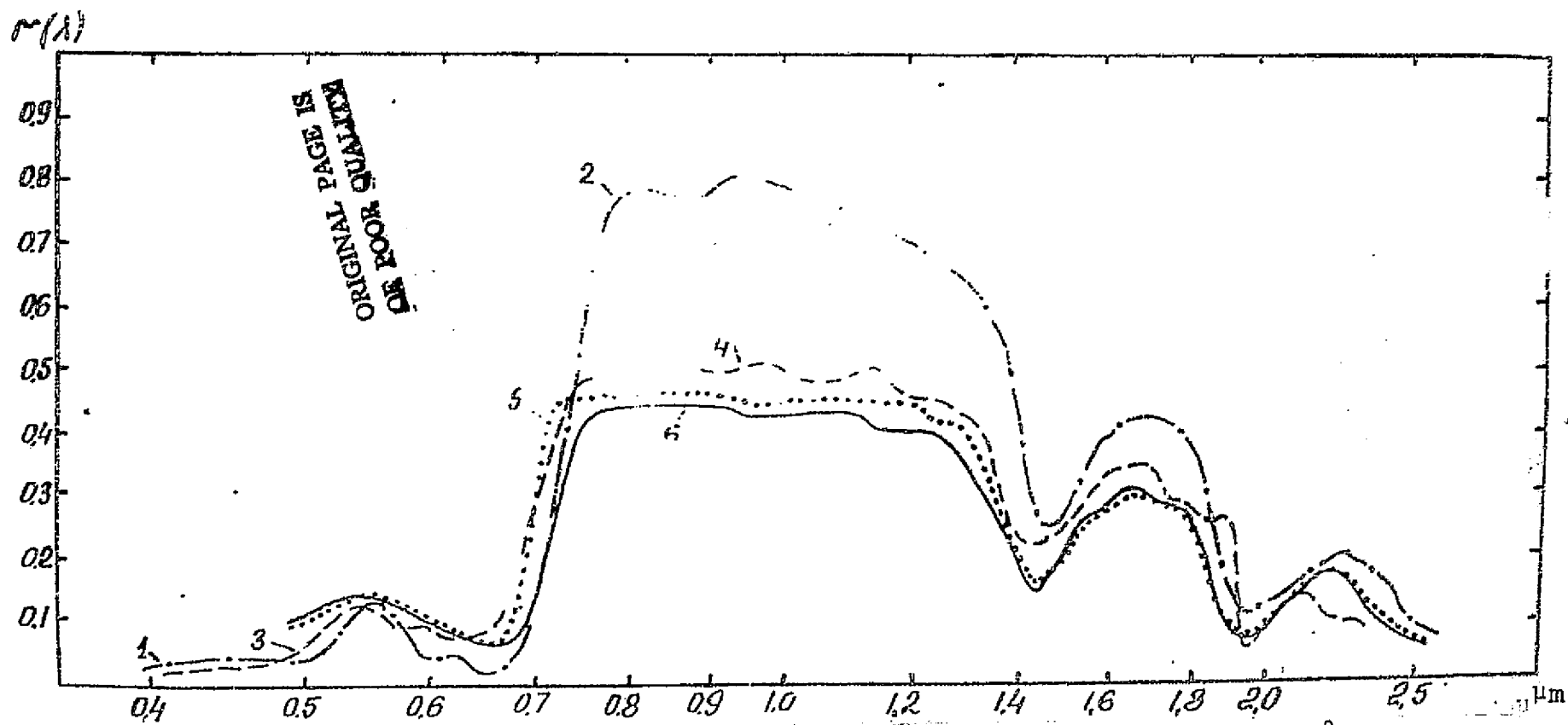
Fig. 13. Spectral brilliance coefficients of: 1- grass [15]; 2- meadow grass, mowed [13]; 3- birches [15]; 4- birch leaves [13]; 5- cotton leaves [33]; 6- corn leaves [33].
