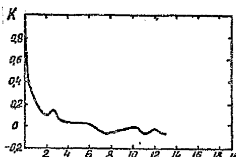
Fig. 8. [20] K(\lambda) and Q(\Omega) of a mowed meadow of various grasses and word illegible ( \lambda = 0.55 \pm 0.70 \mu\text{m} ).
