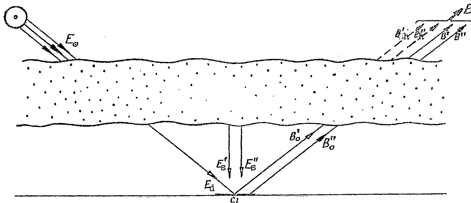
Fig. 43. Transfer of radiation currents in the earth's atmosphere. E_0 -density of solar radiation on the upper limit of the earth's atmosphere; E_d, E_s', E_s'' -irradiation of object c_1 ; direct and scattered solar radiation and thermal back radiation in the atmosphere; B_o' and B_o'' - brilliancy of object c_1 due to reflected solar radiation and inherent radiation; B -remote measurement (observed) of the brilliancy of object c_1 ; B_h' and B_h'' - basic components of remote measurements of brilliancy B , coming from object c_1 ; B_h' - reflected and inherent radiation; B_h'' - atmospheric haze brilliancy caused by scattering; B_h'' - brilliancy of inherent radiation in the atmosphere.
