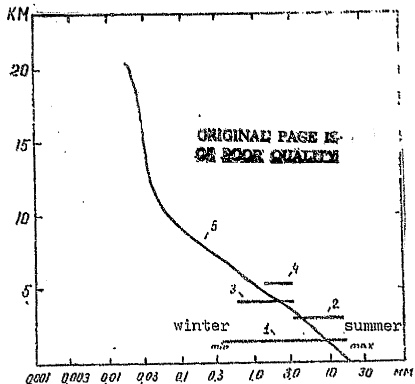
Fig. 40. [24] The water vapor concentration in the earth's atmosphere in a vertical path in mm from precipitated water at a given altitude: 1-Denver, USA; 2-El'brus, USSR; 3-Evans, USA; (summer); 4-Chakartaya, Bolivia; 5-average global data.
