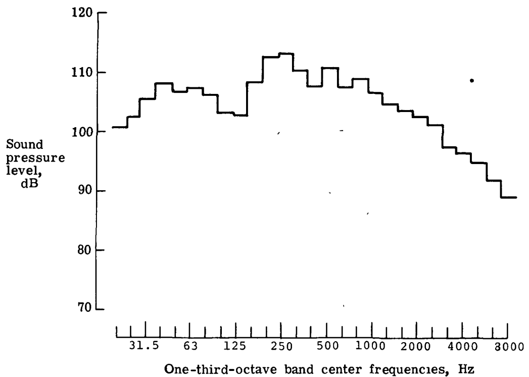
(a) Concorde.
