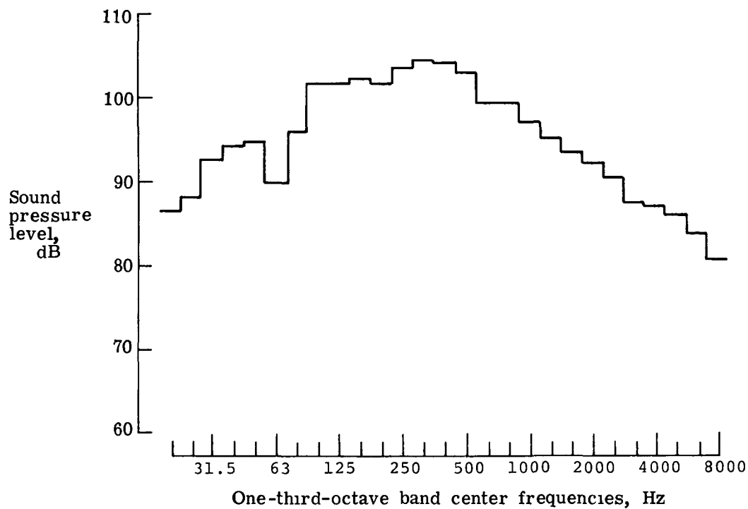
(a) Concorde.
