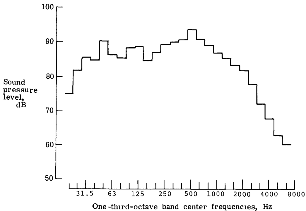
(a) Concorde.
