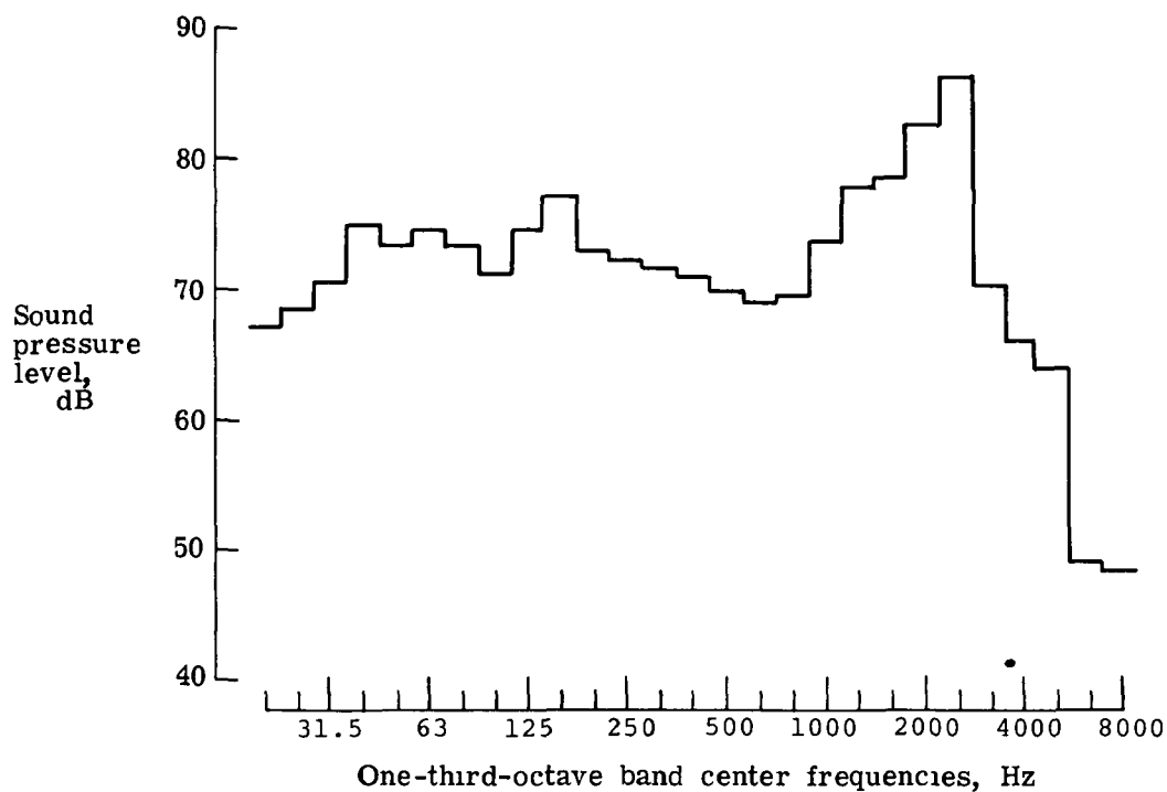
(c) B-707.
