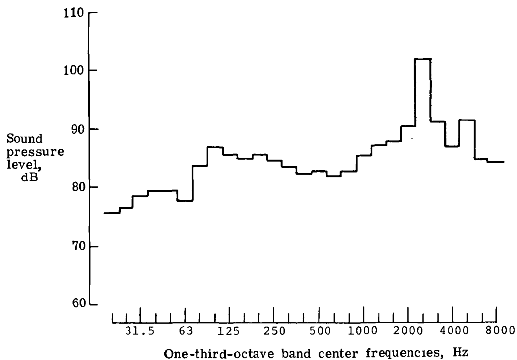
(c) B-707.
