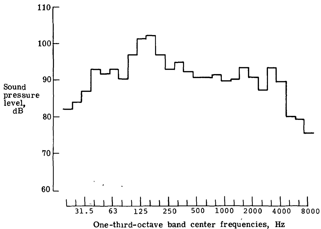
(c) B-707.
