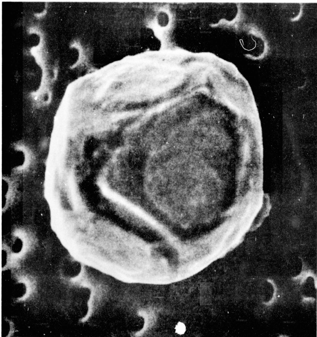
Fig. 15. SEM image of an unusual FSN particle, with octahedron and cubic crystal faces, from the U-2 stratospheric particle collection. Major elements are Fe, S; minor element is Ni [Brownlee et al., 1976].
