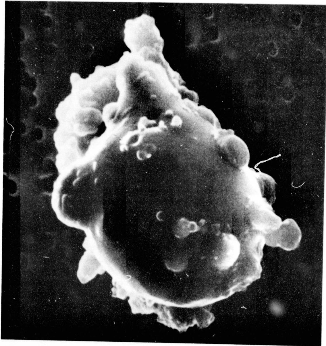
Fig. 17. SEM image of an unusual round chondritic particle covered with Fe-Ni mounds. Major elements are Si, Mg, Fe; minor elements are Ca, Al, Ni, and Cr [Brownlee et al., 1976].
