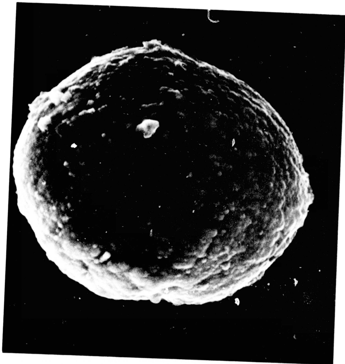
Fig. 6. SEM images of spherules ablated from the Murchison meteorite: (b) sulfide sphere composed of magnetite, pyrrhotite, and wüstite.
