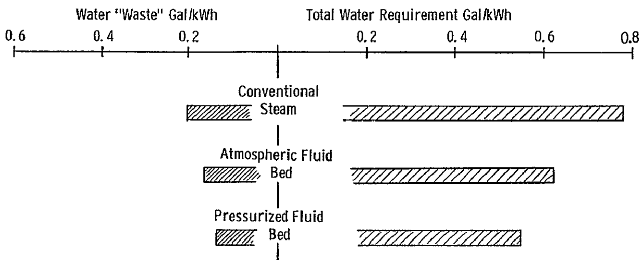
Figure 15. Water Requirement
