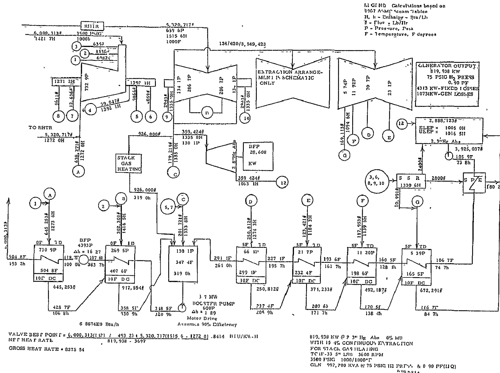
Figure 5. Conventional Furnace with Wet Scrub—250 F Stack
