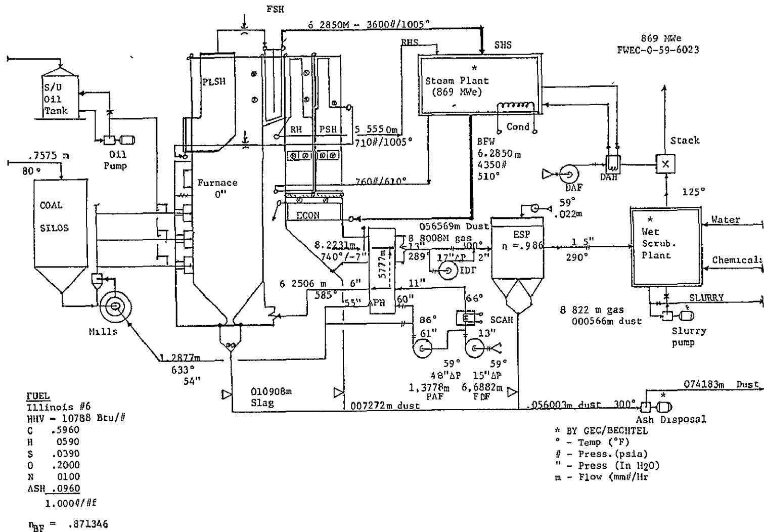
Figure 4. Conventional Steam Plant Flow—860 MWe
