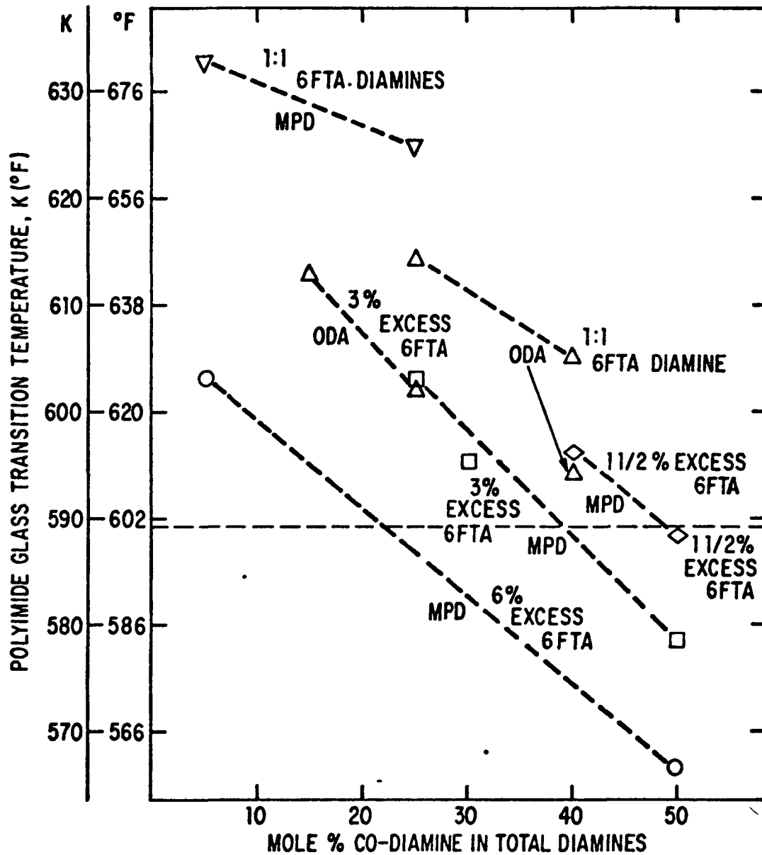
FIGURE 1 EFFECT OF CHEMICAL COMPOSITION OF NR-150 TYPE POLYIMIDES ON POLYMER T g (6 FTA/PPD/CO-DIAMINE SYSTEMS)
