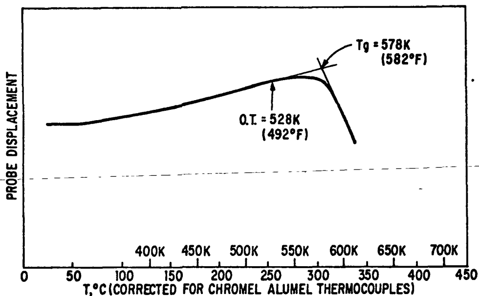
FIGURE 4 TMA CURVE OF ADHESIVE BOND LINE FROM SAMPLE 20 TABLE VII
