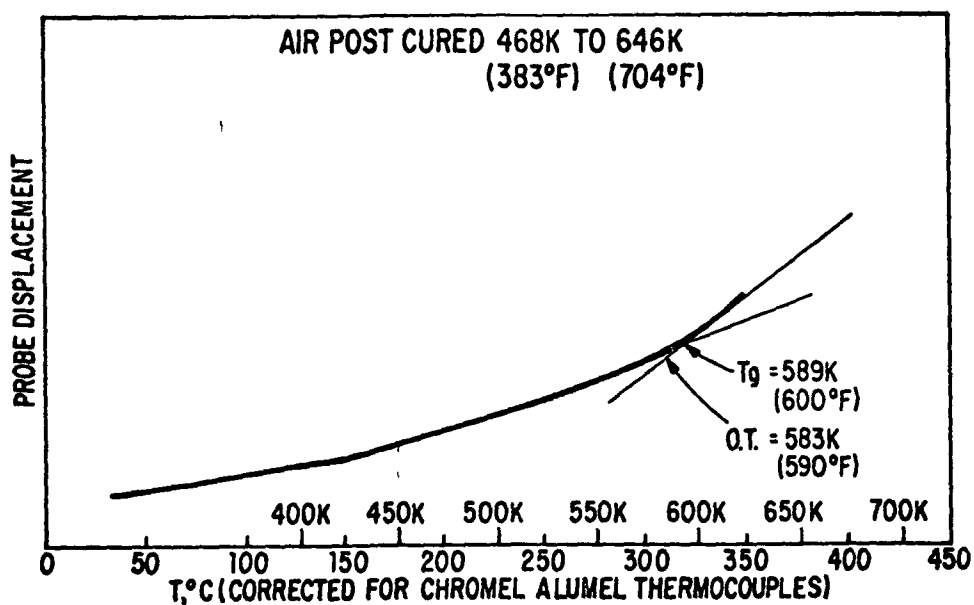
FIGURE 12 TMA CURVE OF ADHESIVE BOND LINE FROM SAMPLE 75 TABLE XI I
