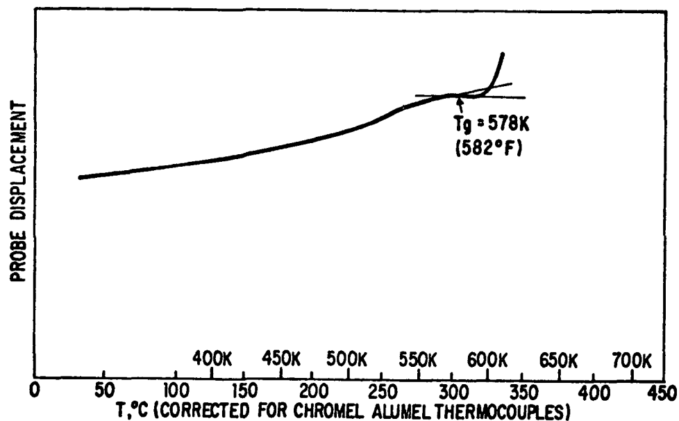
FIGURE 3 TMA CURVE OF ADHESIVE BOND LINE FROM SAMPLE 19 TABLE VII
