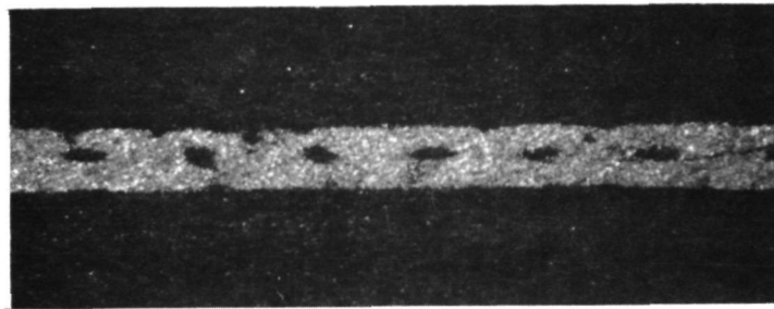
Bond Line Near Overlap Area (25X)
