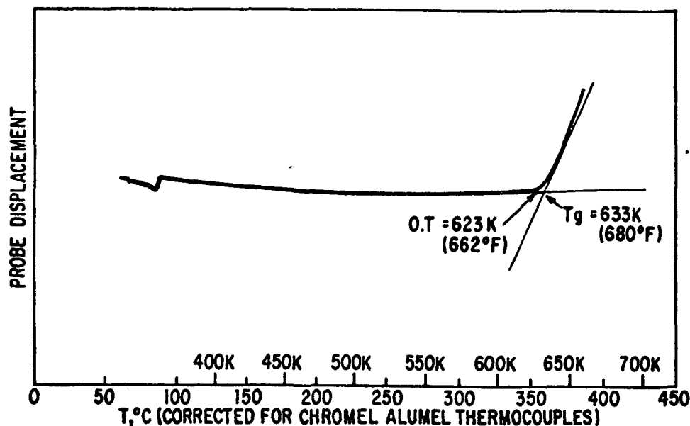
FIGURE 2. TMA CURVE OF LAMINATE MOLDED FROM NR-150B2G/GLASS CLOTH ADHESIVE PREPREG
