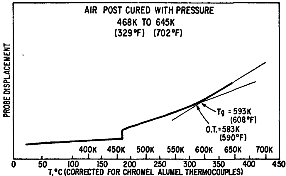
FIGURE 13 TMA CURVE OF ADHESIVE BOND LINE FROM SAMPLE 77 TABLE XI
