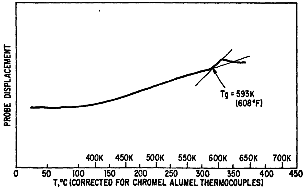
FIGURE 8 TMA CURVE OF ADHESIVE BOND LINE FROM SAMPLE 28 TABLE II
