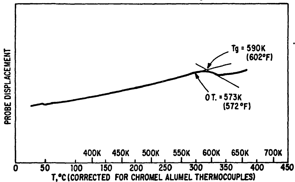
FIGURE 9 TMA CURVE OF ADHESIVE BOND LINE FROM SAMPLE 30 TABLE VIII
