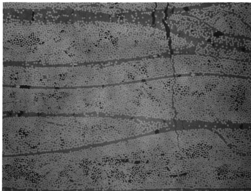
PICTURE MADE FROM AREA SHOWING GOOD C-SCAN USING 15 MHZ TRANSDUCER
