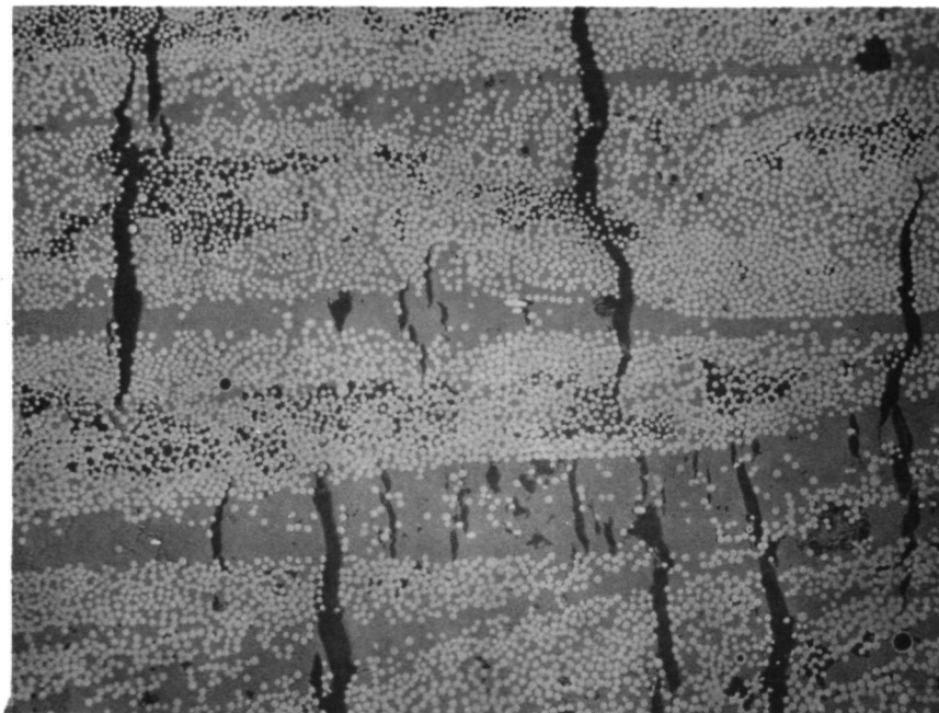
PICTURE MADE FROM AREA SHOWING POOR C-SCAN USING 15 MHZ TRANSDUCER
