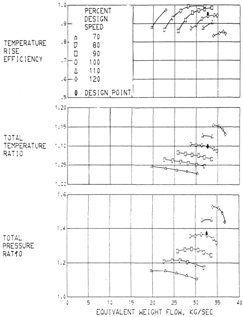
FIGURE 7. - OVERALL PERFORMANCE FOR ROTOR 53.
