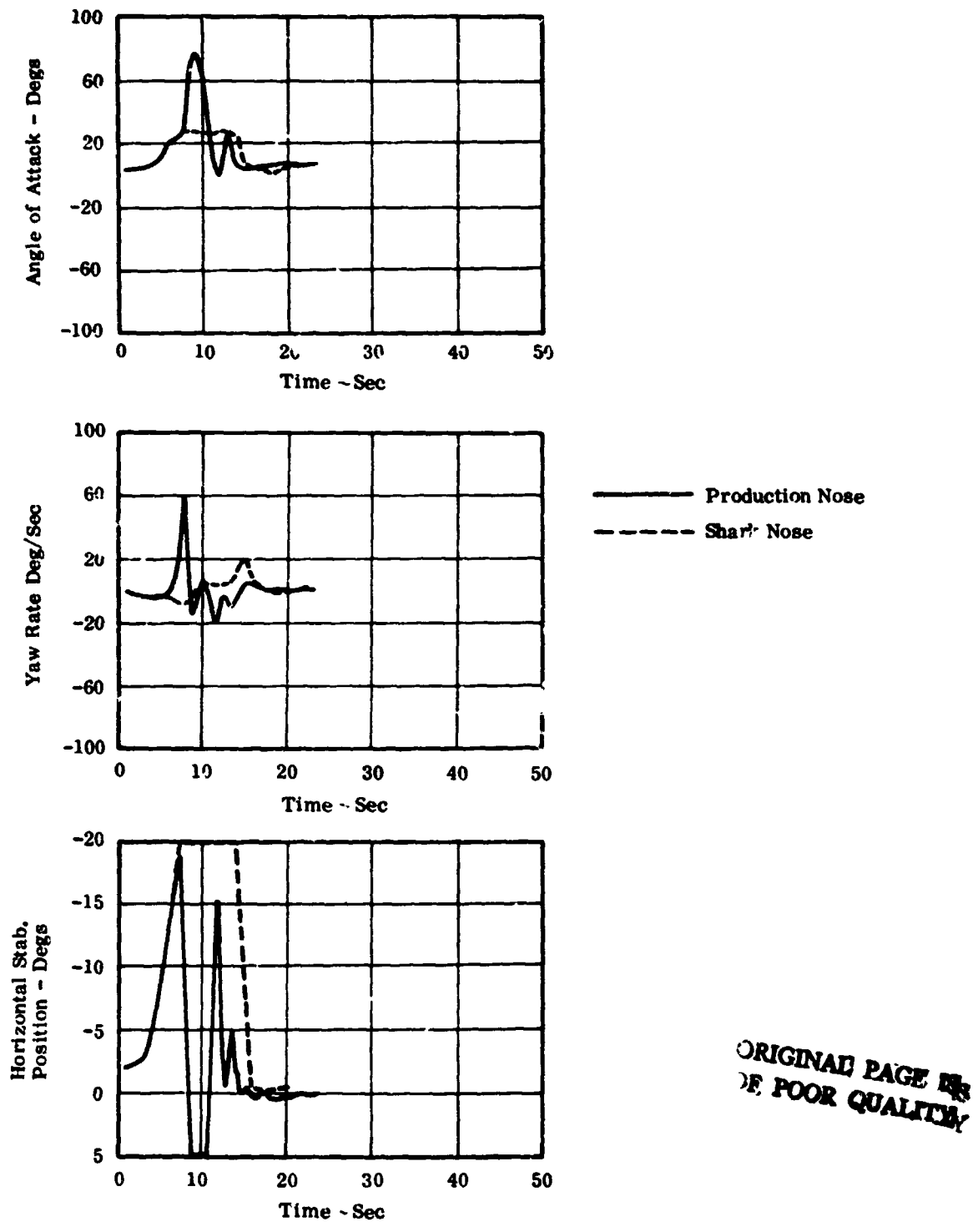
FIGURE 142. F-5F CENTERLINE TANK CONFIGURATION, 4-g LEVEL DECEL
