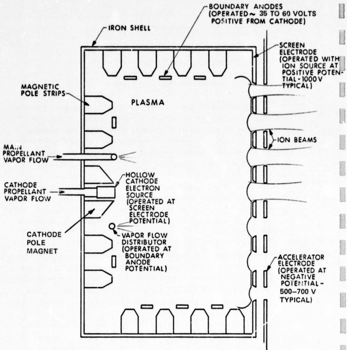
Figure 2-1. MESC Thruster Schematic
