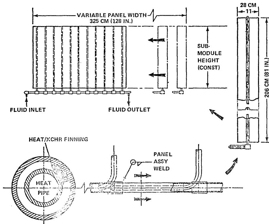
Figure 13. - Modular-heat-pipe radiator.
