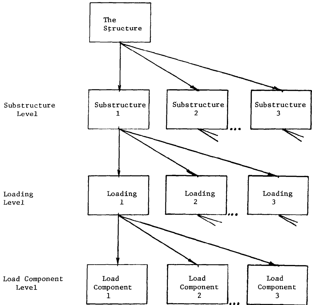
Figure 2.- Context tree.
