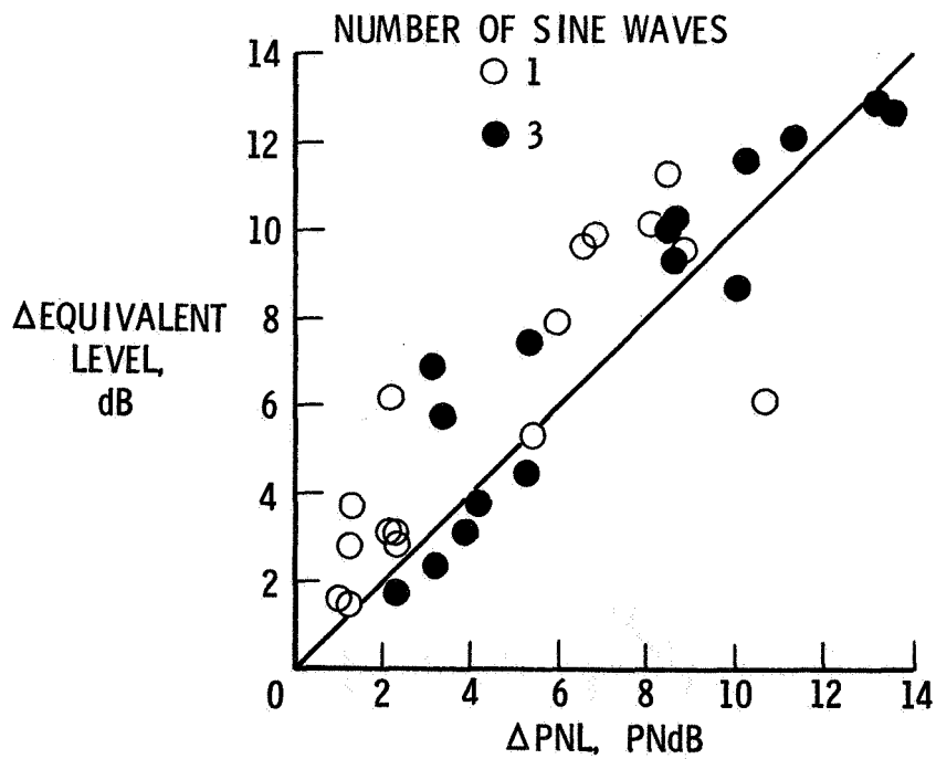
Figure 8.- Effects of impulsiveness for two numbers of sine waves comprising an impulse event.
