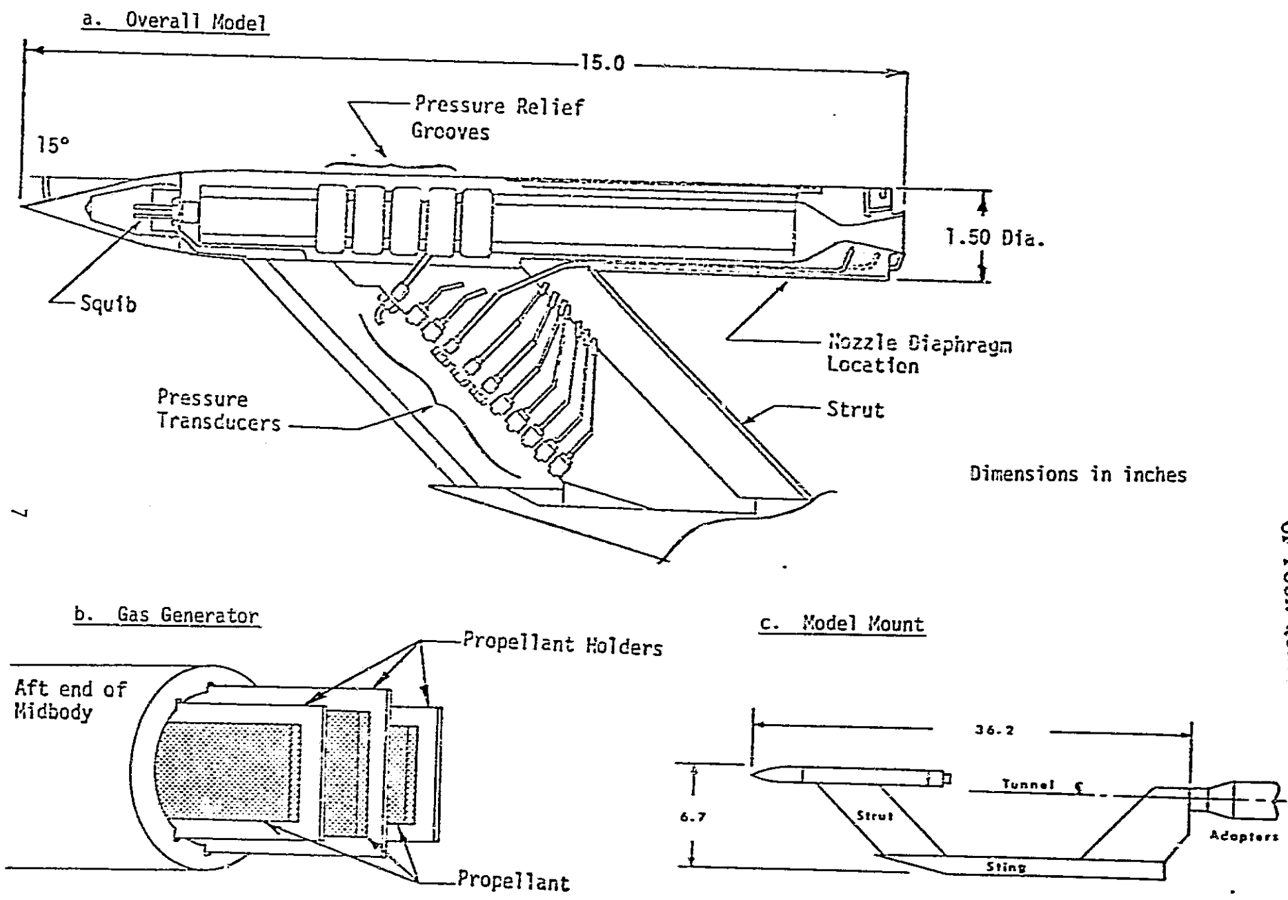
Figure 1 Task 1 Model Design
