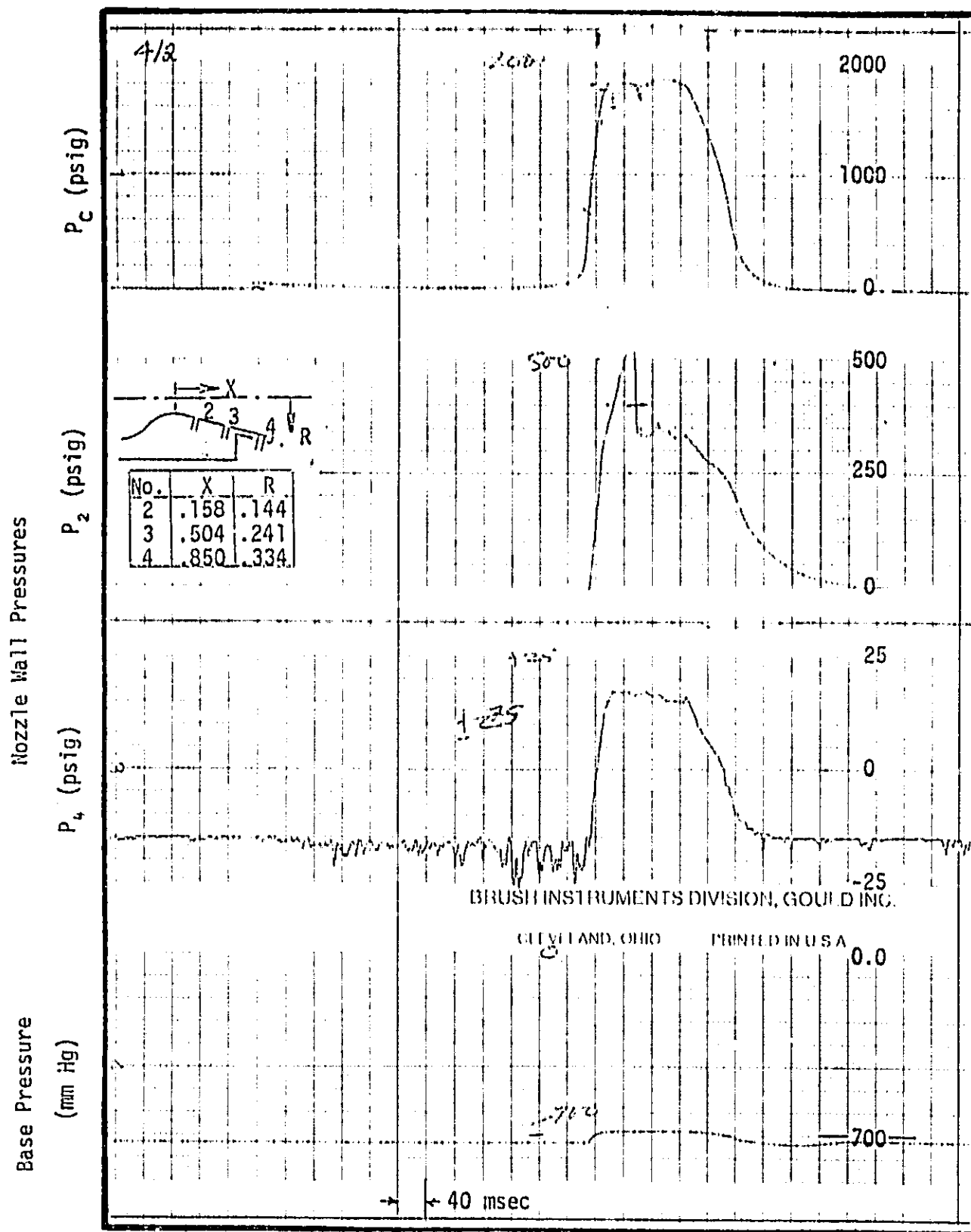
Figure 4. Typical Task 1 Time History of Pressures
