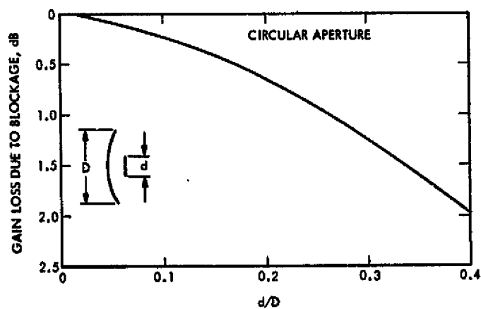
Figure 5. Gain Loss Due to Blockage
