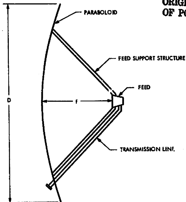
Figure 4. Front-fed Paraboloid
