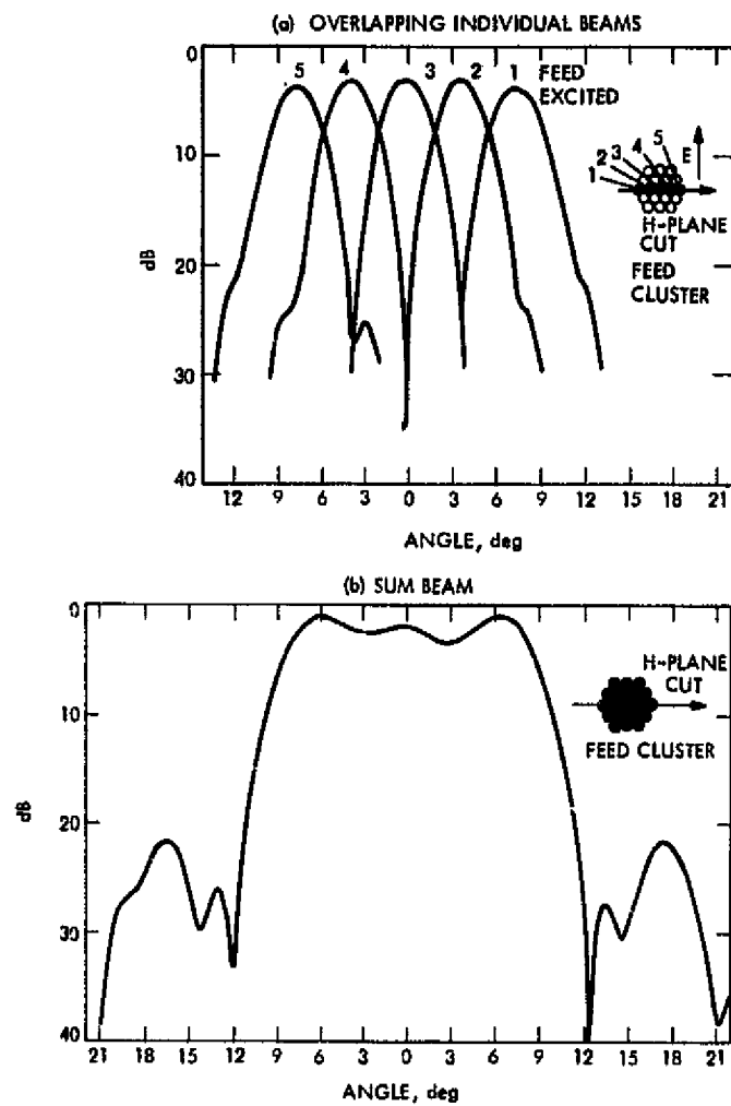
Figure 40. SUMBA Patterns
