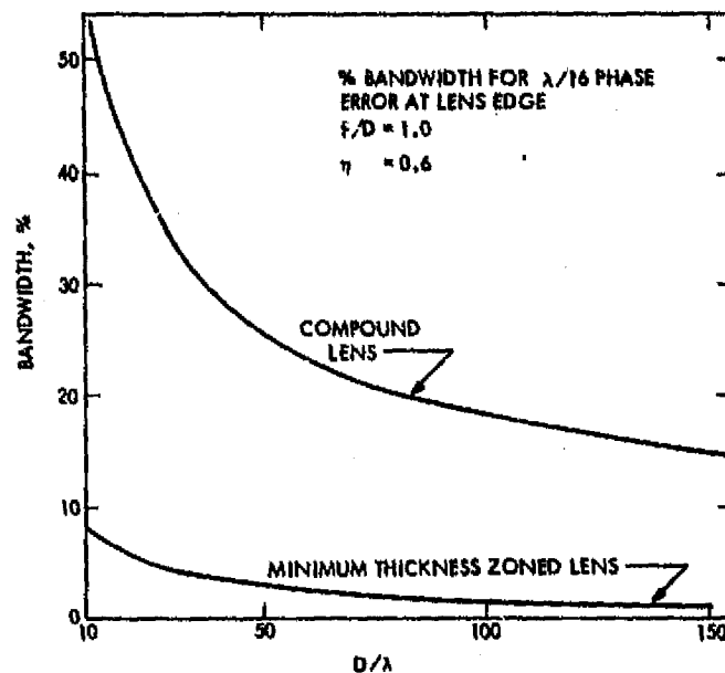
Figure 37. Bandwidth vs Lens Diameter for Compound and Simple Lenses
