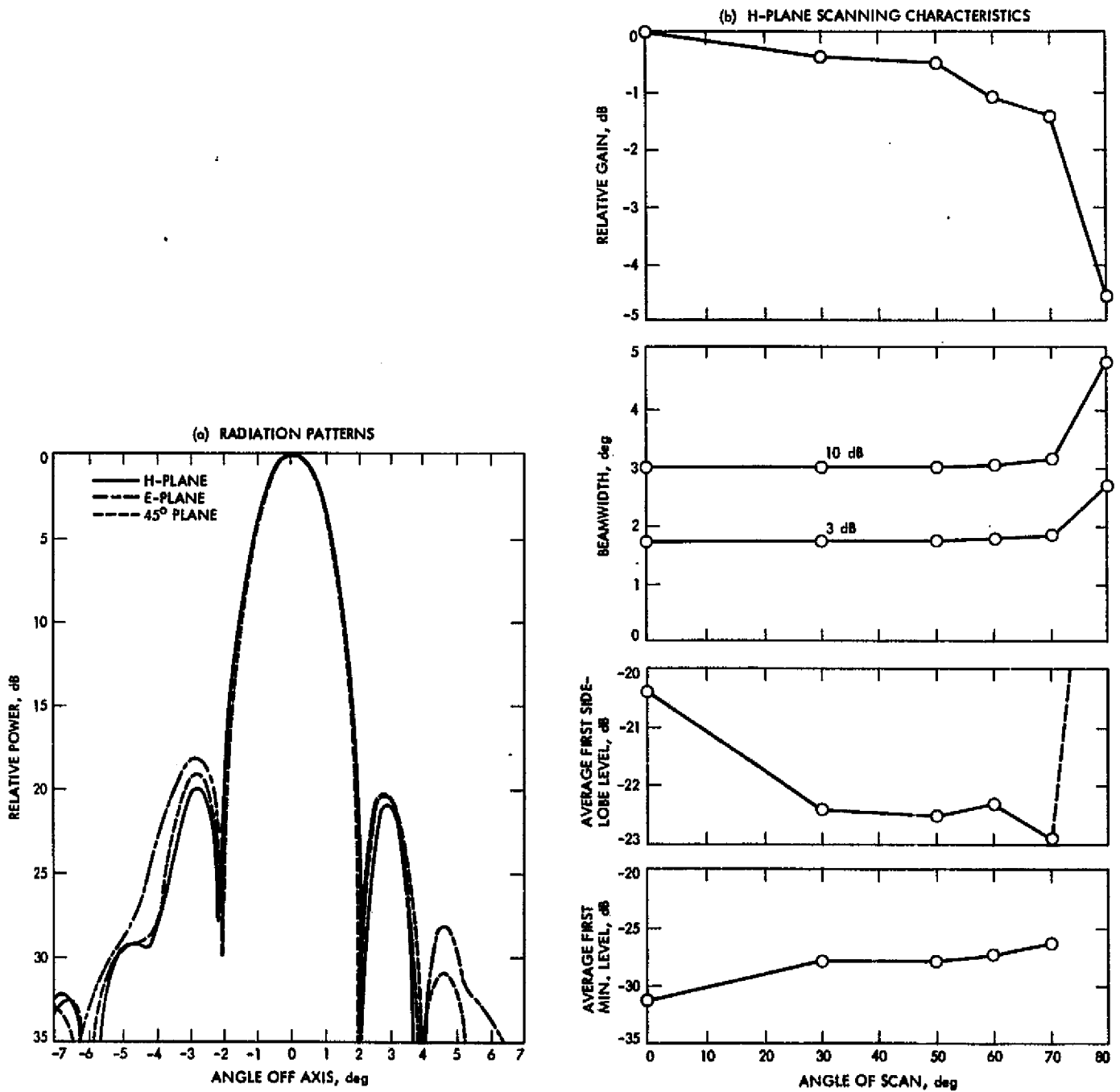
Figure 23. 3-m (10-ft) Spherical Reflector Scan Performance at 11.2 GHz
