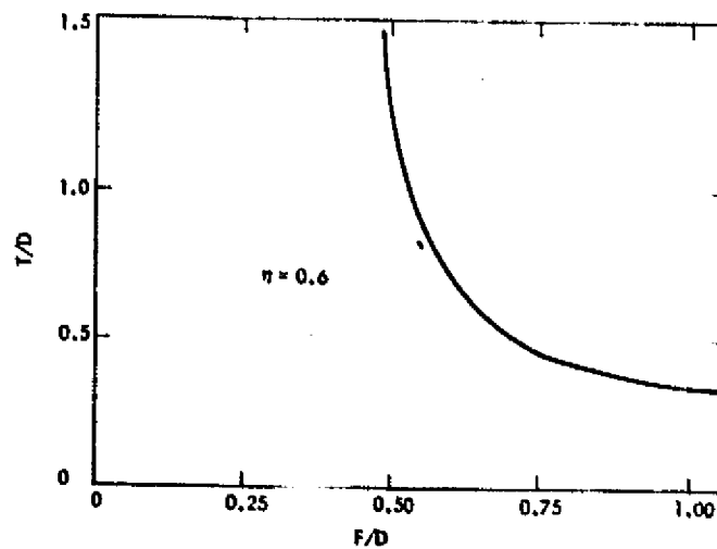
Figure 33. Unstepped Lens Maximum Thickness as a Function of F/D for \eta = 0.6
