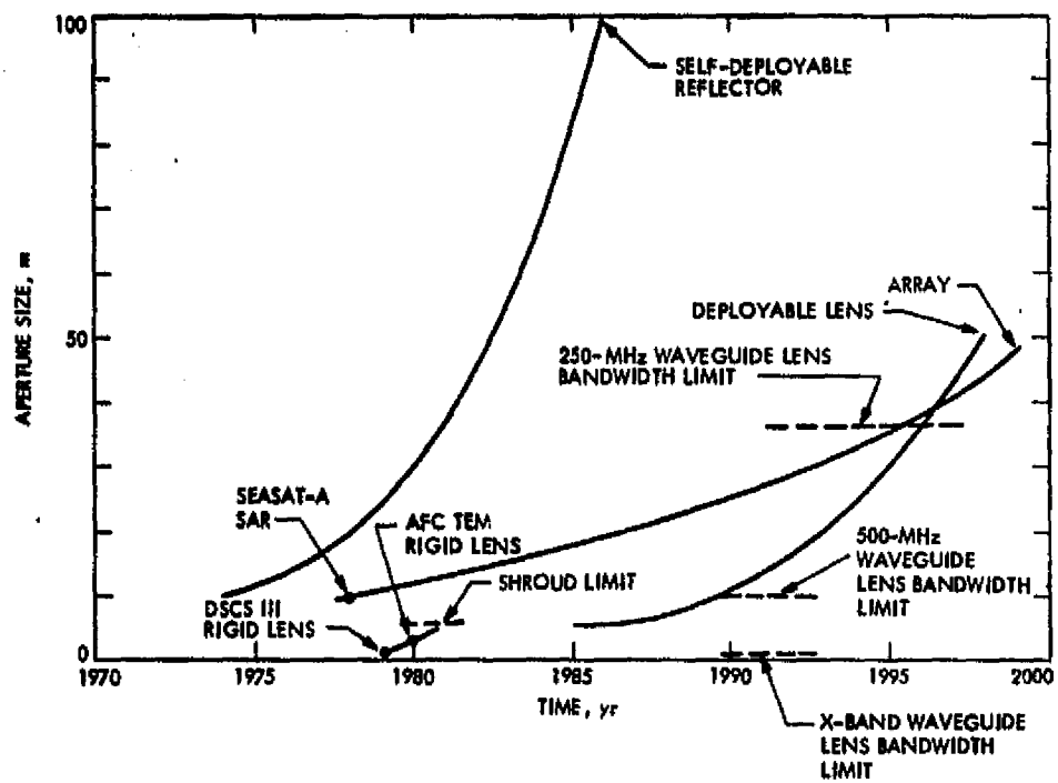
Figure 46. Antenna Size vs Time
