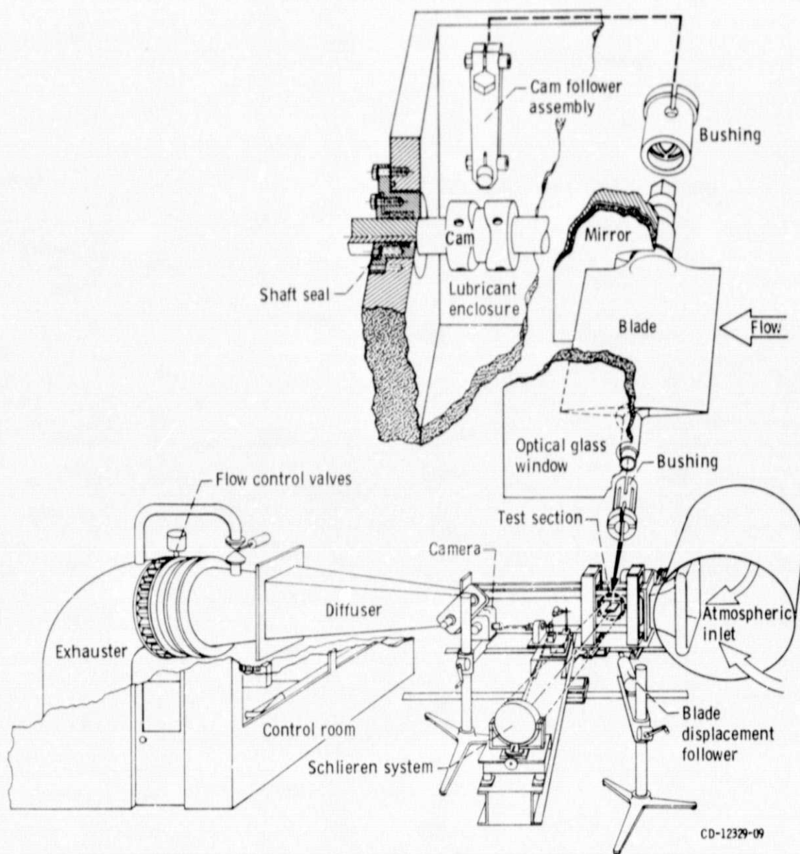
Figure 1. - Flutter test facility.
