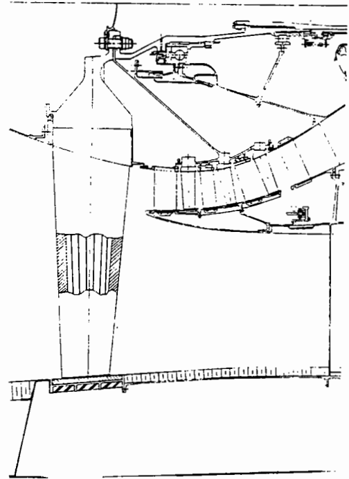
STF 505 M-9 DIRECT-DRIVE, 2 STG HPT
