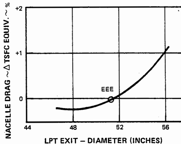
Figure C-40 Low Rotor Trade Study – The effect of low-pressure turbine diameter on nacelle drag is shown.
