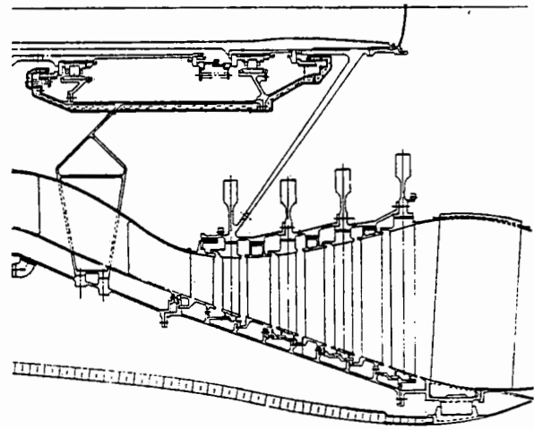
STF 505 M-9 DIRECT-DRIVE, 2 STG HPT
