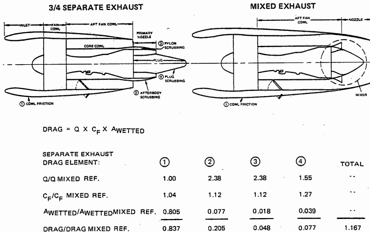
Figure 19 Nacelle Friction Drag Build-up - Mixed exhaust and 75 percent length separate exhaust nacelles.
