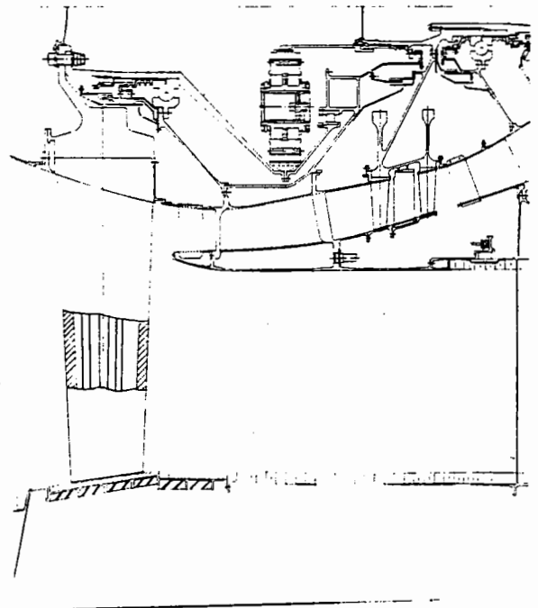
STF 495 M-5 GEARED, 2 STG HPT
