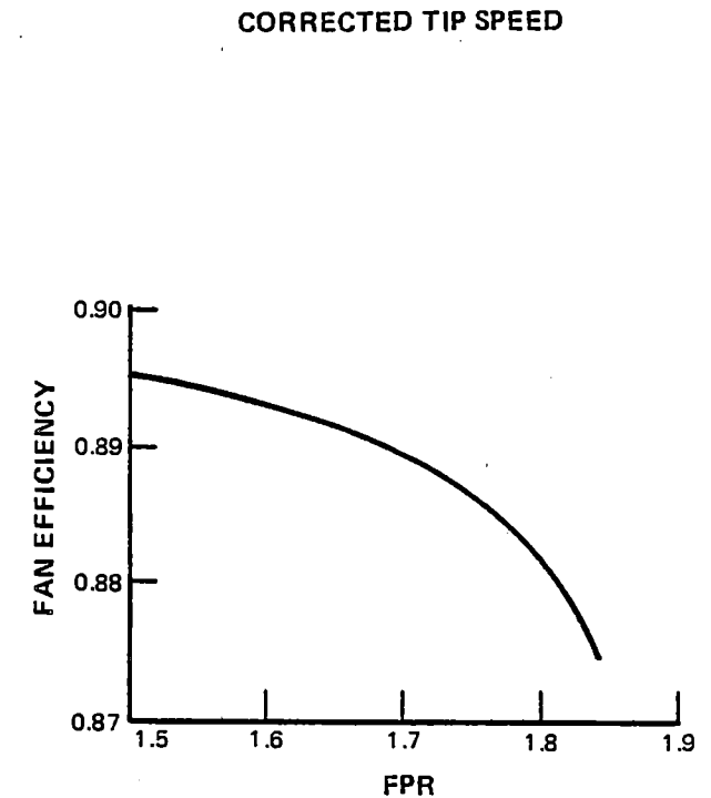
Figure C-93 Geared Engine Fan Efficiency Trends for Growth
