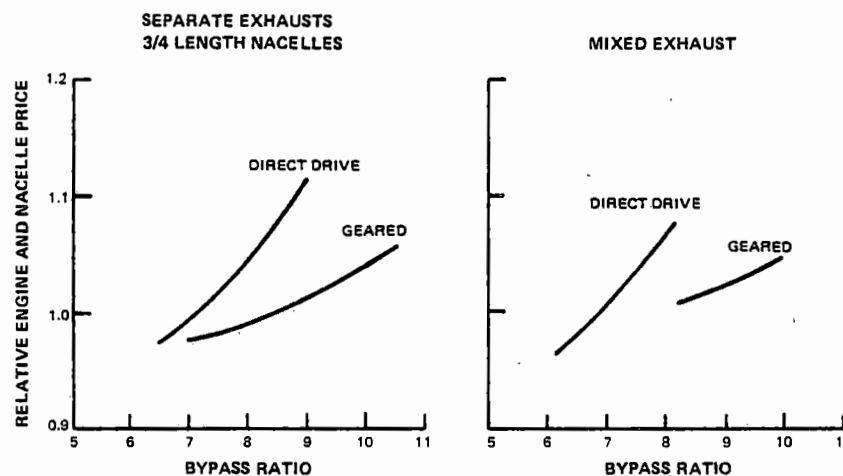
Figure B-15 Task II Total Engine and Nacelle Price Trends (Max. Cruise Thrust = 42.1 kN, OPR = 38.6, RIT = 1210°C). Price trends were similar to weight trends.
