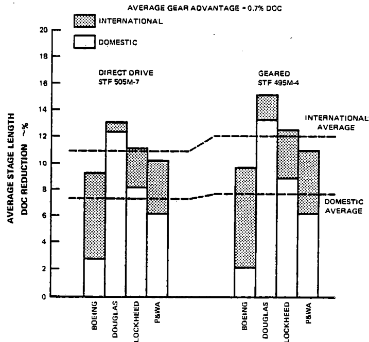
Figure C-88 Task III Average Mission Direct Operating Cost Reductions – Shows reduction relative to the JT9D-7A
