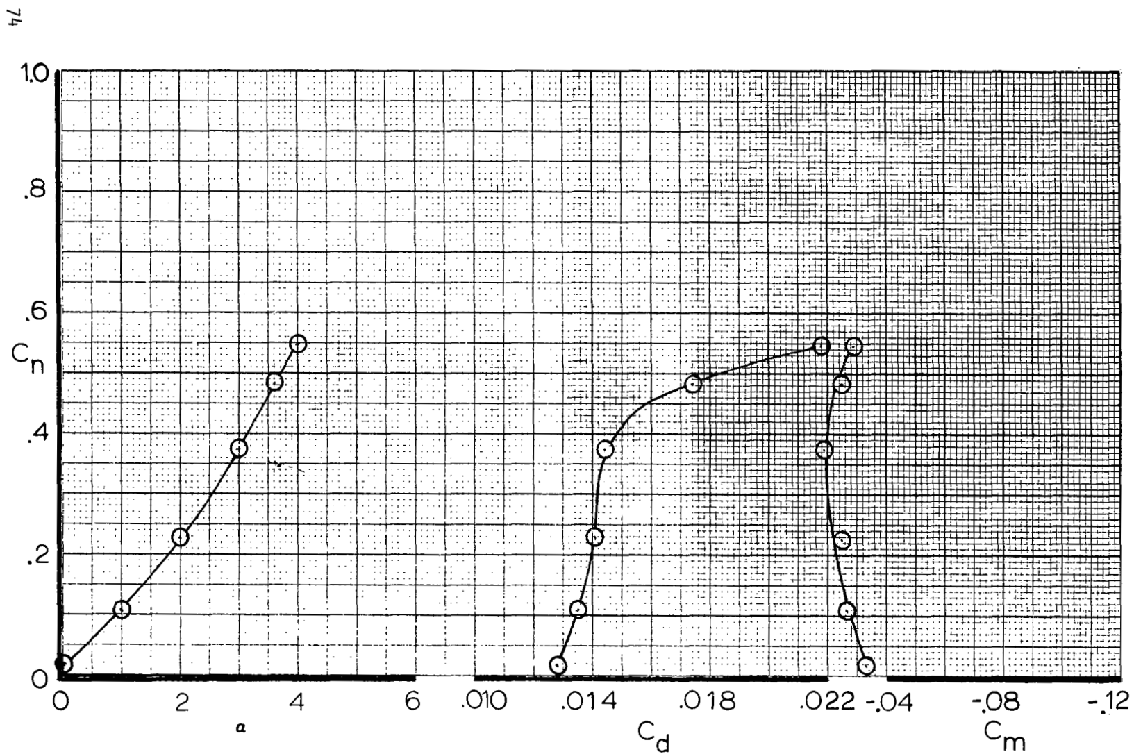
Figure A13. - Airfoil force data for M=0.78 , R_N=4 \times 10^6 , X/C_T=.05
