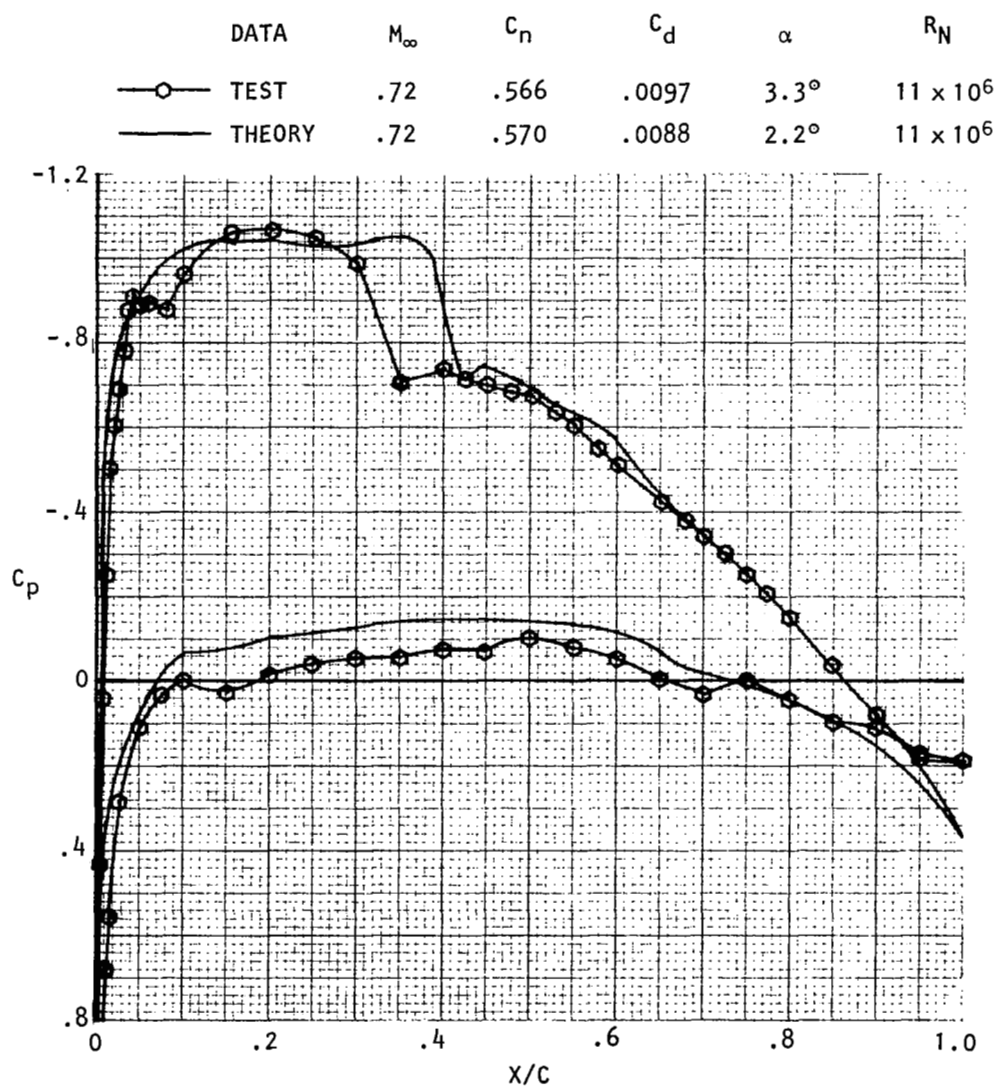
Figure 1. Design point theoretical and experimental pressures for the baseline airfoil (C141-1).
