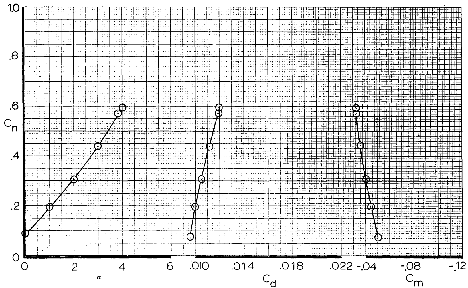
Figure A7 . - Airfoil force data for M = 0.74 , R_N = 11 \times 10^6 , X/C_T = \text{Free}
