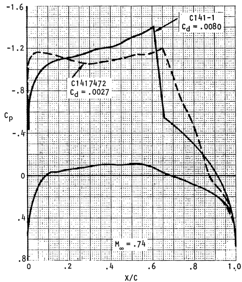
Figure 3. Airfoil C141H7472 inviscid design pressures ( \alpha = 2^\circ ).
