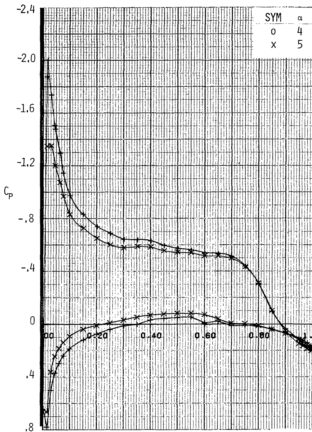
Figure A15.- Airfoil Pressure Distribution for M = 0.55 , R_N = 11 \times 10^6 , X/C_T = \text{Free}
