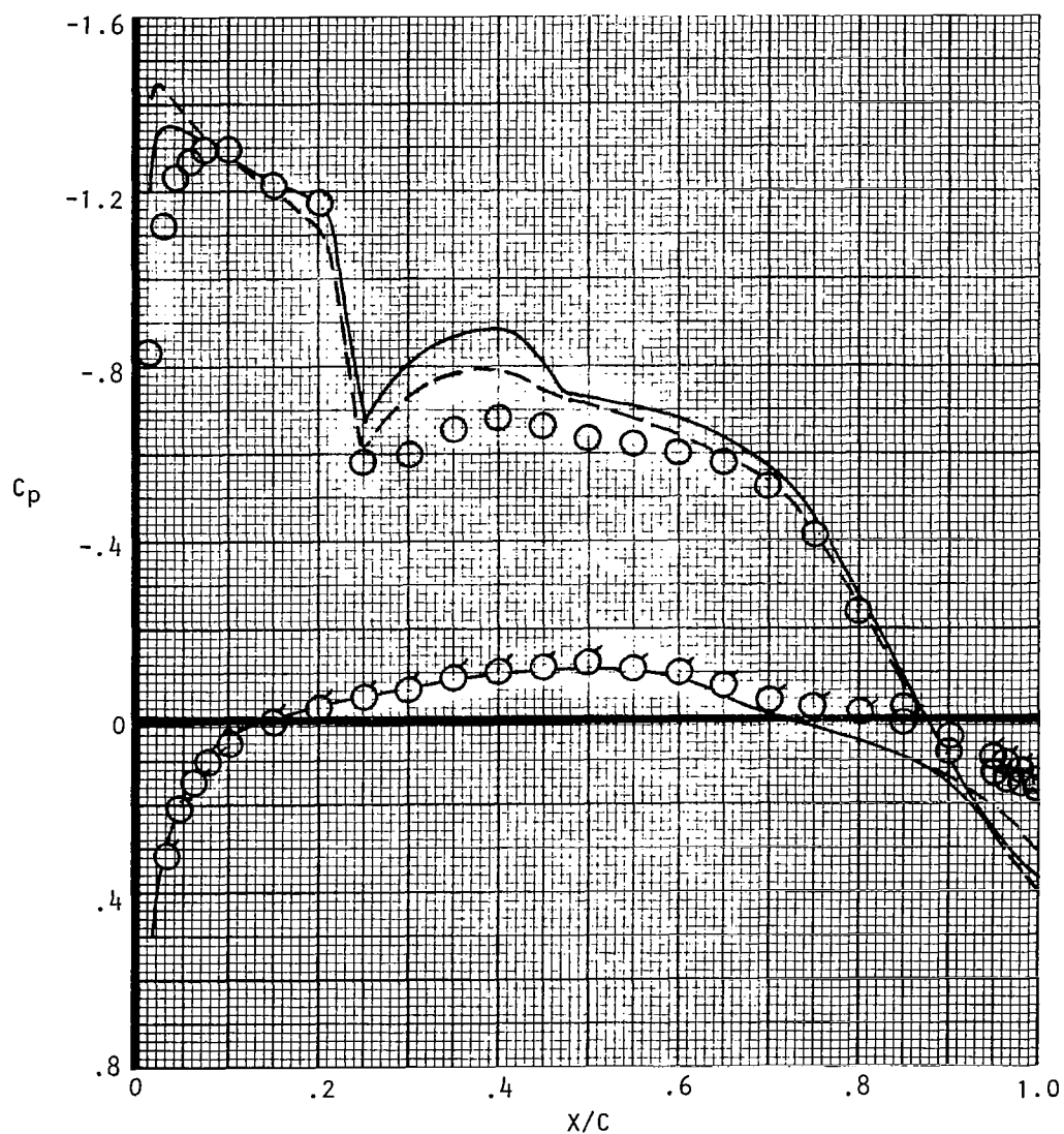
Figure 20. Airfoil C141H7472 theoretical and experimental pressure match.
