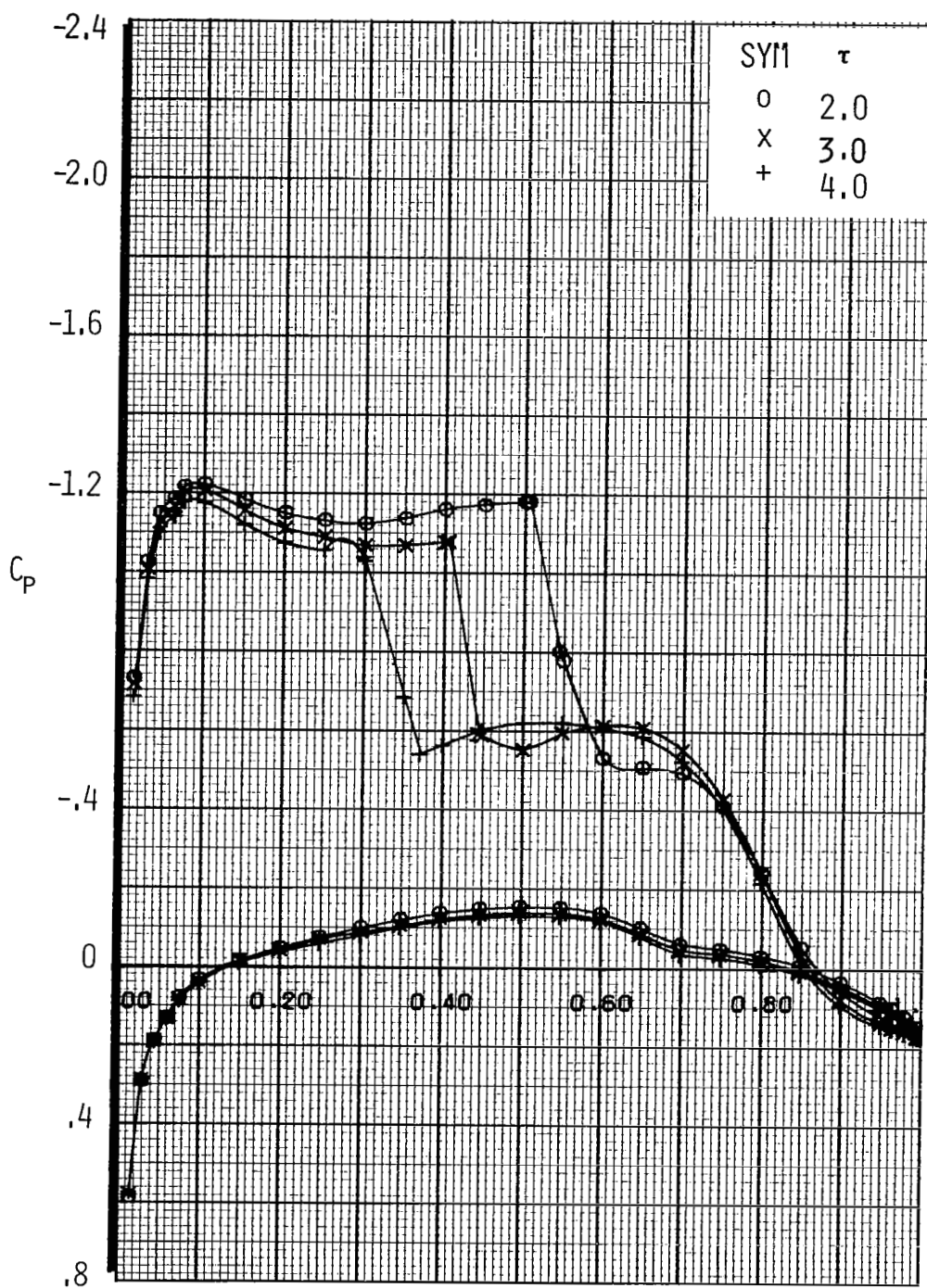
Figure A37.- Effect of Wind Tunnel Wall Porosity on Airfoil Pressure Distribution, M = .74 , R_N = 11 \times 10^6 , \alpha = 3.85^\circ .
