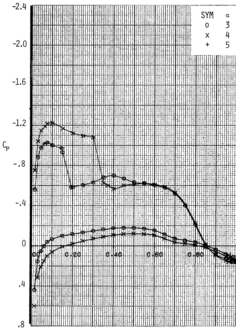
Figure A25.- Airfoil Pressure Distribution for M = 0.74 , R_N = 11 \times 10^6 , X/C_T = \text{Free}
