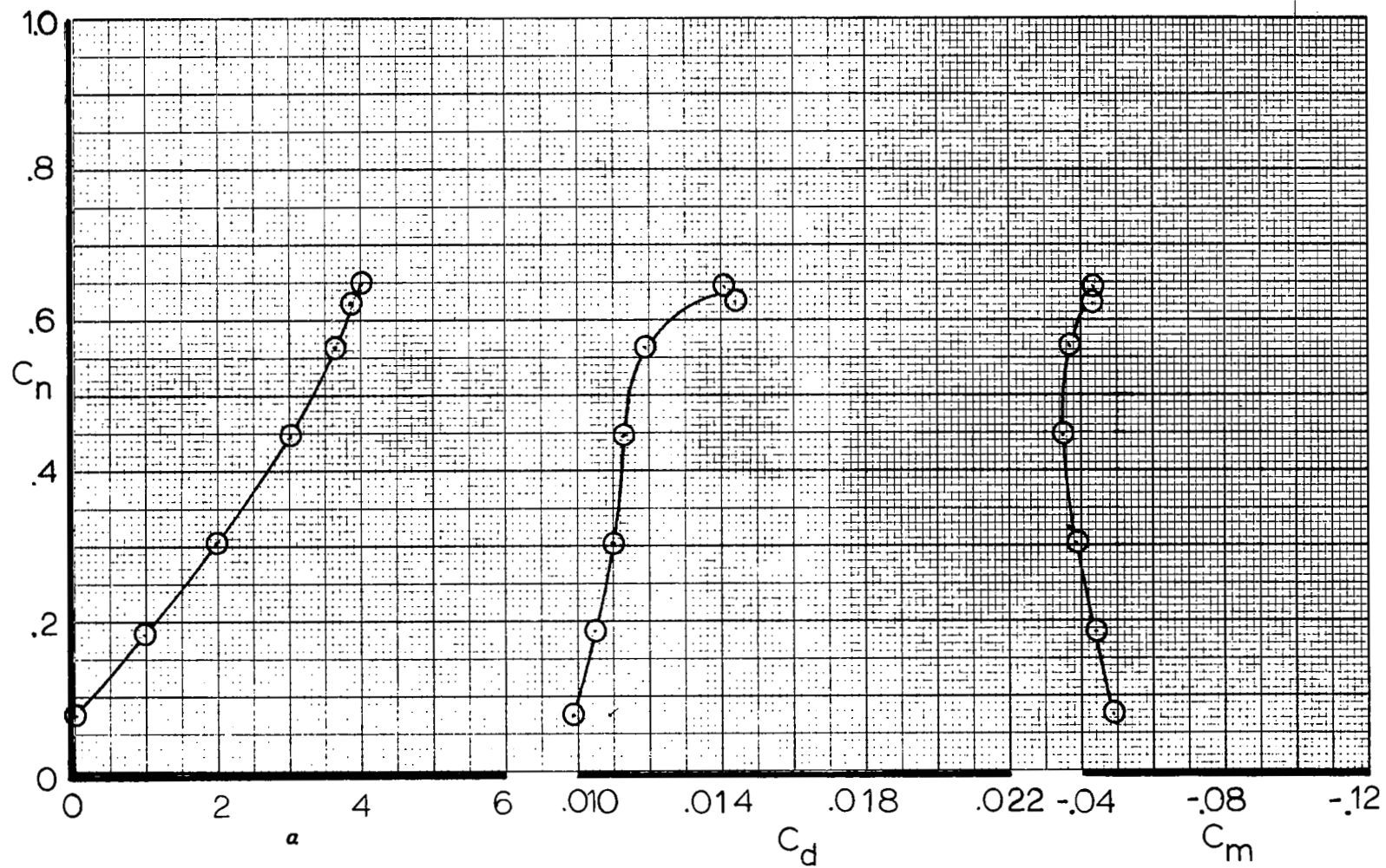
Figure A8 . - Airfoil force data for M=0.76 , R_N=11 \times 10^6 , X/C_T = \text{Free}
