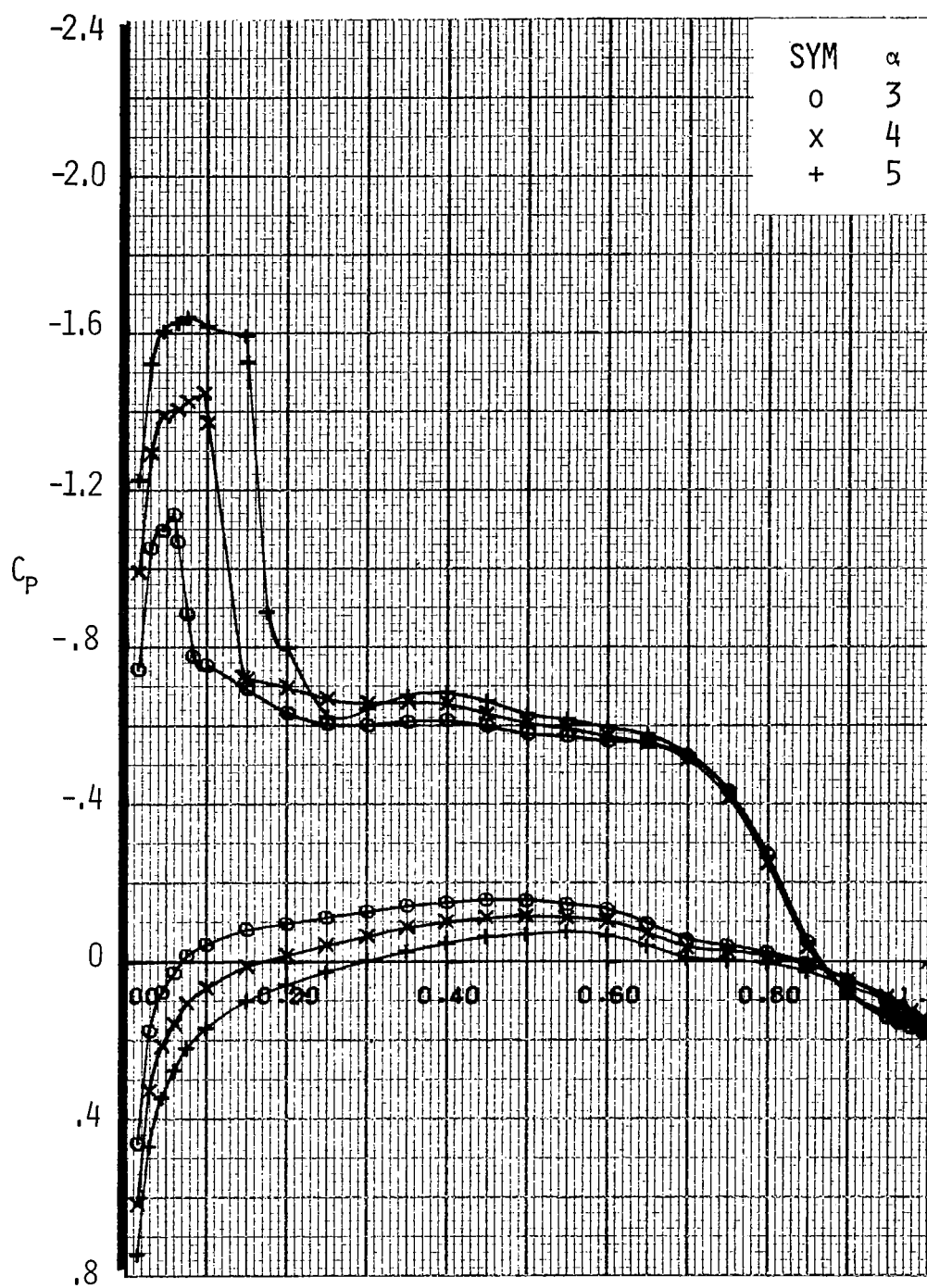
Figure A21.- Airfoil Pressure Distribution for M = 0.68 , R_N = 11 \times 10^6 , X/C_T = \text{Free}
