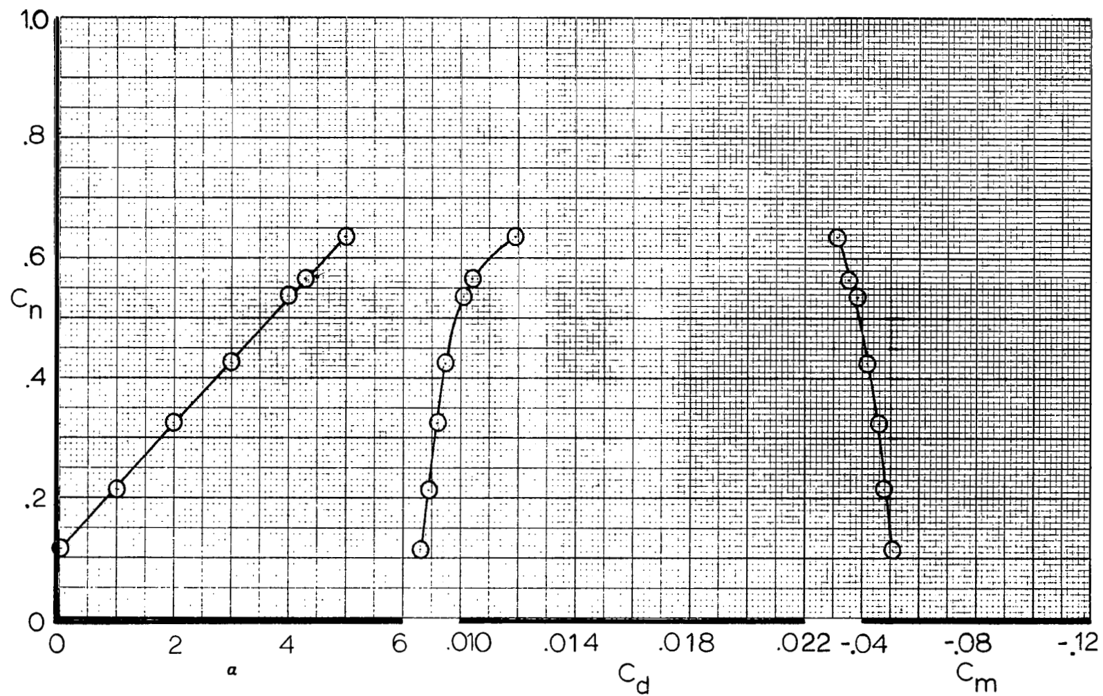
Figure A4. - Airfoil force data for M=0.64 , R_N=11 \times 10^6 , X/C_T = \text{Free}
