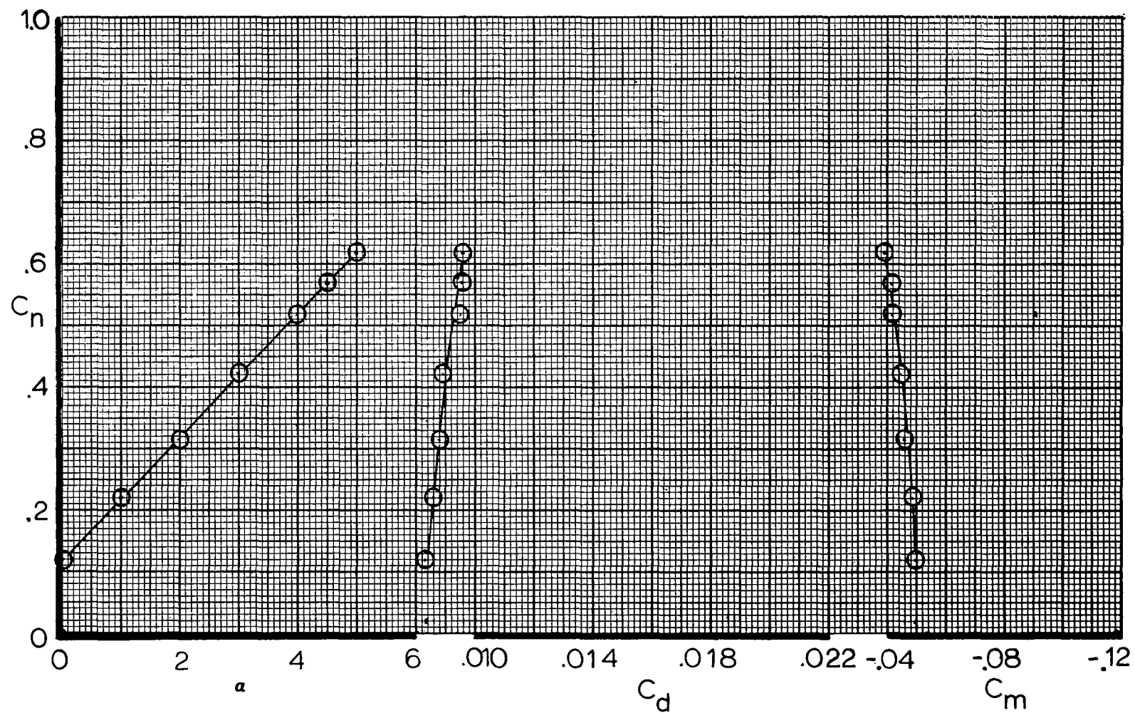
Figure A2 . - Airfoil force data for M=0.55 , R_N=11 \times 10^6 , X/C_T=Free
