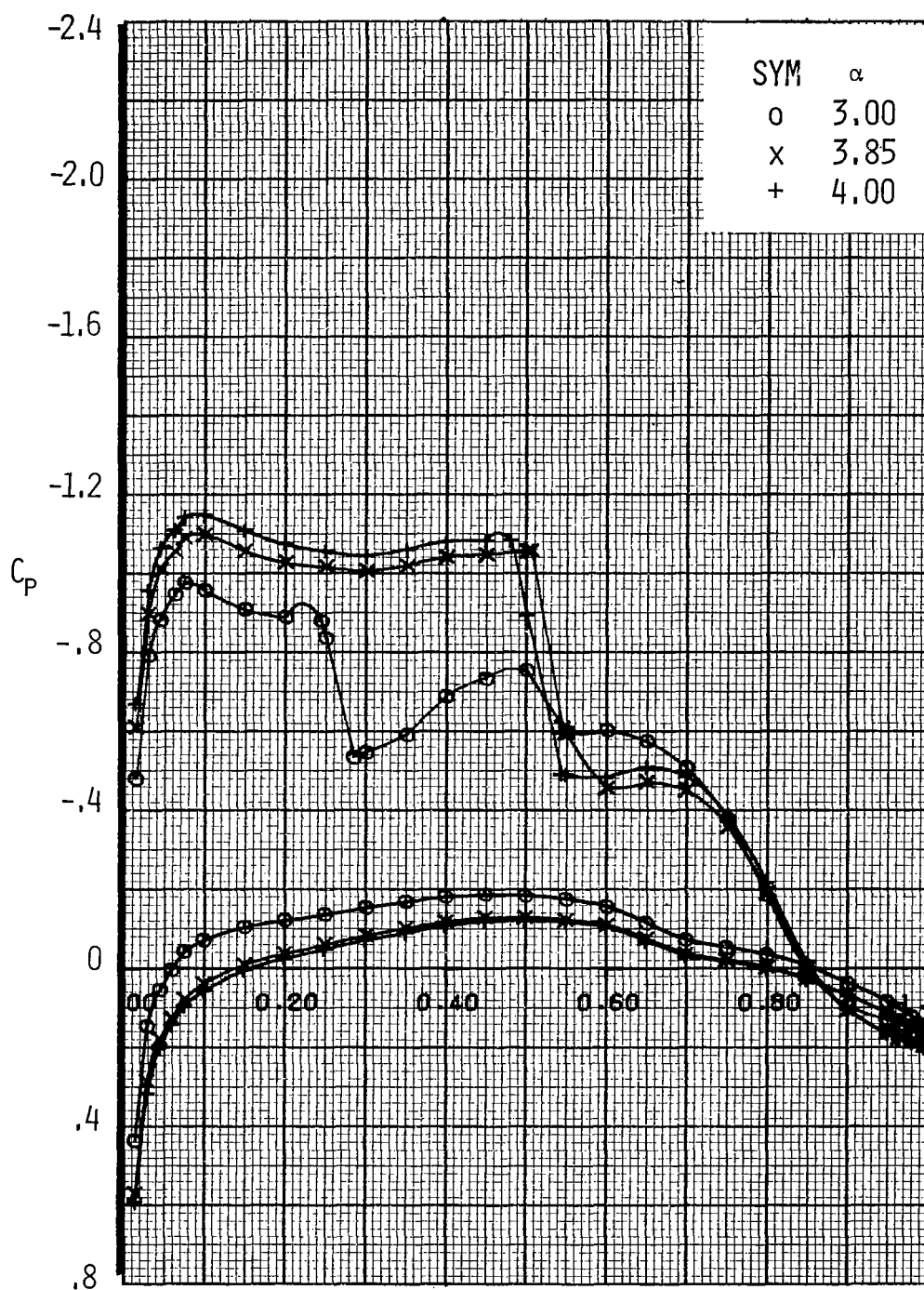
Figure A27.- Airfoil Pressure Distribution for M = 0.76 , R_N = 11 \times 10^6 , X/C_T = \text{Free}
