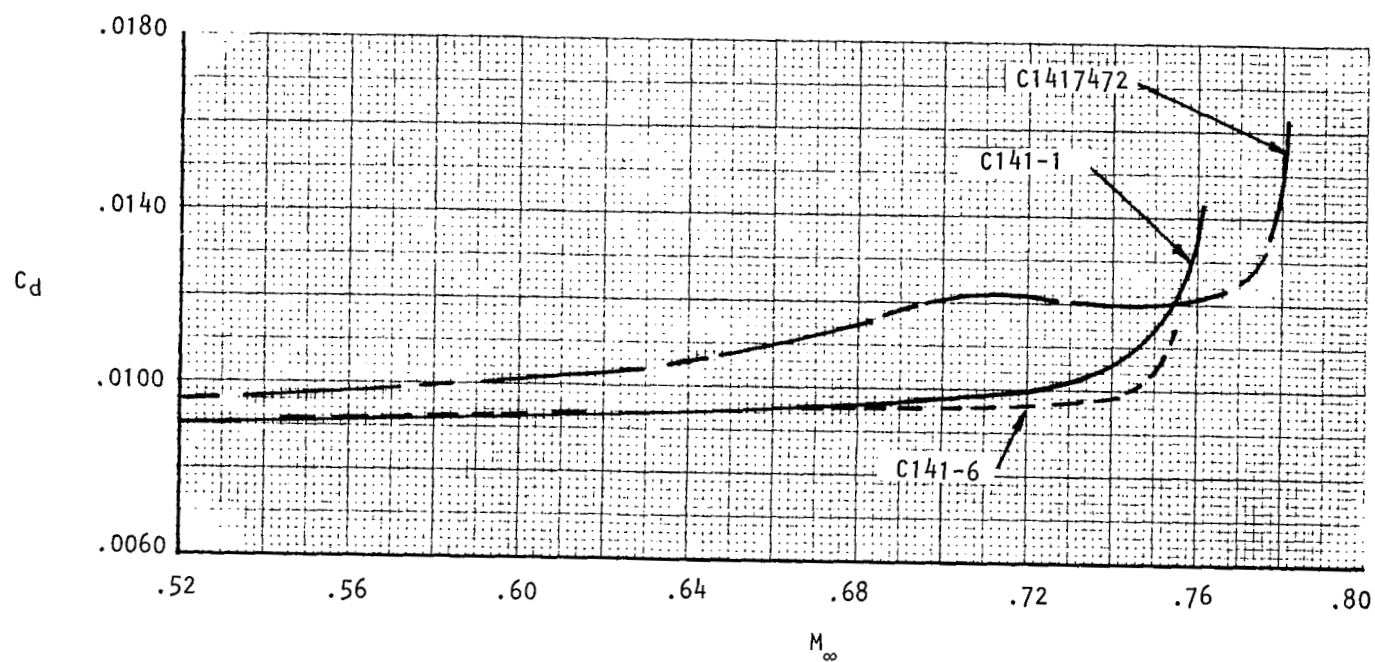
Figure 11. Comparison of measured airfoil performances at C_n = 0.57 , R_N = 11 \times 10^6 .
