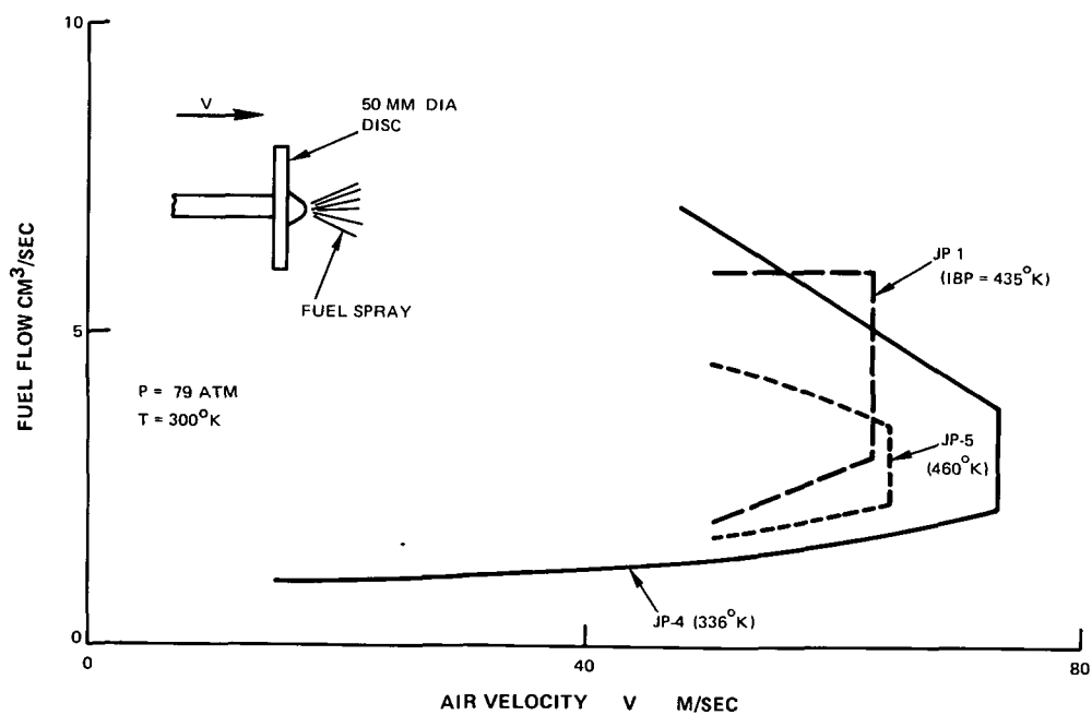
Figure 4-15 Effect of Fuel Volatility on Ignition With Buff Body Flameholder
