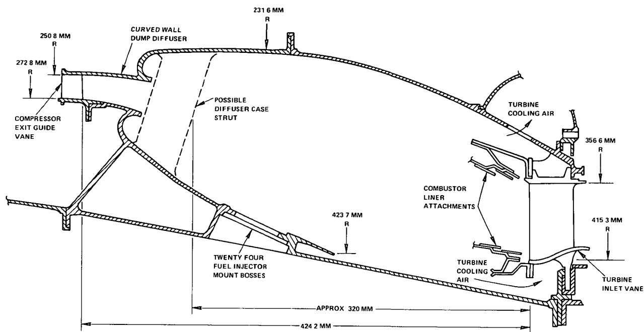
Figure 3-2 Combustor Section of Energy Efficient Engine
