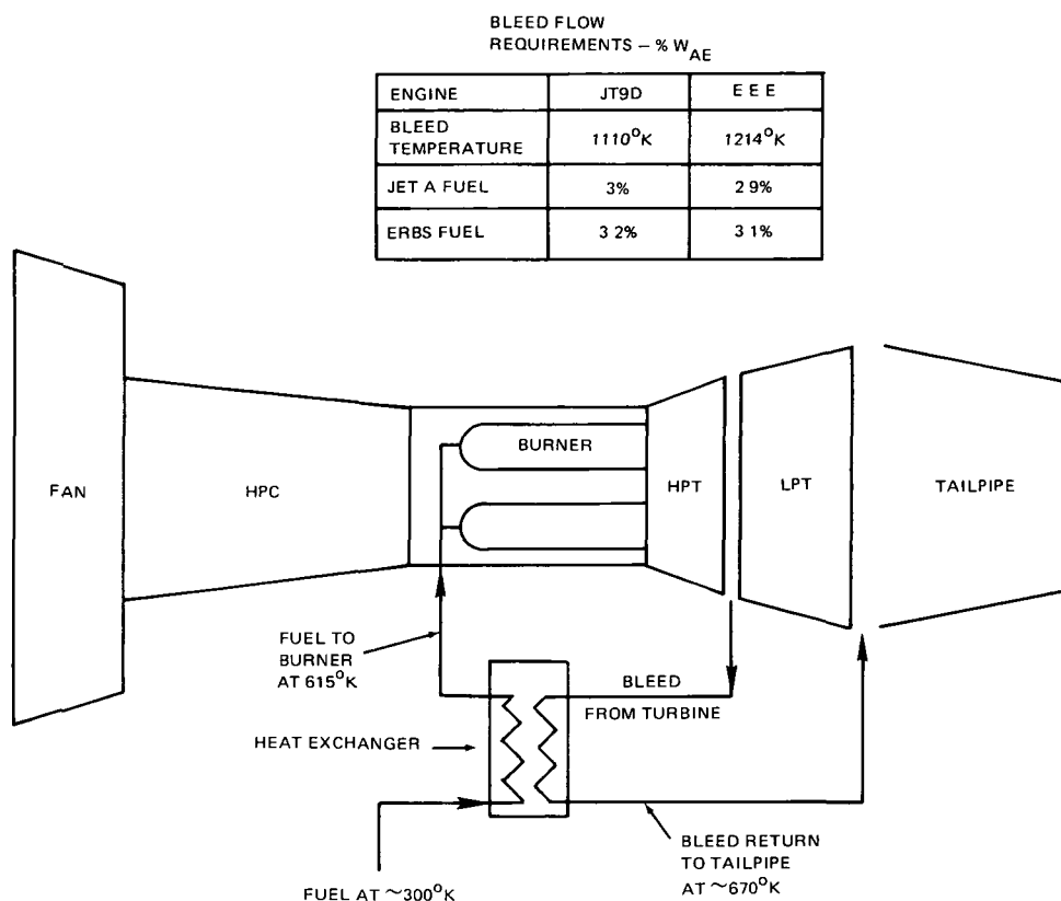
Figure 4-23 External Fuel Preheating With Low Turbine Bypass Flow
