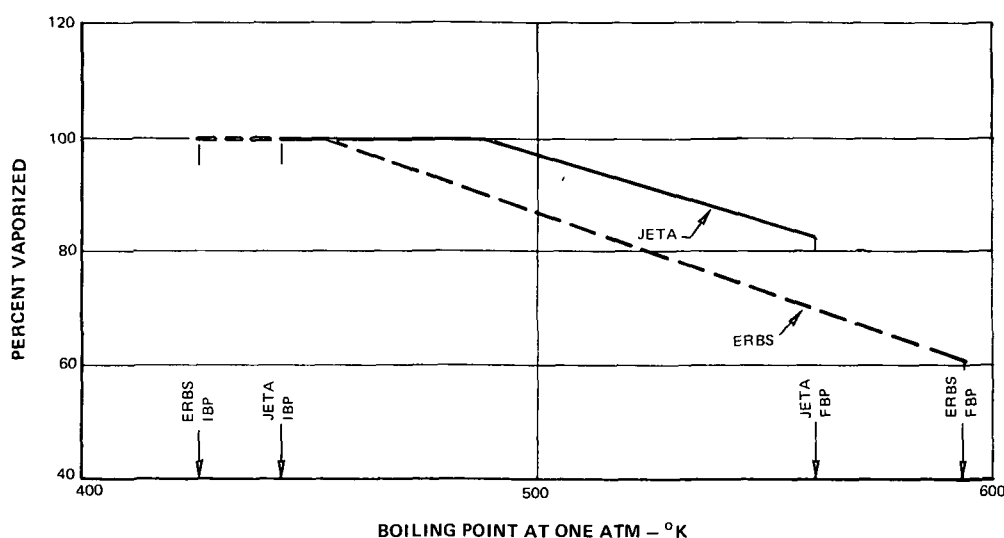
Figure 4-26 Approximate Vaporization Profile at Discharge From a Premixing Passage
