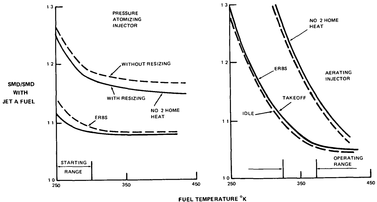
Figure 4-3 Effect of Fuel Composition on Atomization
