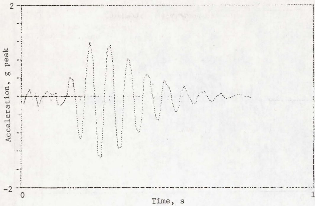
Figure 5. - Measured transient at location A--test condition 1.
