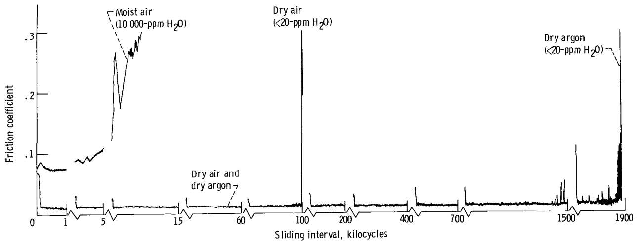
Figure 3. - Friction coefficient as a function of sliding interval for rubbed \text{MoS}_2 films applied to sanded 440C HT steel disks and evaluated in three atmospheres. Rider material, 440C HT steel; sliding speed, 2.6 meters per second (1000 rpm); load, 1 kilogram; temperature, 25^\circ\text{C} .
