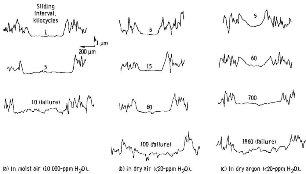
Figure 4. - Surface profiles of wear tracks on rubbed MoS 2 films applied to sanded 440C HT steel disks and evaluated in three atmospheres.
