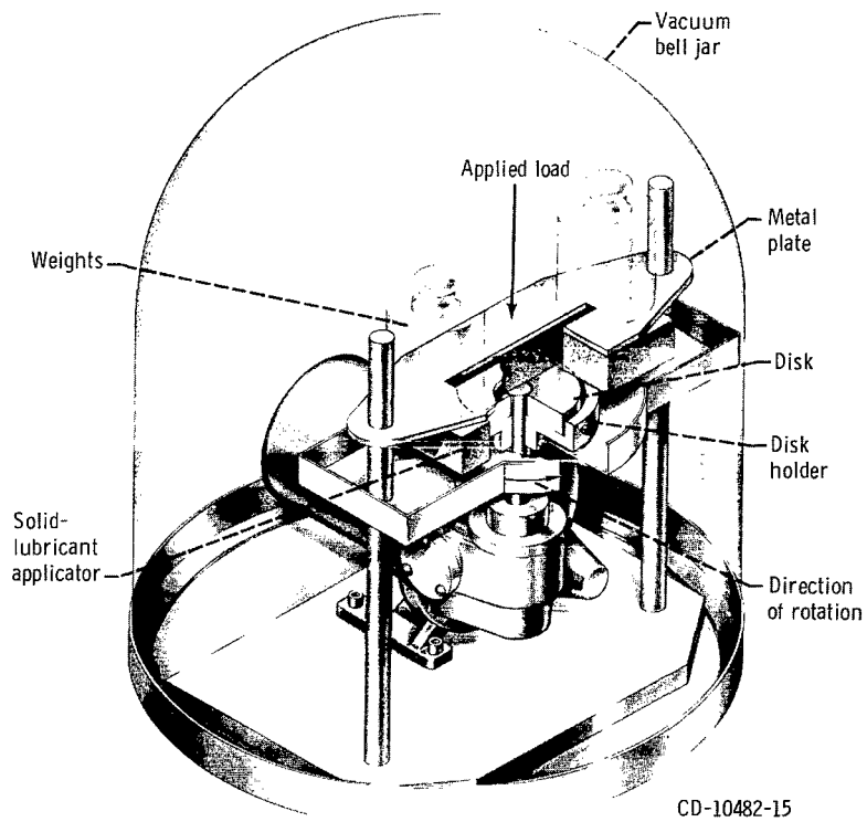
Figure 2. - Apparatus used for applying molybdenum disulfide films.
