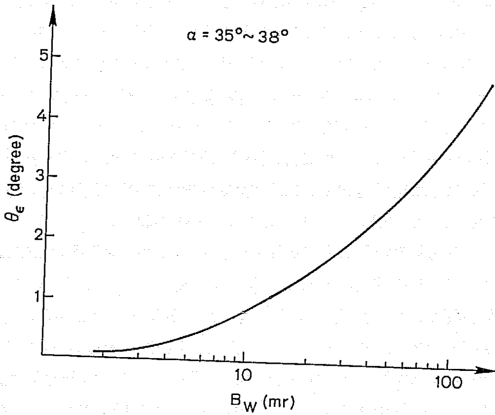
Fig. B.5. THE ANGLE \theta_\epsilon VS WAVE AMPLITUDE, ASSUMING ELECTRON PITCH ANGLE TO BE ABOUT 35^\circ TO 38^\circ . This angle becomes greater than 4^\circ when the wave is stronger than 100 my.
