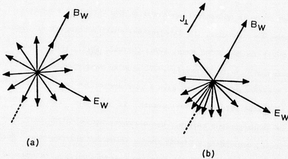
Fig. B.11. ILLUSTRATION OF PHASE BUNCHING MECHANISM. See text.
