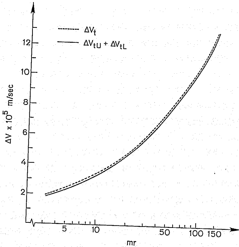
Fig. B.8. THE CALCULATED TRAPPING WIDTH \Delta V_t BY EQ. (B.10) AND THE VALUE OF \Delta V_{tU} + \Delta V_{tL} VS WAVE INTENSITY.
