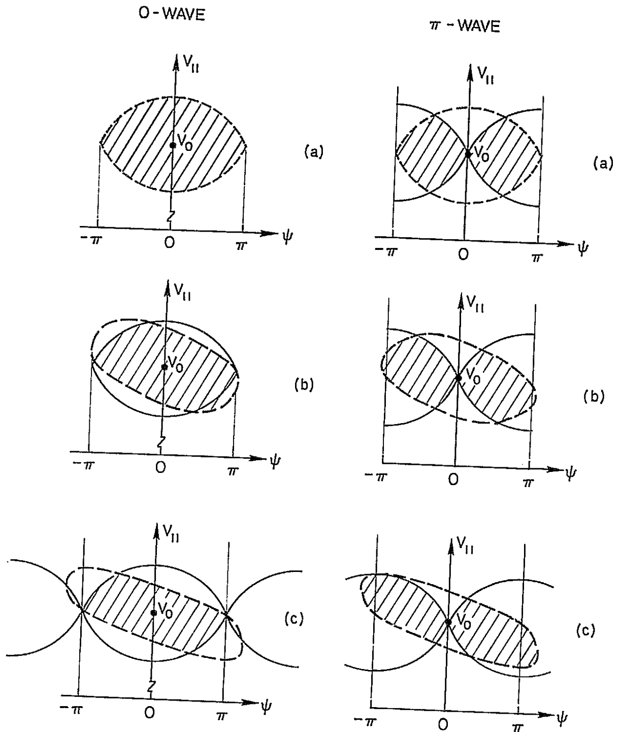
Fig. 3.8. DEFORMATION OF THE TRAPPING DOMAIN DURING THE GAPS. The gap size equals (a) 0 msec, (b) 10 msec, and (c) 20 msec. Electrons in the shaded areas are those which were trapped by the pre-gap section and are still trapped by the post-gap section of the signal. A homogeneous model is used. The corresponding frequency range of the trapping range in V_{||} is assumed to be 50 Hz.
