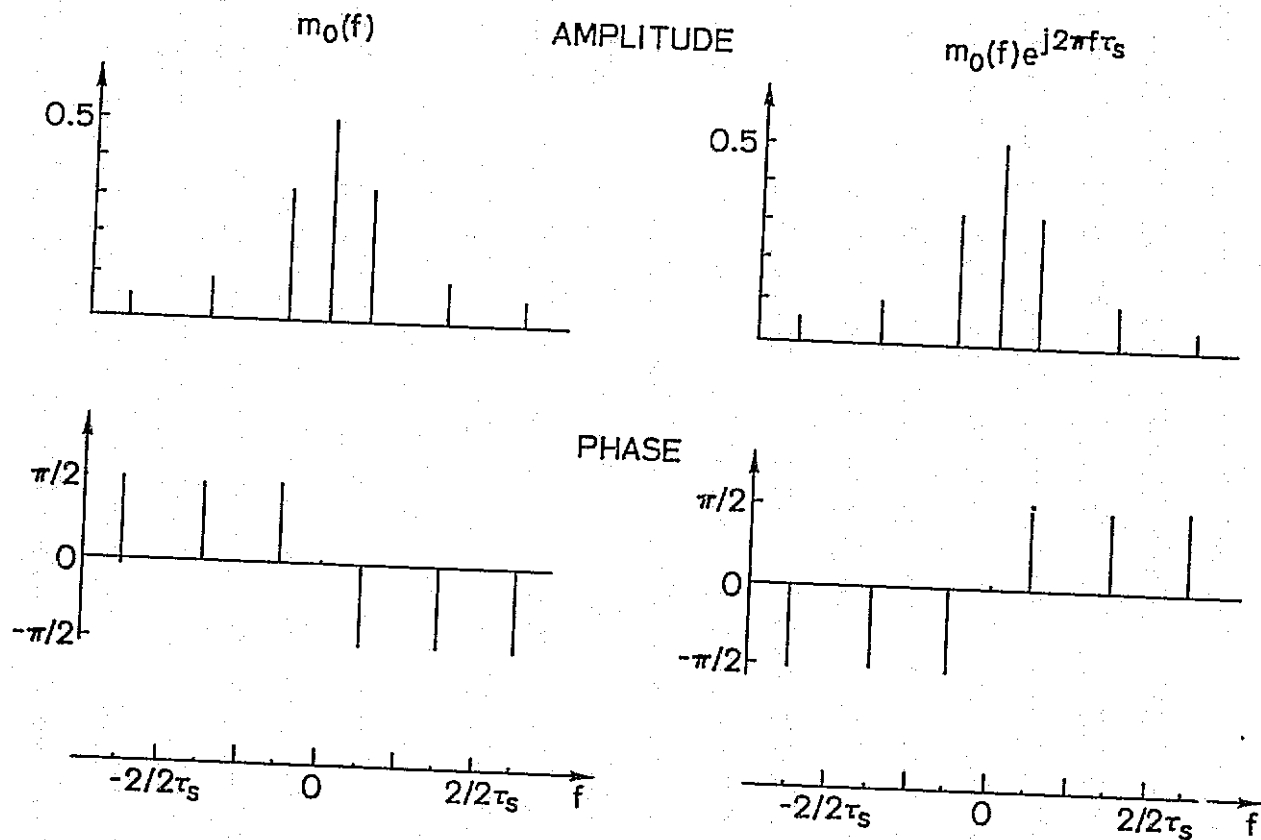
Fig. C.2. THE CORRESPONDING SPECTRUM m_0(f) OF M_0(t) AND m_0(f)e^{i2\pi f\tau_s} IN THE FREQUENCY DOMAIN.
