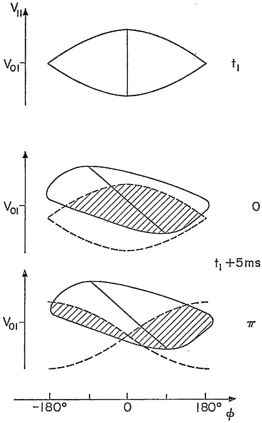
Fig. 3.9. DEFORMATION OF THE TRAPPING DOMAIN DURING A 10 msec GAP IN AN INHOMOGENEOUS MODEL. The transit time of an electron to cross the gap requires about 5 ms because the electron and the wave travel in opposite directions.
