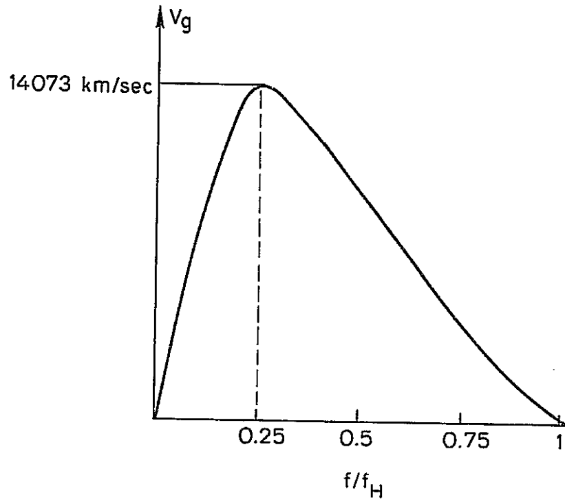
Fig. 2.4. A PLOT OF GROUP VELOCITY VS FREQUENCY OF A WM SIGNAL PROPAGATING IN A HOMOGENEOUS MAGNETO-PLASMA IN WHICH f_N = 180 \text{ kHz} AND f_H = 13 \text{ kHz} .
