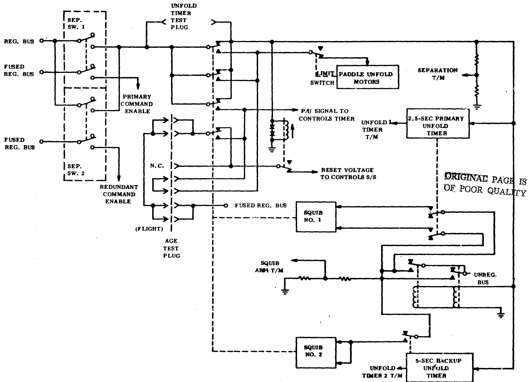
Figure 12-3. Separation and Unfold Subsystem Functional Block Diagram
