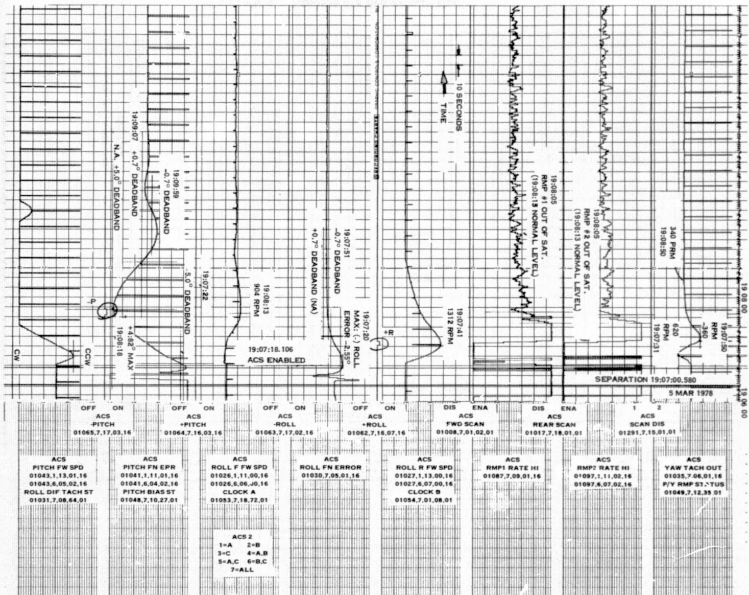
Figure 6-5. Landsat 3's Sun Acquisition
