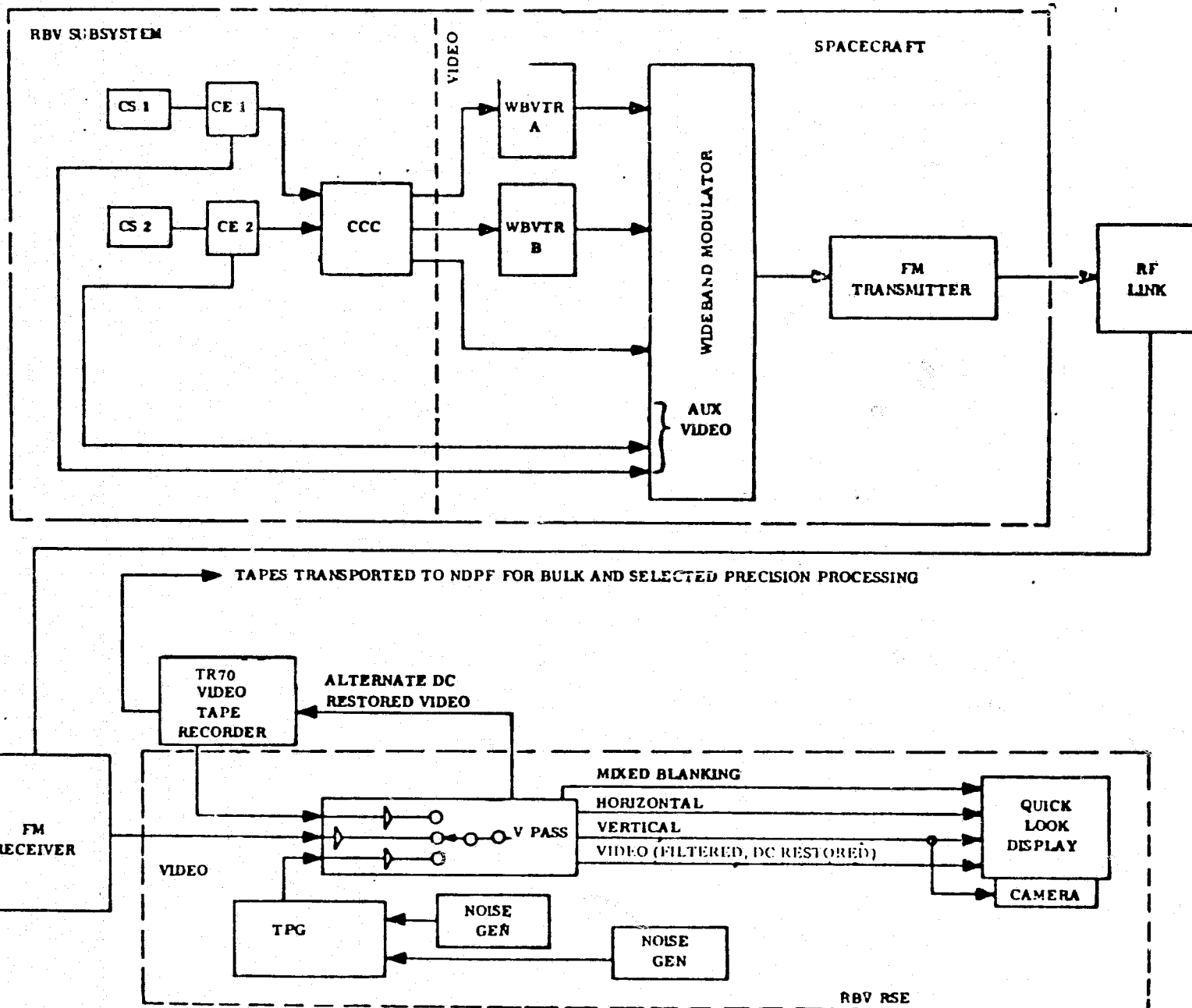
Figure 19-1. Return Beam Vidicon System Functional Block Diagram
