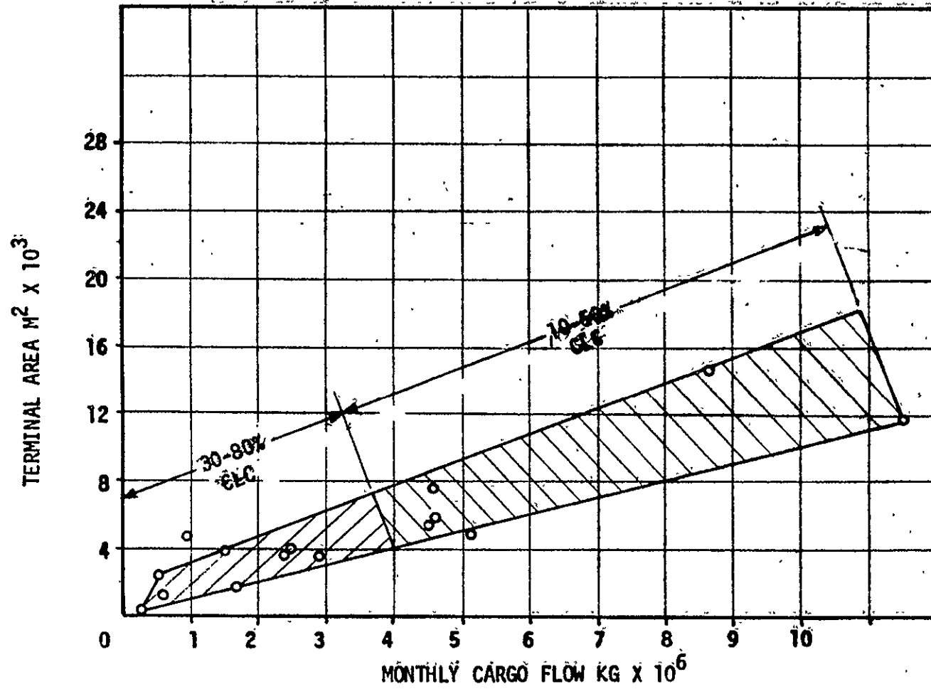
Figure 3-17. Monthly Cargo Flow per Terminal Area (CLC)
