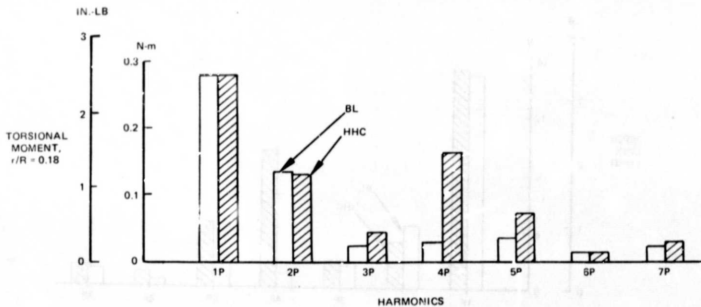
Figure 10. Harmonic Decomposition of Blade Torsional Moment (Ref. 10)
