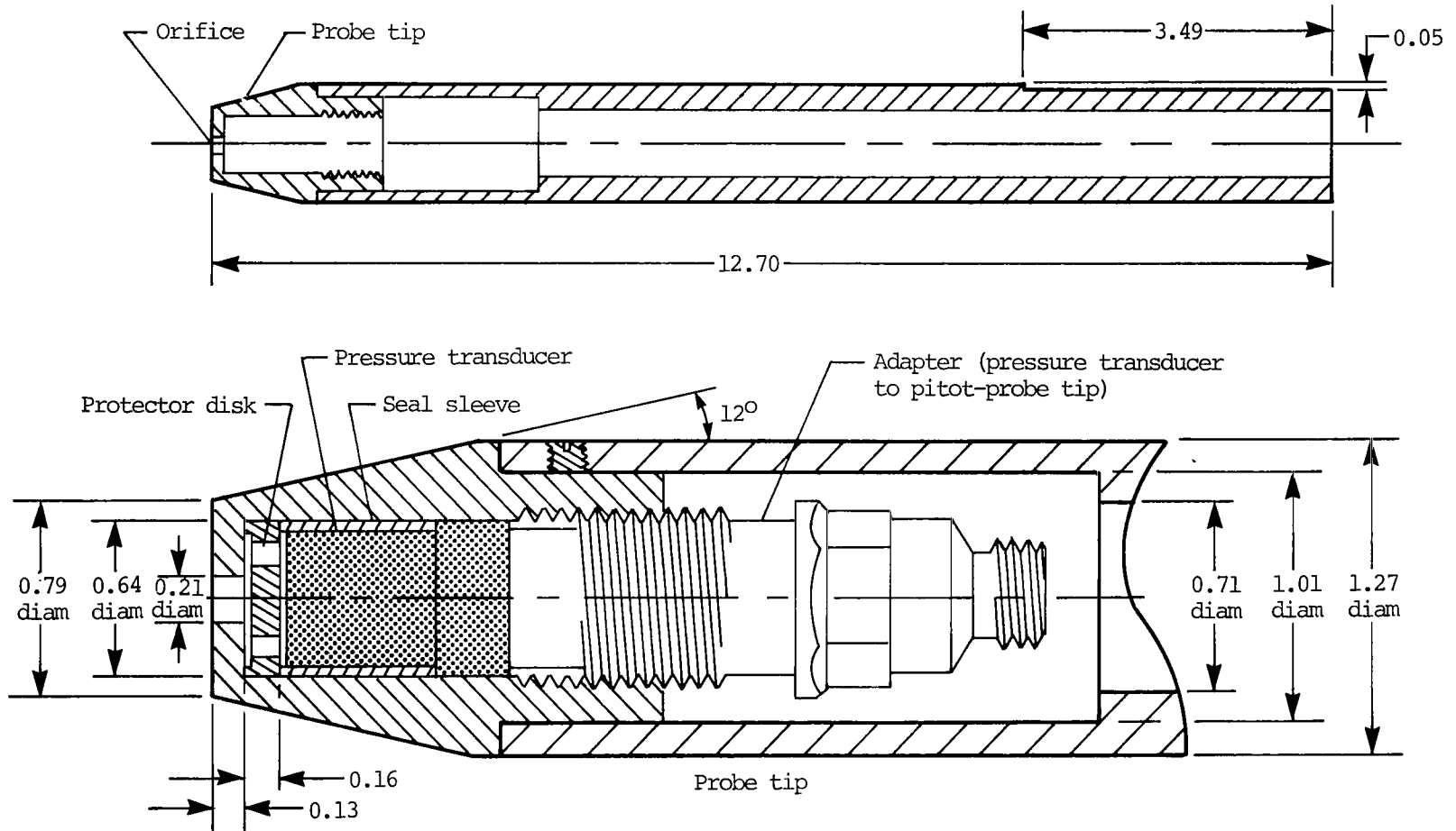
(b) Pitot-pressure probe.
