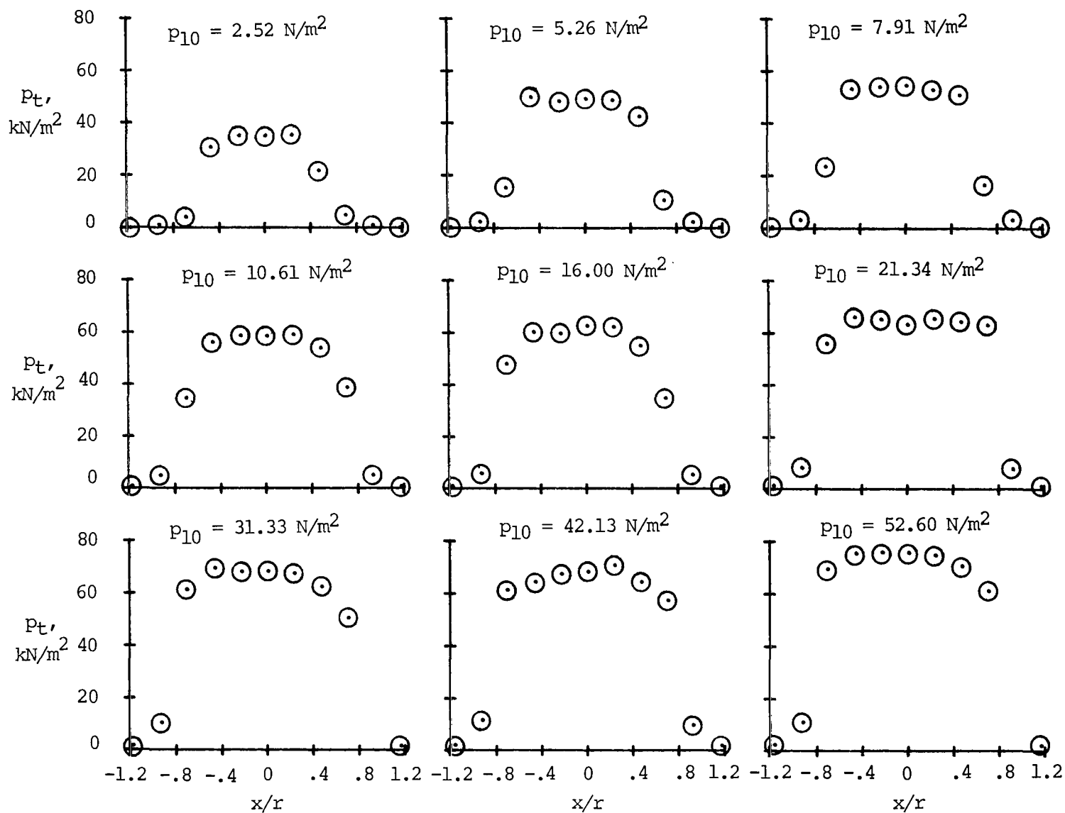
Figure 15.- Effect of quiescent acceleration-gas pressure on pitot-pressure profile. z_e = 5.64 \text{ cm} ; t = 150 \text{ } \mu\text{s} ; p_1 \approx 3.45 \text{ kN/m}^2 .
