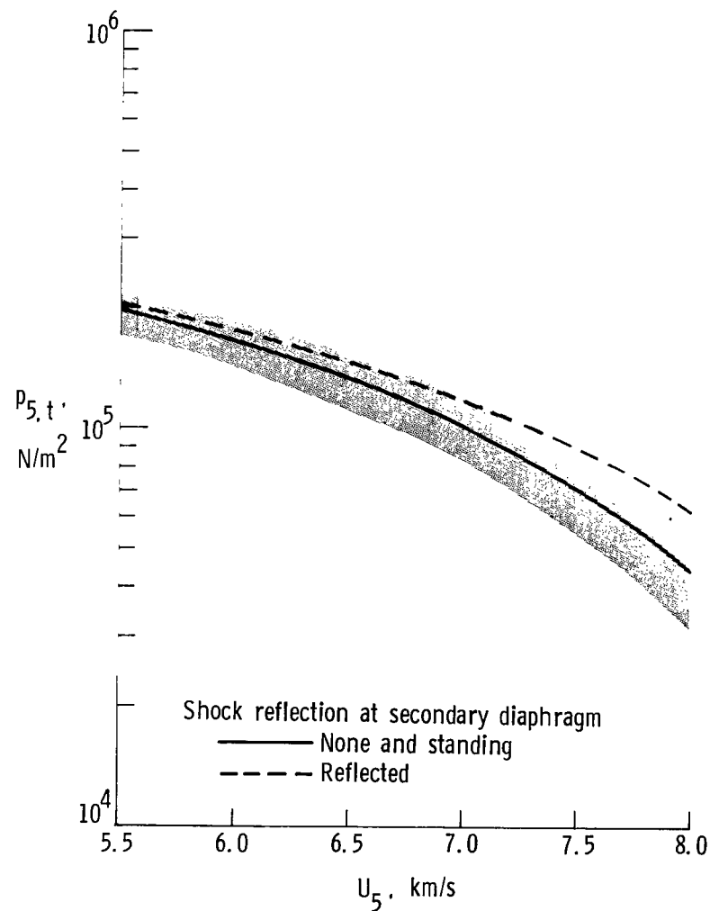
(b) Pitot pressure.
