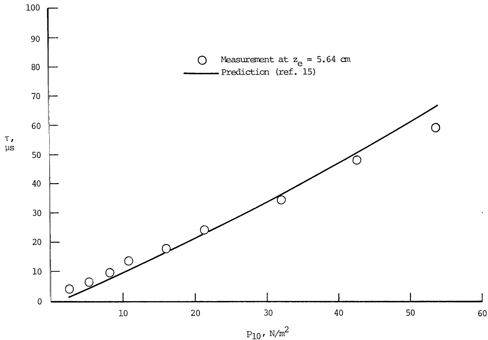
Figure 7.- Time interval between incident shock and acceleration-gas/test-gas interface as a function of quiescent acceleration-gas pressure. p_1 \approx 3.45 \text{ kN/m}^2 .
