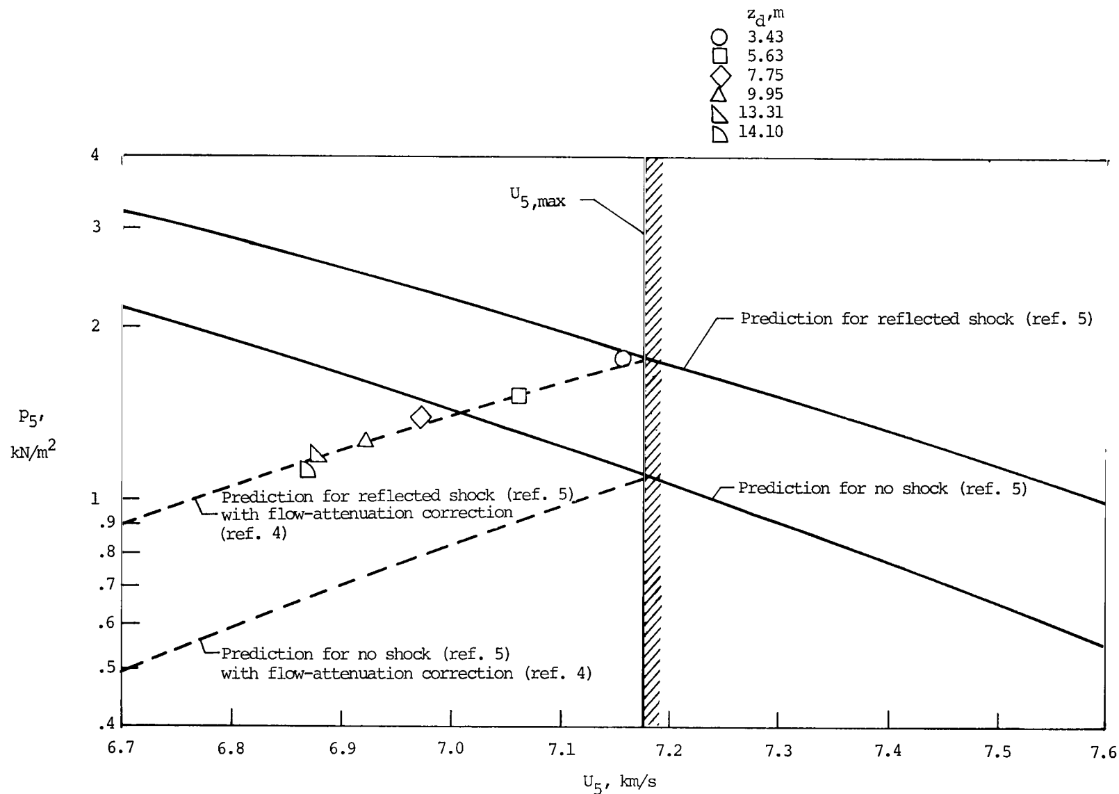
Figure 14.- Comparison of measured tube-wall pressure at various distances downstream of secondary diaphragm with predictions. p_1 \approx 3.45 kN/m^2 ; p_{10} = 16.00 N/m^2 .
