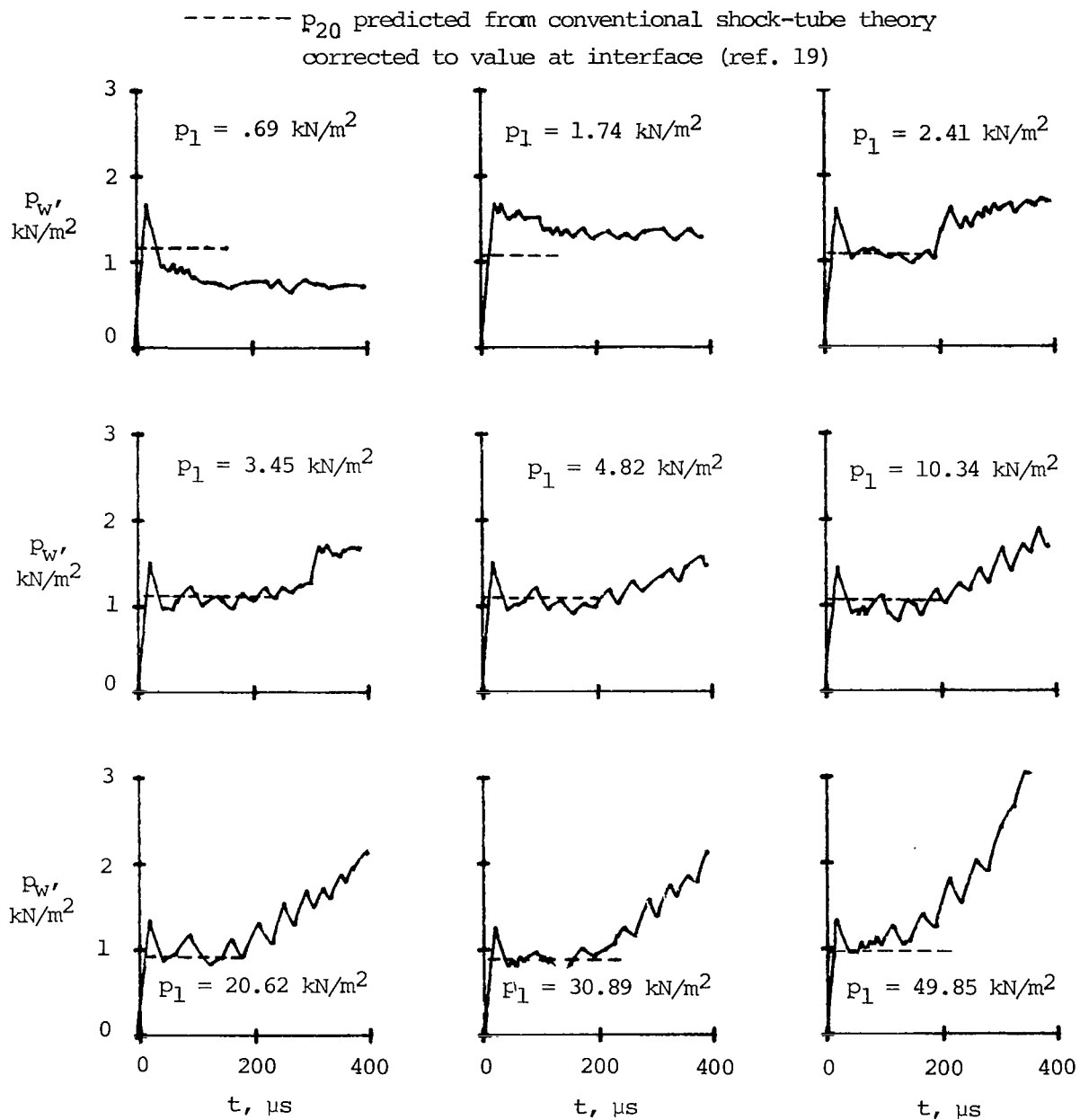
Figure 23.- Effect of quiescent test-gas pressure on time history of tube-wall pressure 2.54 cm upstream of tube exit. P_{10} \approx 16.00 \text{ N/m}^2 .
