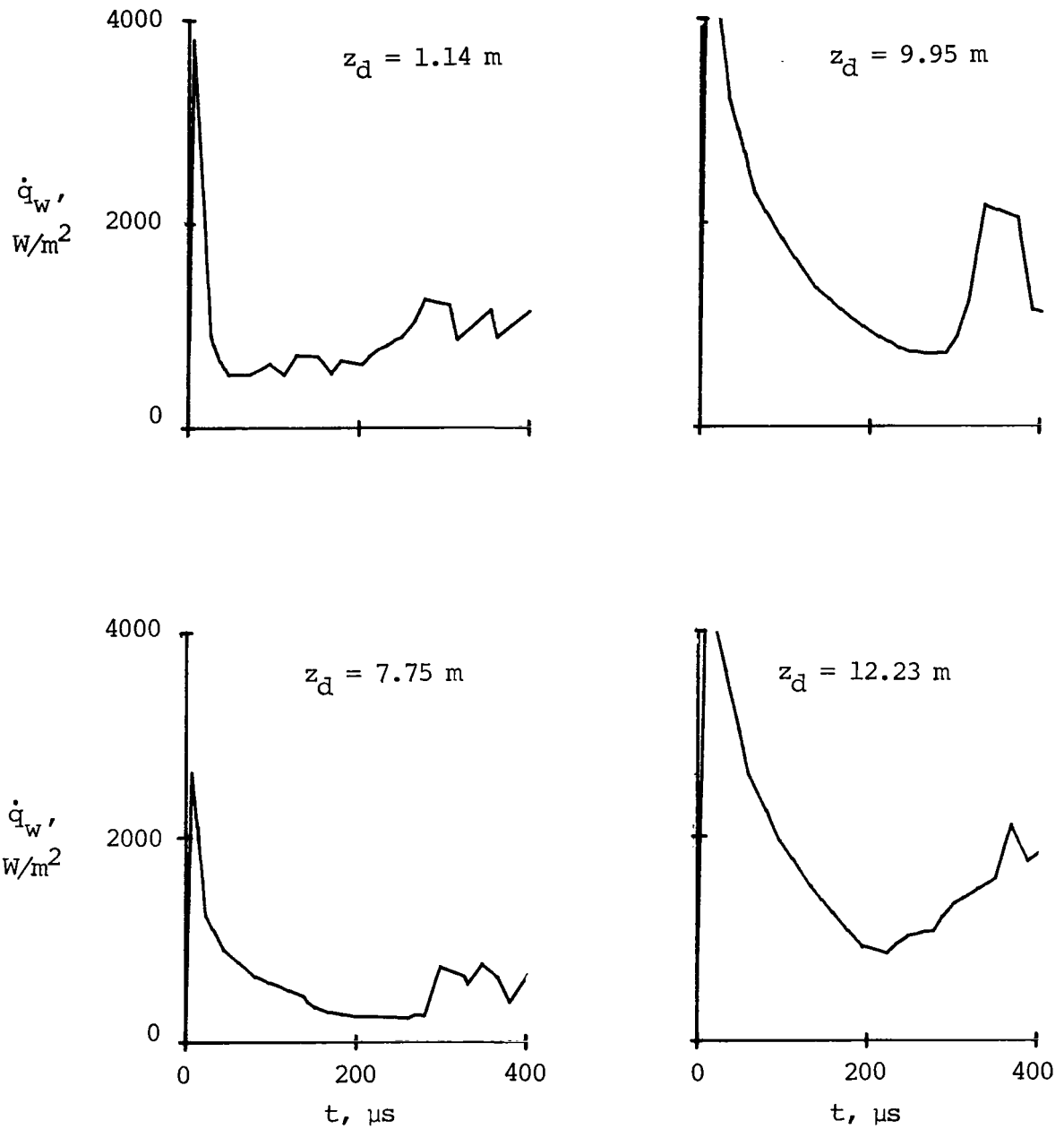
Figure 11.- Time history of tube-wall heat transfer at various distances downstream of secondary diaphragm. p_1 \approx 3.45 \text{ kN/m}^2 ; p_{10} = 52.60 \text{ N/m}^2 . ( \dot{q}_w was obtained to illustrate trends only and should not be used quantitatively.)
