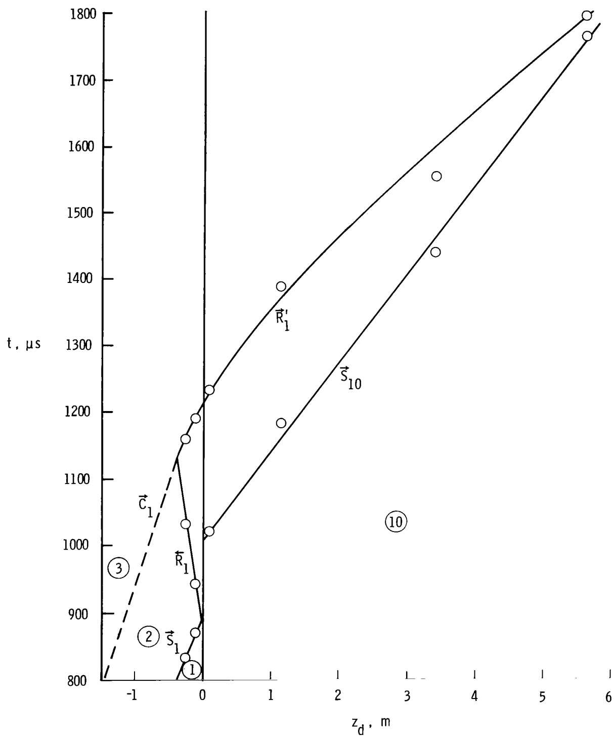
Figure 22.- Distance-time diagram showing refraction phenomenon of reflected shock in vicinity of secondary diaphragm. p_{10} \approx 16.00 \text{ N/m}^2 ; p_1 = 0.69 \text{ kN/m}^2 .
