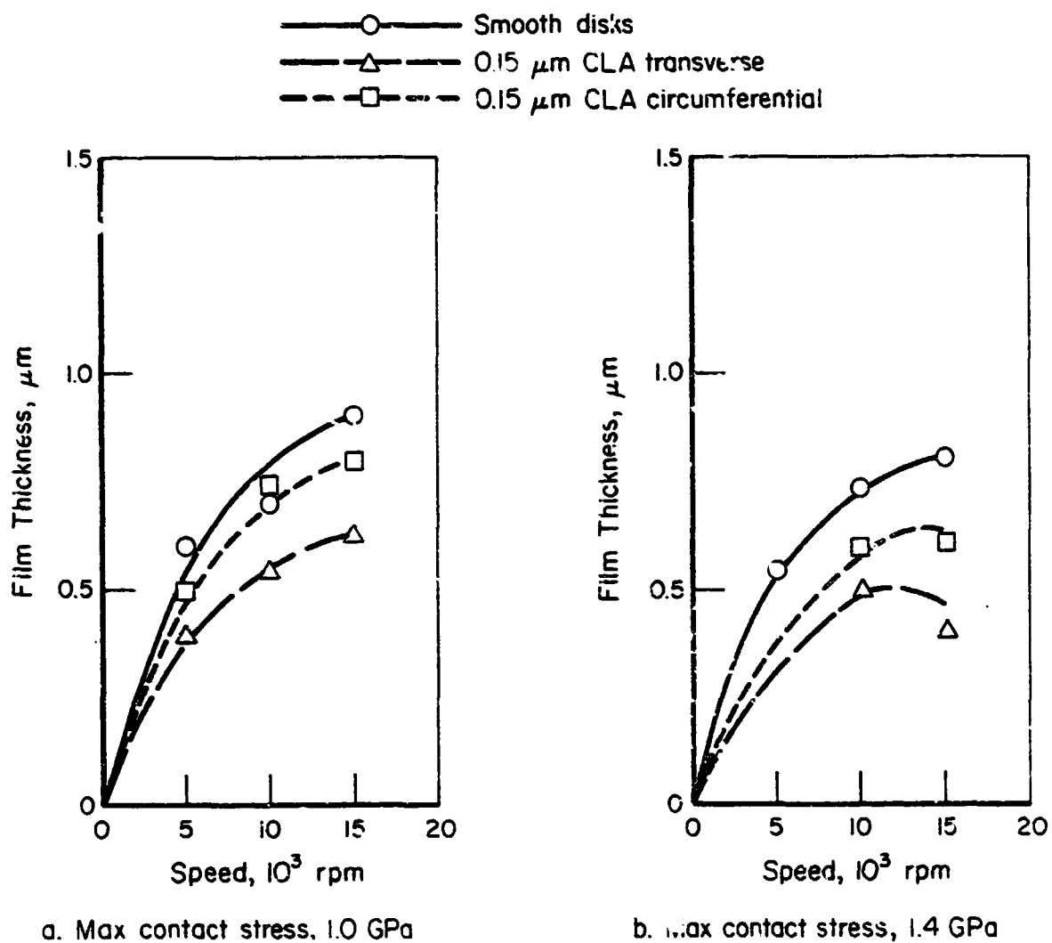
FIGURE 14. FILM THICKNESS AS A FUNCTION OF DISK SPEED FOR VARIOUS LEVELS OF SURFACE ROUGHNESS FOR XRM-177T AT 90 C
