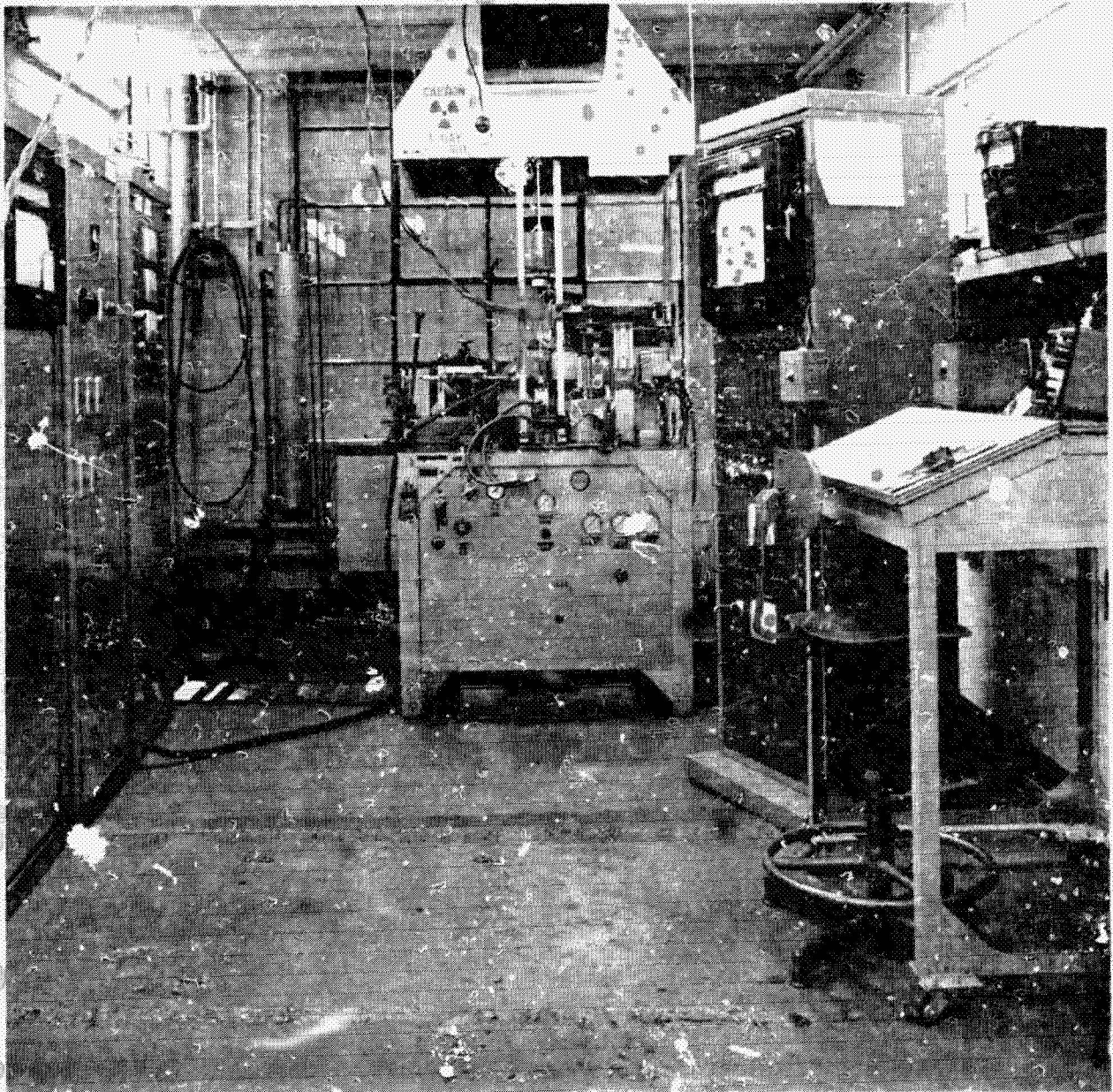
FIGURE 2. PHOTOGRAPH OF DIS U APPARATUS
