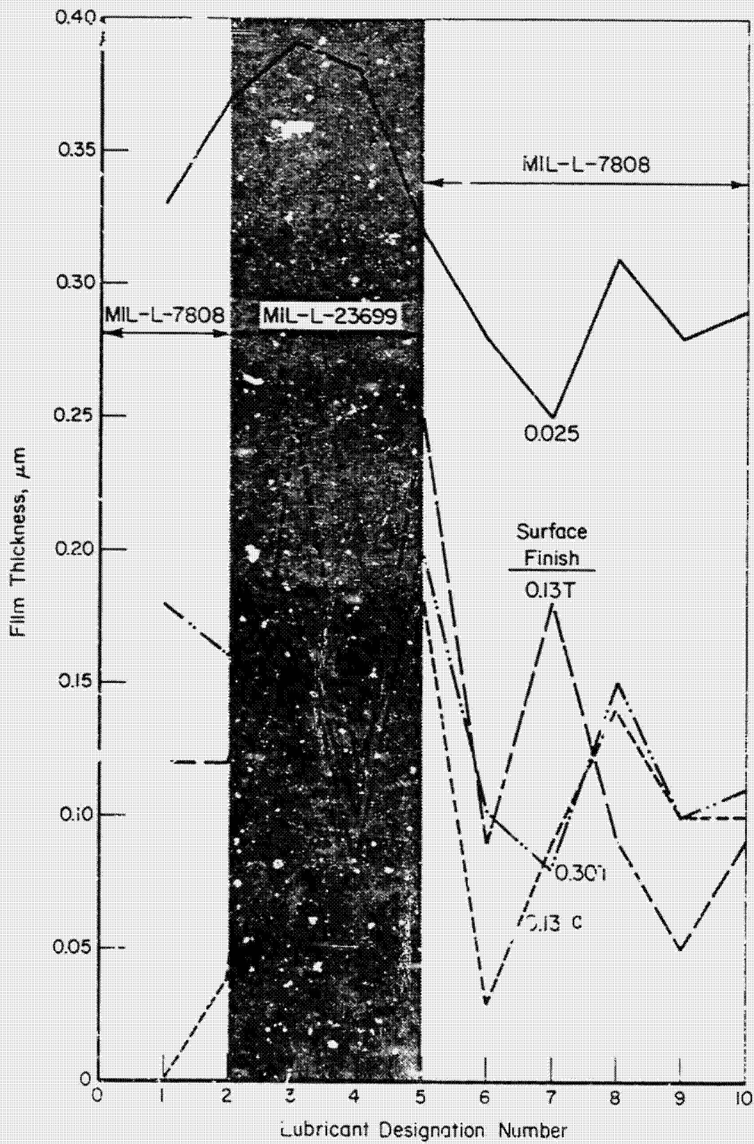
FIGURE 30. COMPARISON OF FILM THICKNESS FOR DIFFERENT SURFACE ROUGHNESS ON LOWER DISK
