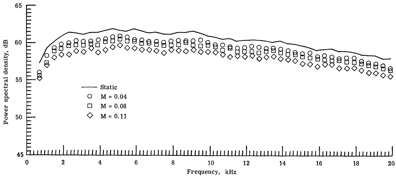
Figure 9.- Power spectral densities from free-jet test at 90° observer angle.
