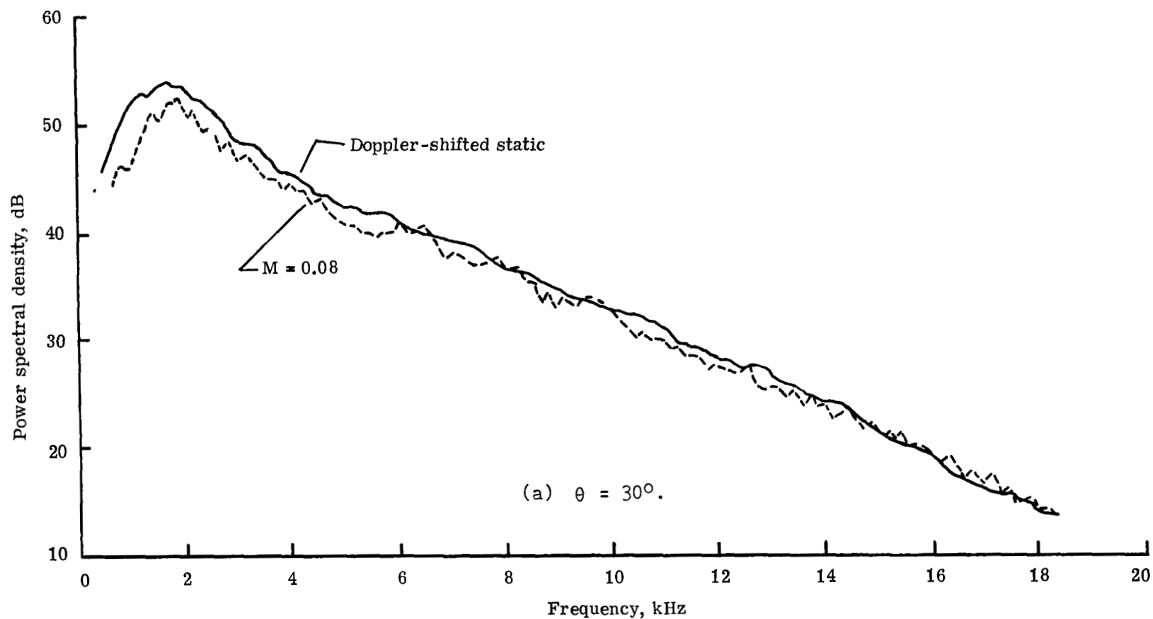
Figure 4.- Comparison of motion spectra with Doppler-shifted static spectra for M = 0.08 . (Moving vehicle tests.)
