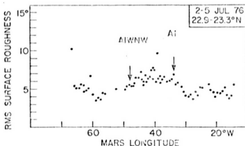
Fig. 7 - Surface roughness estimates over the Chryse region from 1976 spectra. "A1" was the original prime landing site, "A1WNW" was the final site.
