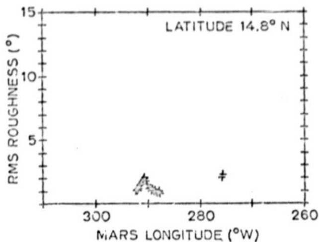
Fig. 3 - Surface roughness estimates in Syrtis Major from 1978 spectra. The apparent increase in roughness near 291^{\circ}\text{W} may be due to scattering by the ridge-like feature Arena Dorsum.
