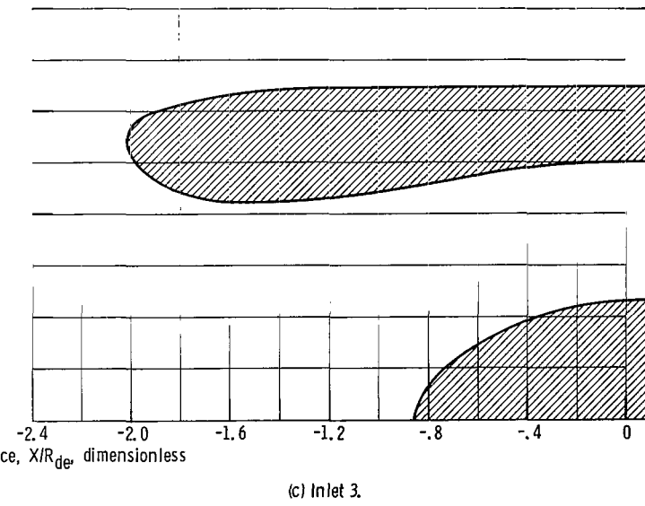
Figure 2. - Inlet geometry: variation of inlet contraction ratio. Cubic diffuser; maximum wall angle, 8.7^\circ ; lip major-to-minor axis ratio, 2.0; drag-divergence Mach number, 0.8; diffuser-exit-area to throat-area ratio, 1.10.
