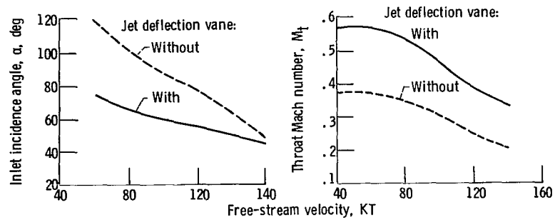
Figure 6. - Inlet operating requirements for tilt nacelle V/STOL aircraft.
