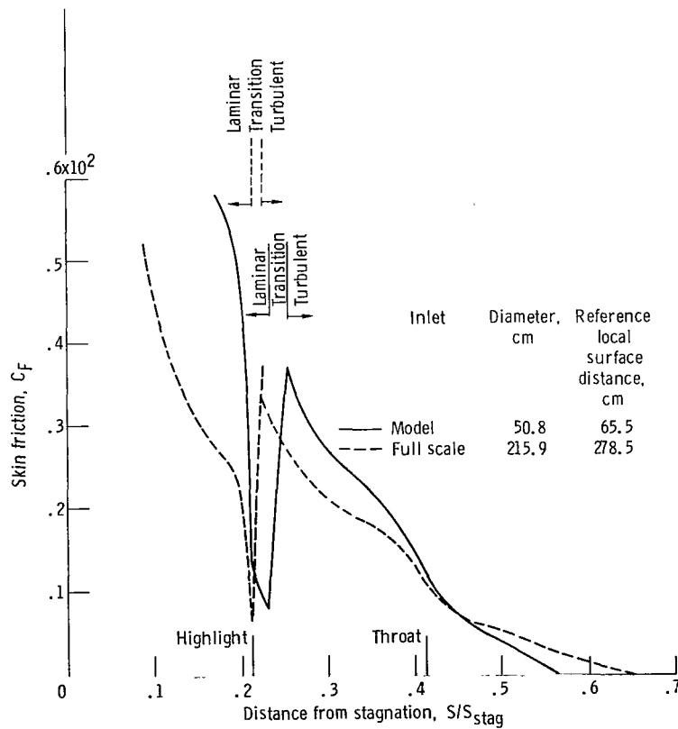
Figure 16. - Effect of scaling on skin friction for baseline inlet (inlet 1).
