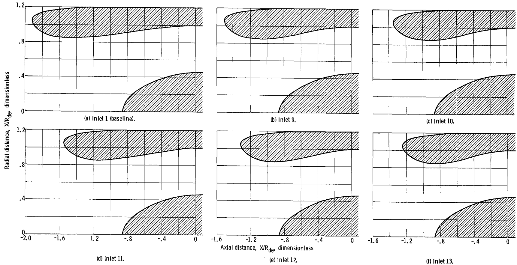
Figure 5. - Inlet geometry; variation of diffuser type and angle. Major-to-minor axis ratio, 2.0; contraction ratio, 1.56; drag-divergence Mach number, 1.10; maximum diameter to fan diameter ratio, 1.2.
