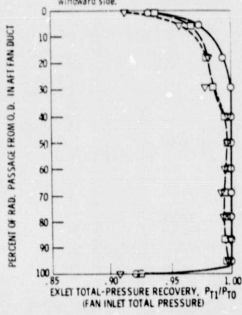
Fig. 11 Exlet and aft fan duct pressure profiles \beta = 148^\circ ; N/\sqrt{B} \sim 85\% ; A_e/A_D = 2.0 ; M_D = 0.30 to 0.35.
