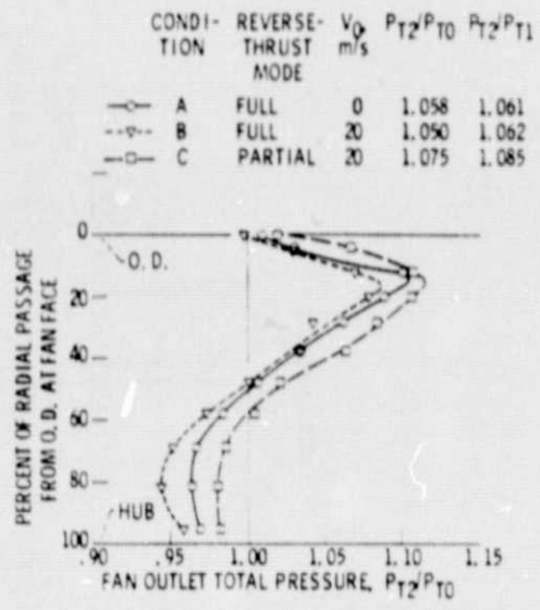
Fig. 12 Fan outlet radial pressure distribution in full and partial reverse-thrust modes. Low-Mach inlet; A_i/A_F = 0.932 ; \beta = 148^\circ ; N/\sqrt{B} \sim 85\% .
