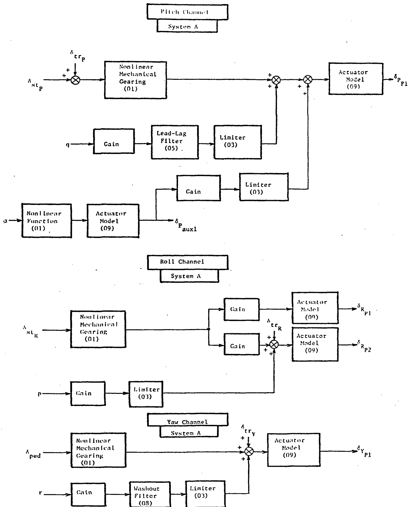
Figure 2-1. Schematics of control system A.
