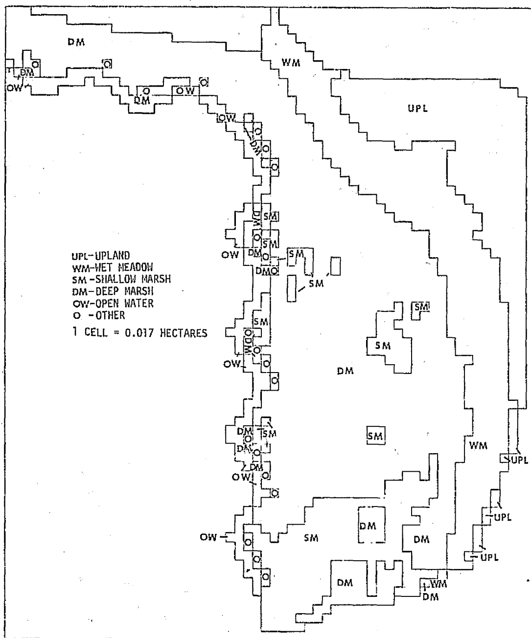
3a. Ground truth
