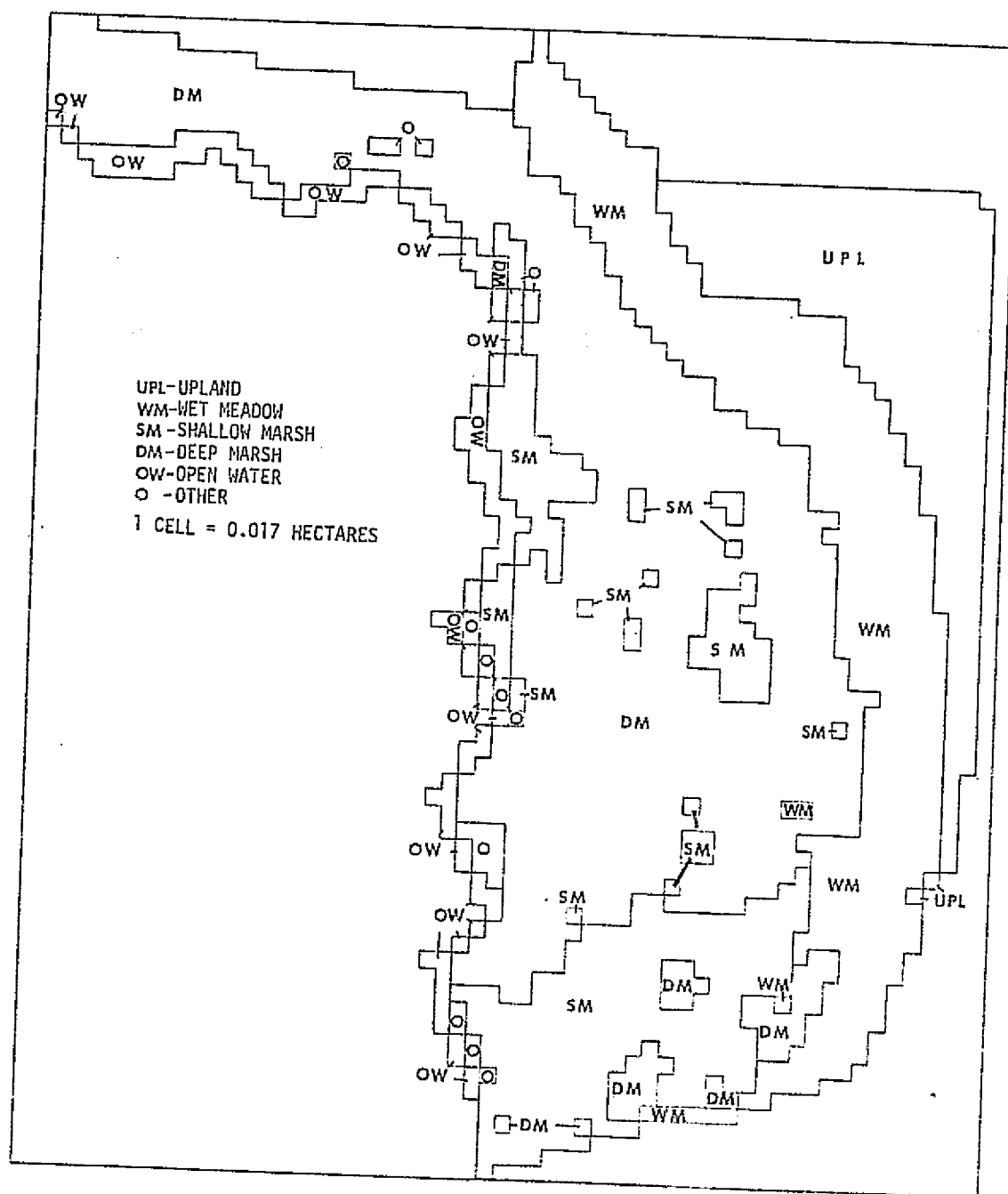
3b. Density sliced interpretation
