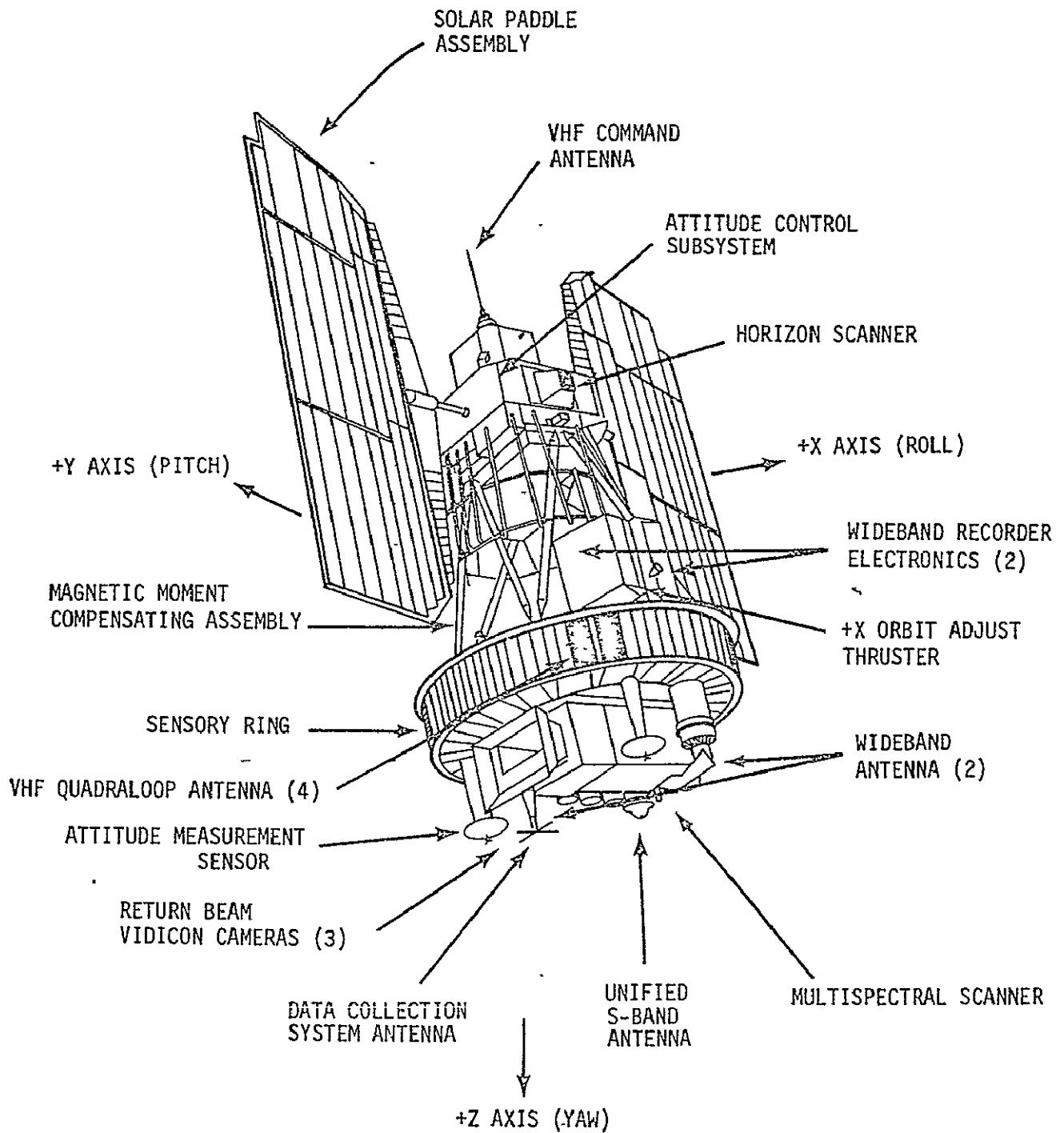
Figure 2 - Landsat spacecraft
