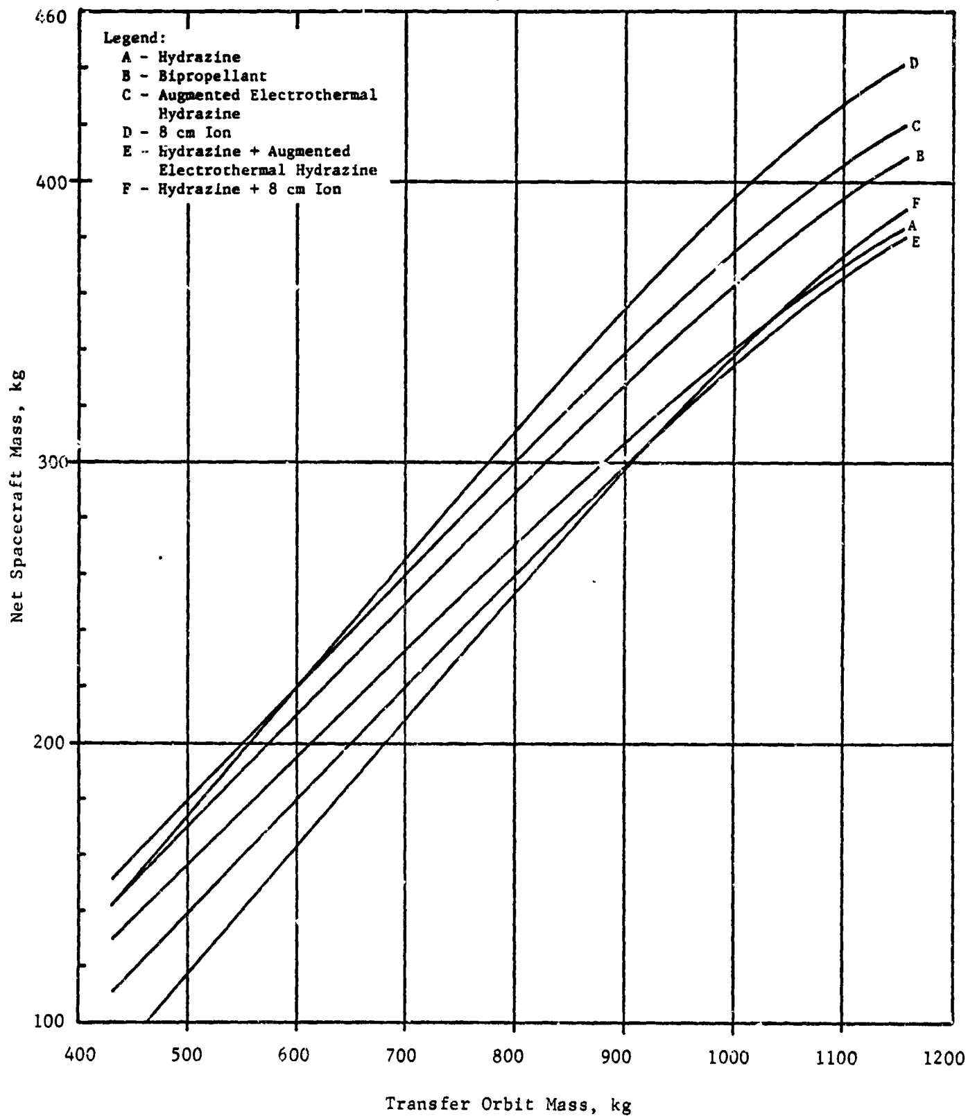
FIGURE 3-19. SPACECRAFT MASS ON SSUS-D
