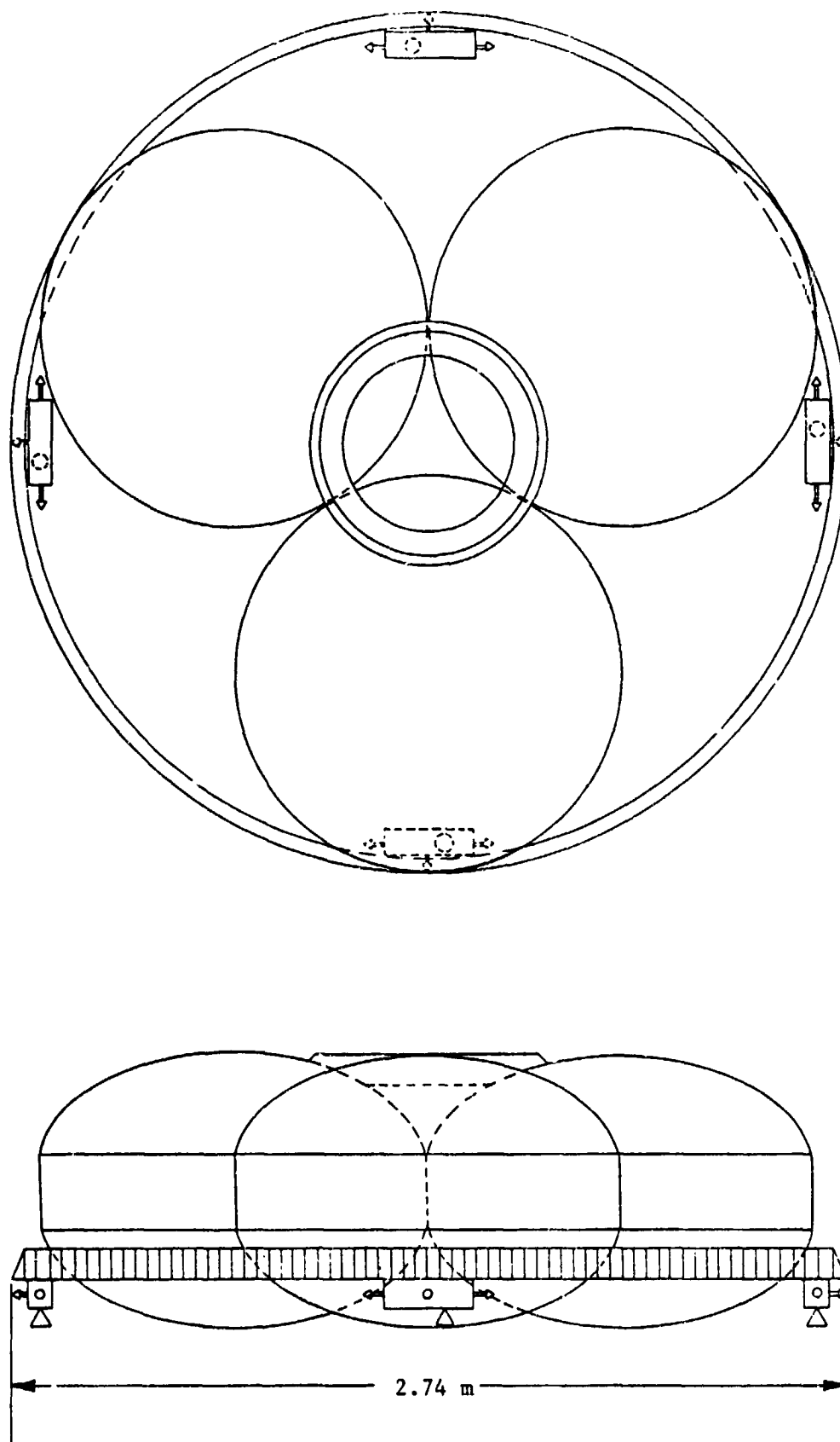
FIGURE 5-3. THREE-TANK HYDRAZINE SYSTEM
