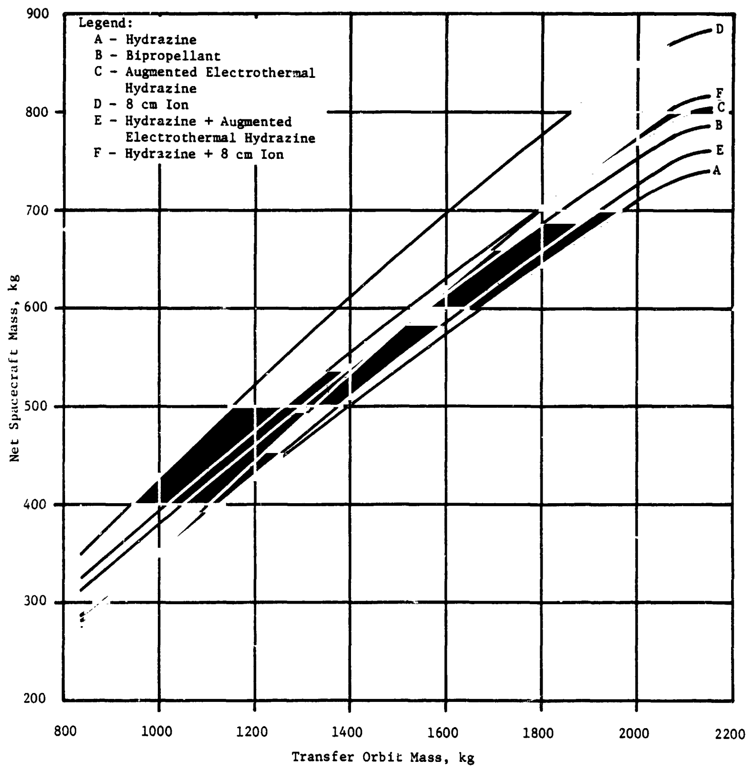
FIGURE 3-20. SPACECRAFT MASS ON SSUS-A
