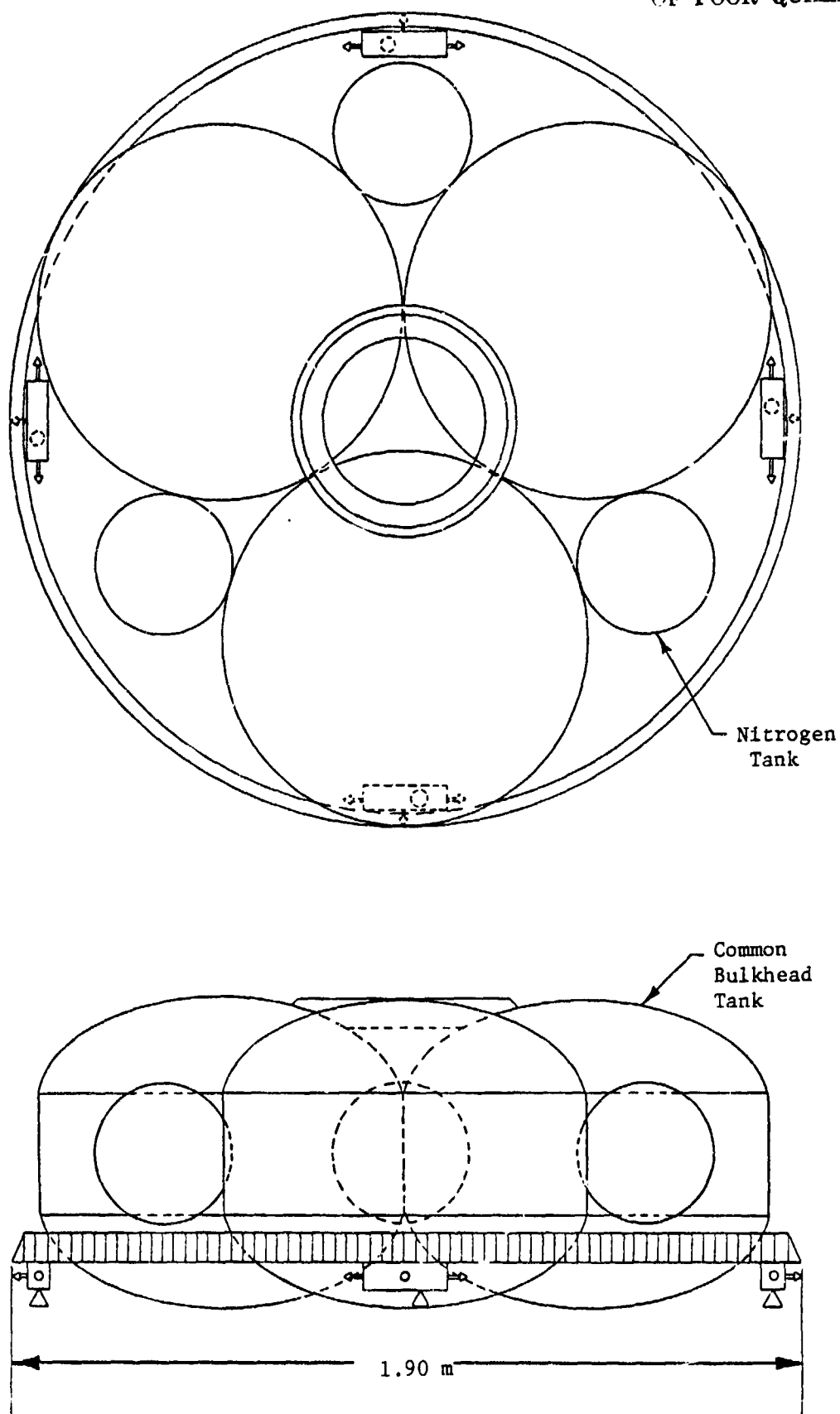
FIGURE 5-6. NEW THREE-TANK BIPOPELLANT MODULE
